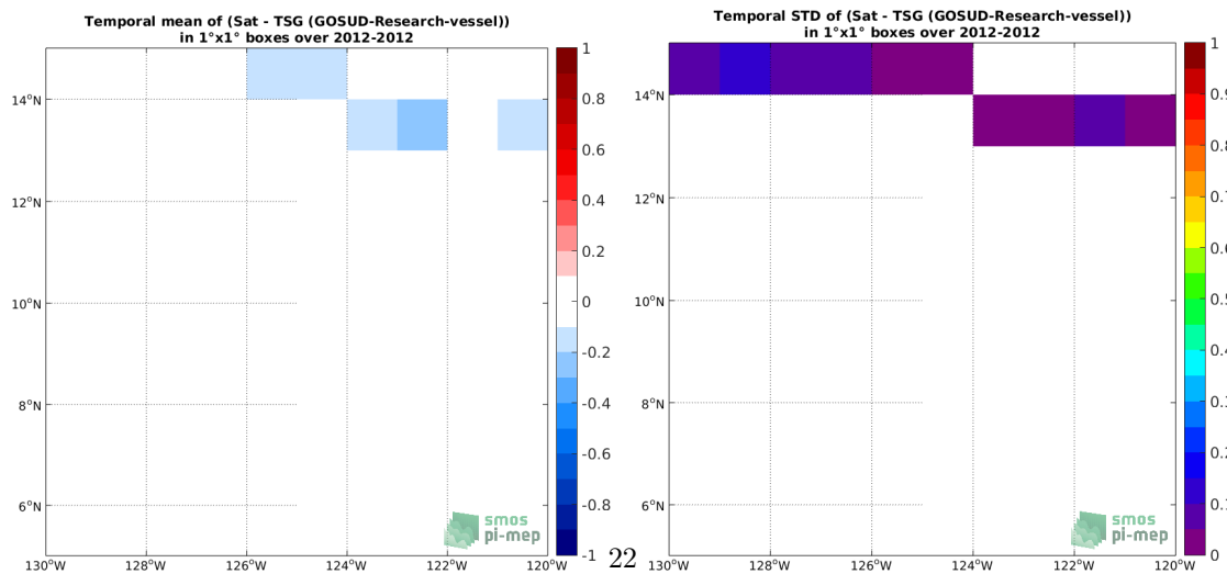
Figure 6: Temporal mean (left) and Std (right) of SSS from Aquarius SSS L3 OR v5 - 7-Day running (NASA-GSFC) (top), TSG (GOSUD-Research-vessel) (middle), and of \Delta SSS (Satellite - TSG (GOSUD-Research-vessel)). Only match-up pairs are used to generate these maps.
