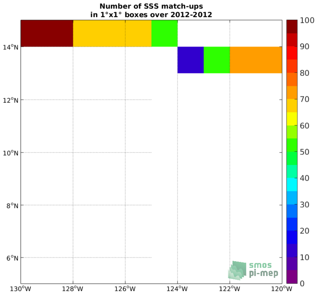
Figure 4: Number of SSS match-ups between TSG (GOSUD-Research-vessel) SSS and the Aquarius SSS L3 OR v5 - 7-Day running (NASA-GSFC) SSS product for the SPURS 2 Pi-MEP region over 1°×1° boxes and for the full satellite product period.
