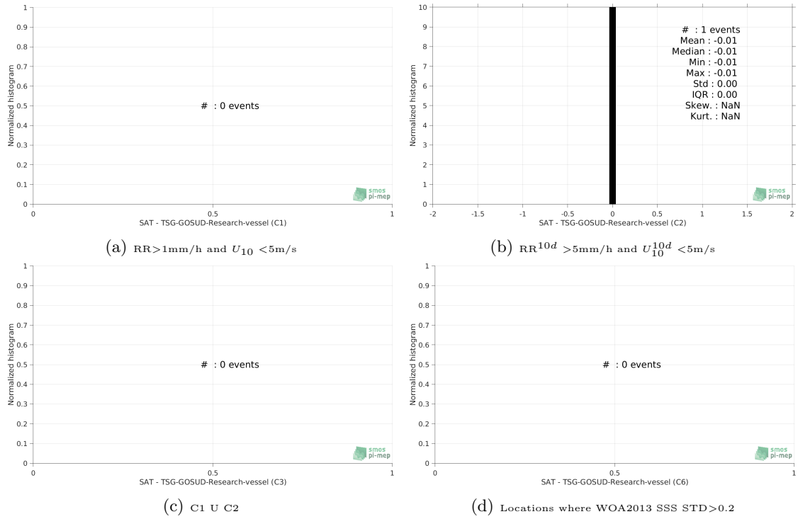
Figure 13: Normalized histogram of \Delta\text{SSS} (Aquarius-L3-OR-V5-7DAY-RUNNING-1DEG - TSG-GOSUD-Research-vessel) for 6 different subdatasets corresponding to: RR > 1\text{mm/h} and U_{10} < 5\text{m/s} (a), RR^{10d} > 5\text{mm/h} and U_{10}^{10d} < 5\text{m/s} (b), C1 U C2 (c), Locations where WOA2013 SSS STD > 0.2 (d).
