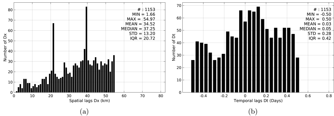
Figure 5: Histograms of the spatial (a) and temporal (b) lags between the time of the TSG-GOSUD-Research-vessel measurements and the date of the corresponding Aquarius-L3-OR-V5-7DAY-RUNNING-1DEG SSS product.
