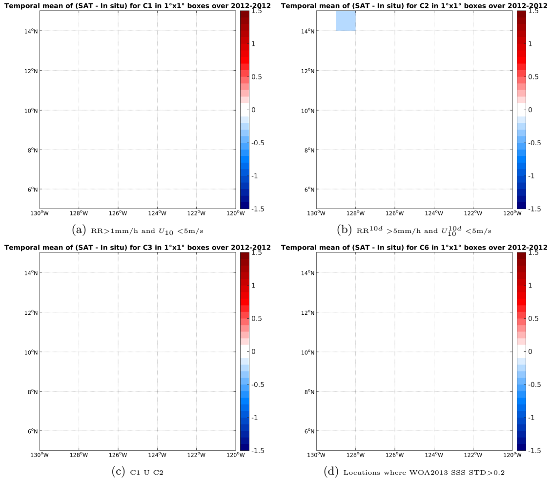
Figure 12: Temporal mean gridded over spatial boxes of size 1°x1° of \Delta SSS (Aquarius-L3-OR-V5-7DAY-RUNNING-1DEG - TSG-GOSUD-Research-vessel) for 4 different subdatasets corresponding to: RR > 1mm/h and U_{10} < 5m/s (a), RR^{10d} > 5mm/h and U_{10}^{10d} < 5m/s (b), C1 U C2 (c), Locations where WOA2013 SSS STD > 0.2 (d).
