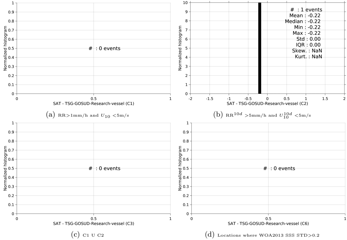
Figure 13: Normalized histogram of \Delta\text{SSS} (Aquarius-L3-OR-V5-7DAY-RUNNING-1DEG - TSG-GOSUD-Research-vessel) for 6 different subdatasets corresponding to: RR > 1\text{mm/h} and U_{10} < 5\text{m/s} (a), RR^{10d} > 5\text{mm/h} and U_{10}^{10d} < 5\text{m/s} (b), C1 U C2 (c), Locations where WOA2013 SSS STD > 0.2 (d).
