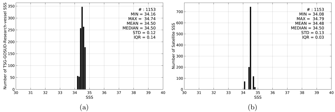
Figure 2: Histograms of SSS from TSG-GOSUD-Research-vessel (a) and Aquarius-L3-OR-V5-7DAY-RUNNING-1DEG (b) considering all match-up pairs per bins of 0.1 over the SPURS 2 Pi-MEP region and for the full satellite product period.
