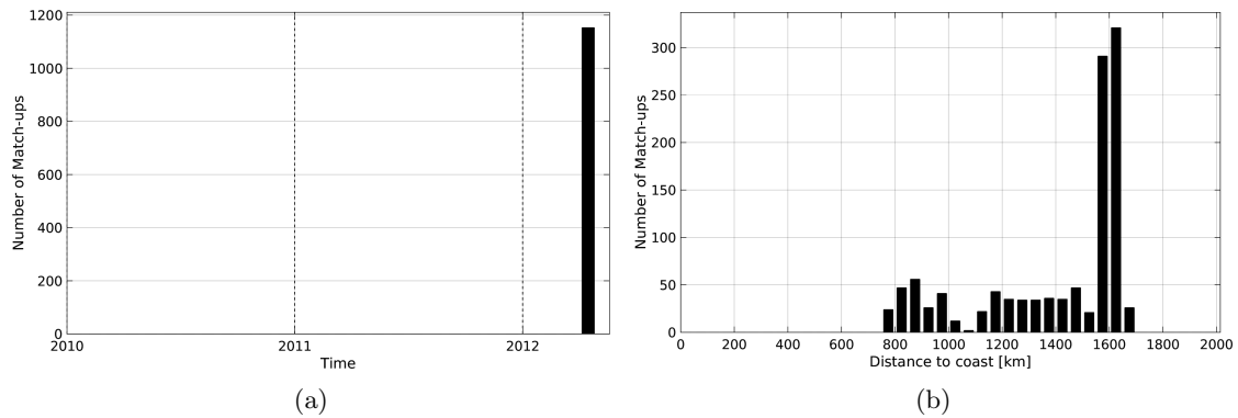
Figure 1: Number of match-ups between TSG-GOSUD-Research-vessel and Aquarius-L3-OR-V5-7DAY-RUNNING-1DEG SSS as a function of time (a) and as function of the distance to coast (b) over the SPURS 2 Pi-MEP region and for the full satellite product period.
