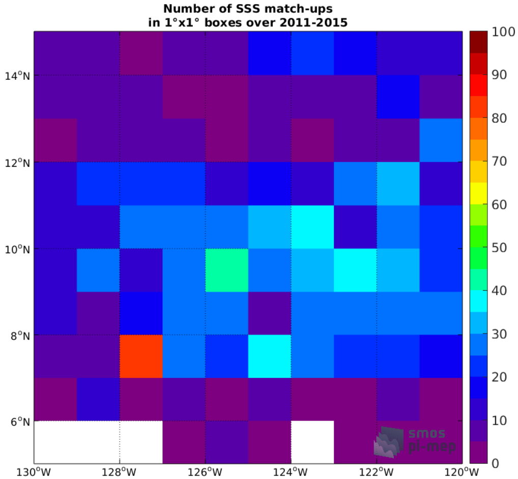
Figure 4: Number of SSS match-ups between Argo SSS and the Aquarius SSS L3 OR v5 - 7-Day running (NASA-GSFC) SSS product for the SPURS 2 Pi-MEP region over 1^\circ \times 1^\circ boxes and for the full satellite product period.
