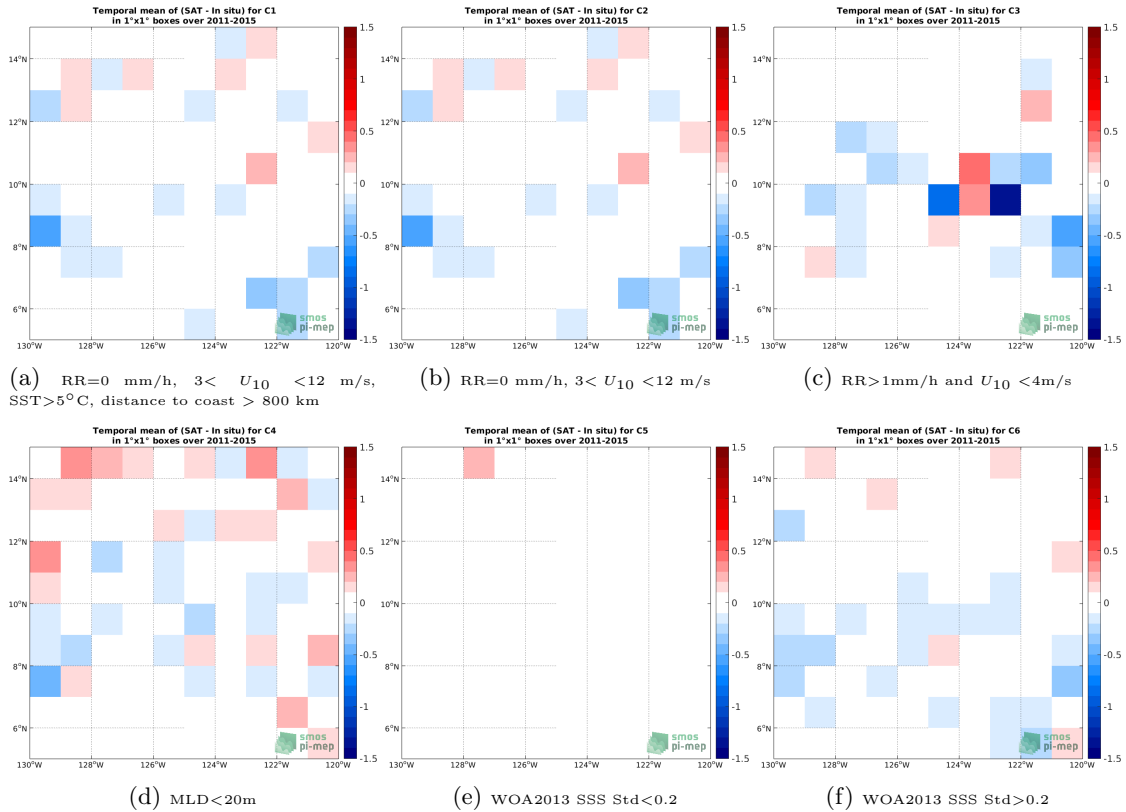
Figure 12: Temporal mean gridded over spatial boxes of size 1^\circ \times 1^\circ of \Delta SSS (Aquarius SSS L3 OR v5 - 7-Day running (NASA-GSFC) - Argo) for 6 different subdatasets corresponding to:RR=0 mm/h, 3 < U_{10} < 12 m/s, SST >5^\circ C, distance to coast > 800 km (a), RR=0 mm/h, 3 < U_{10} < 12 m/s (b), RR >1 mm/h and U_{10} < 4 m/s (c),MLD <20 m (d),WOA2013 SSS Std <0.2 (e),WOA2013 SSS Std >0.2 (f).
