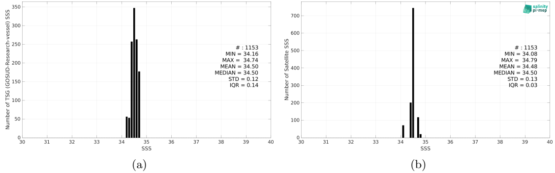
Figure 2: Histograms of SSS from TSG (GOSUD-Research-vessel) (a) and Aquarius SSS L3 OR v5 - 7-Day running - Rain mask (NASA-GSFC) (b) considering all match-up pairs per bins of 0.1 over the SPURS 2 Pi-MEP region and for the full satellite product period.
