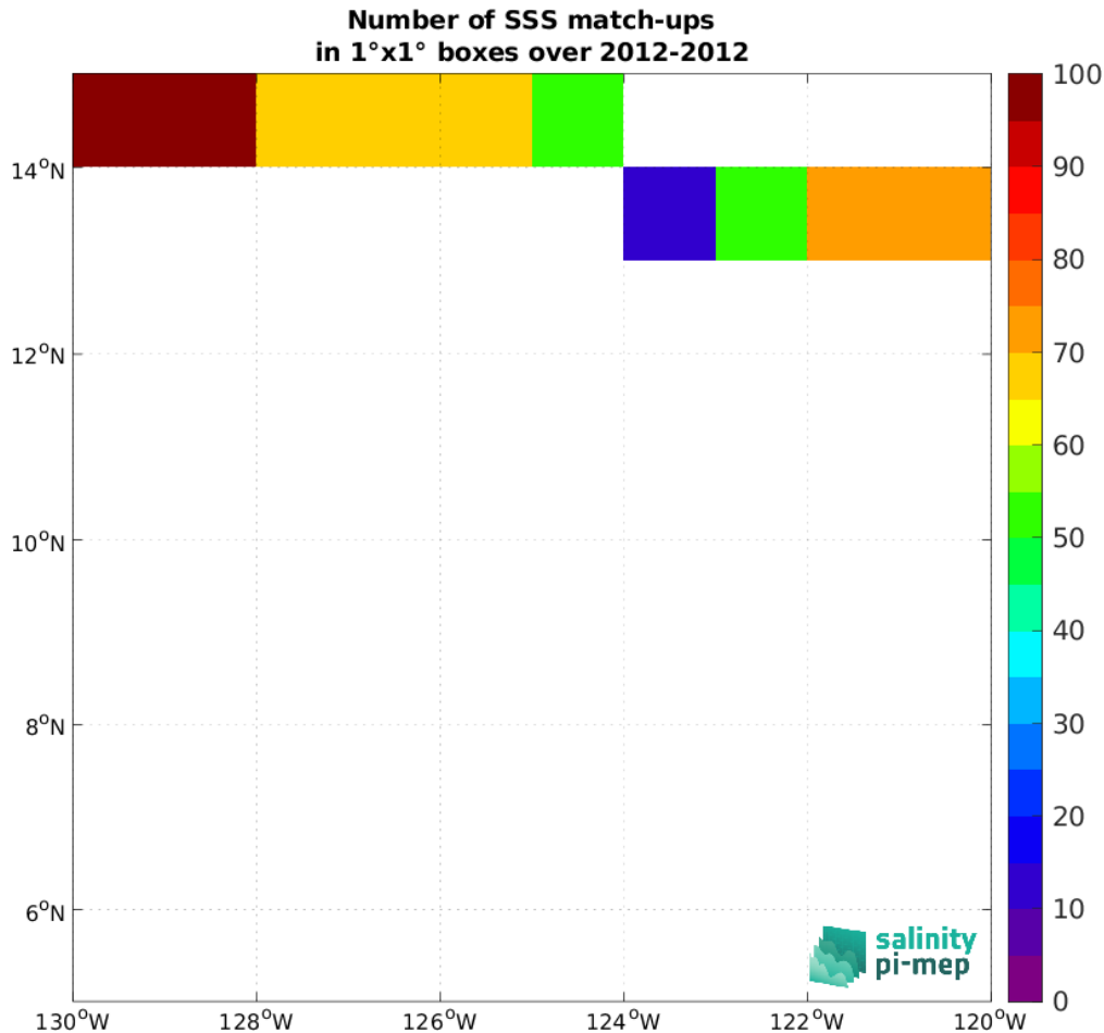
Figure 4: Number of SSS match-ups between TSG (GOSUD-Research-vessel) SSS and the Aquarius SSS L3 OR v5 - 7-Day running - Rain mask (NASA-GSFC) SSS product for the SPURS 2 Pi-MEP region over 1^\circ \times 1^\circ boxes and for the full satellite product period.
