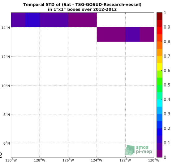
(f) Std( \Delta SSS) (Satellite - TSG-GOSUD-Research-vessel)
