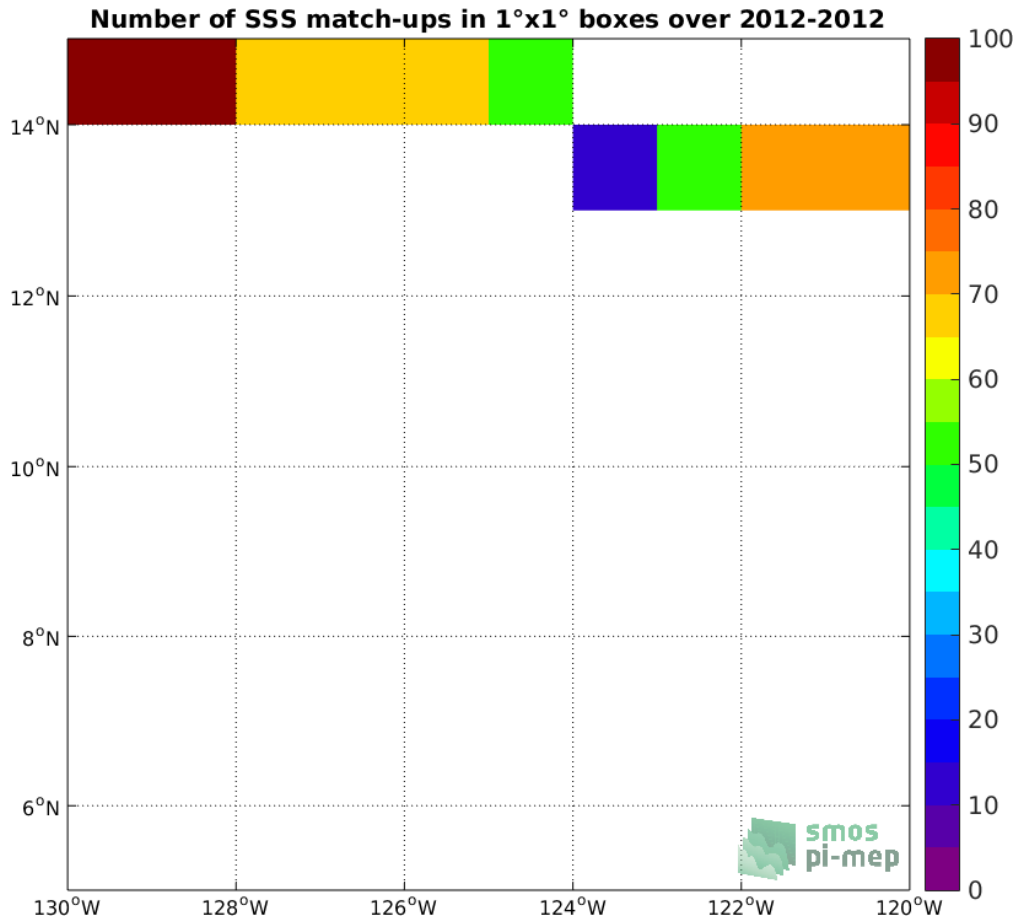
Figure 4: Number of SSS match-ups between TSG-GOSUD-Research-vessel SSS and the Aquarius-L3-OR-V5-7DAY-RUNNING-RAIN-MASK-1DEG SSS product for the SPURS 2 Pi-MEP region over 1°x1° boxes and for the full satellite product period.
