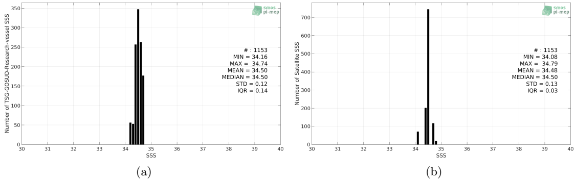
Figure 2: Histograms of SSS from TSG-GOSUD-Research-vessel (a) and Aquarius-L3-OR-V5-7DAY-RUNNING-RAIN-MASK-1DEG (b) considering all match-up pairs per bins of 0.1 over the SPURS 2 Pi-MEP region and for the full satellite product period.
