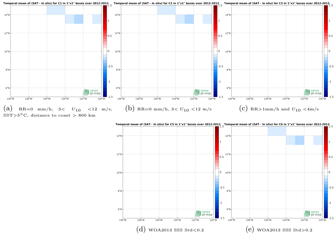
Figure 12: Temporal mean gridded over spatial boxes of size 1^\circ \times 1^\circ of \Delta SSS (Aquarius-L3-OR-V5-7DAY-RUNNING-RAIN-MASK-1DEG - TSG-GOSUD-Research-vessel) for 5 different subdatasets corresponding to:RR=0 mm/h, 3 < U_{10} < 12 m/s, SST >5^\circ C, distance to coast > 800 km (a), RR=0 mm/h, 3 < U_{10} < 12 m/s (b), RR >1 mm/h and U_{10} < 4 m/s (c), WOA2013 SSS Std <0.2 (d), WOA2013 SSS Std >0.2 (e).
