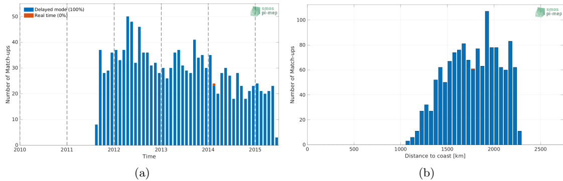
Figure 1: Number of match-ups between Argo and Aquarius SSS L3 OR v5 - 7-Day running - Rain mask (NASA-GSFC) SSS as a function of time (a) and as function of the distance to coast (b) over the SPURS 2 Pi-MEP region and for the full satellite product period.
