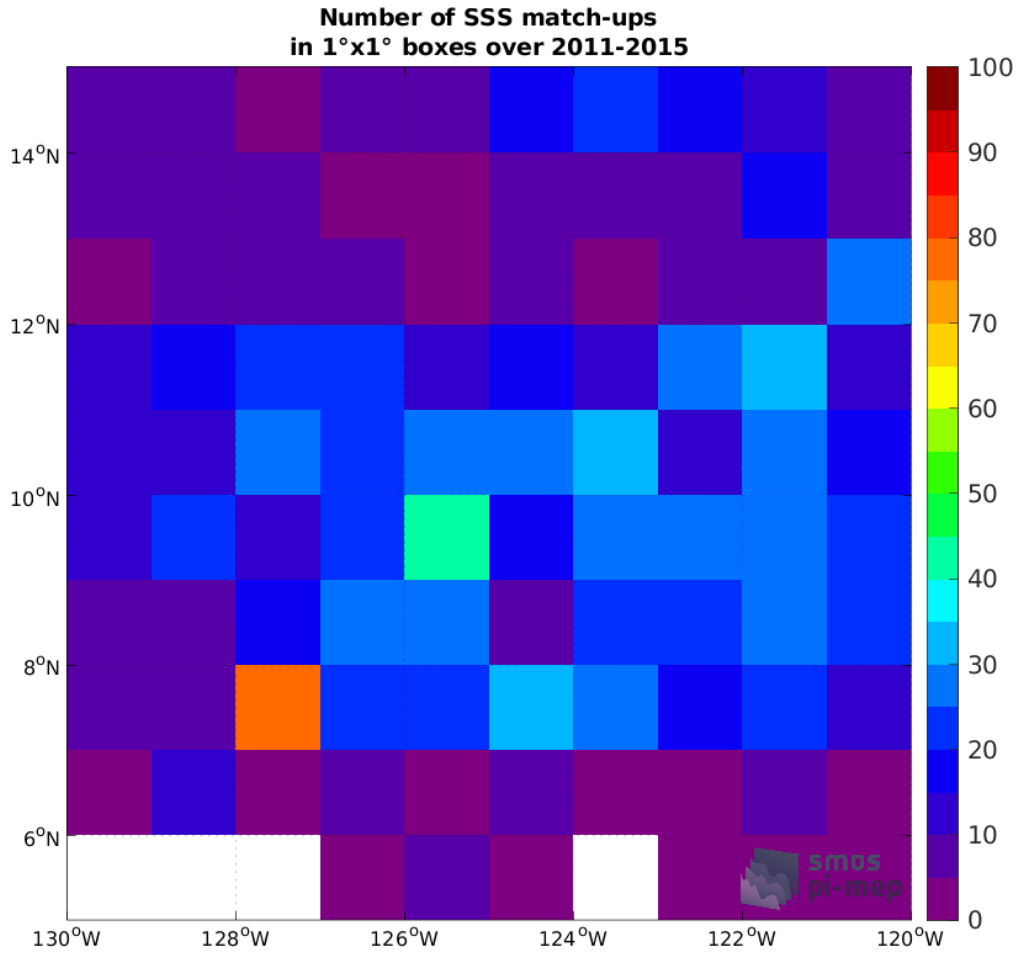
Figure 4: Number of SSS match-ups between Argo SSS and the Aquarius SSS L3 OR v5 - 7-Day running - Rain mask (NASA-GSFC) SSS product for the SPURS 2 Pi-MEP region over 1°x1° boxes and for the full satellite product period.
