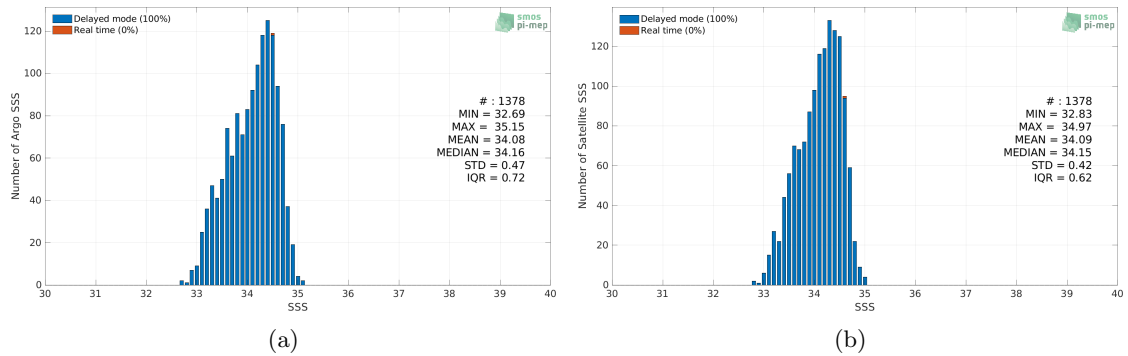
Figure 2: Histograms of SSS from Argo (a) and Aquarius SSS L3 OR v5 - 7-Day running - Rain mask (NASA-GSFC) (b) considering all match-up pairs per bins of 0.1 over the SPURS 2 Pi-MEP region and for the full satellite product period.
