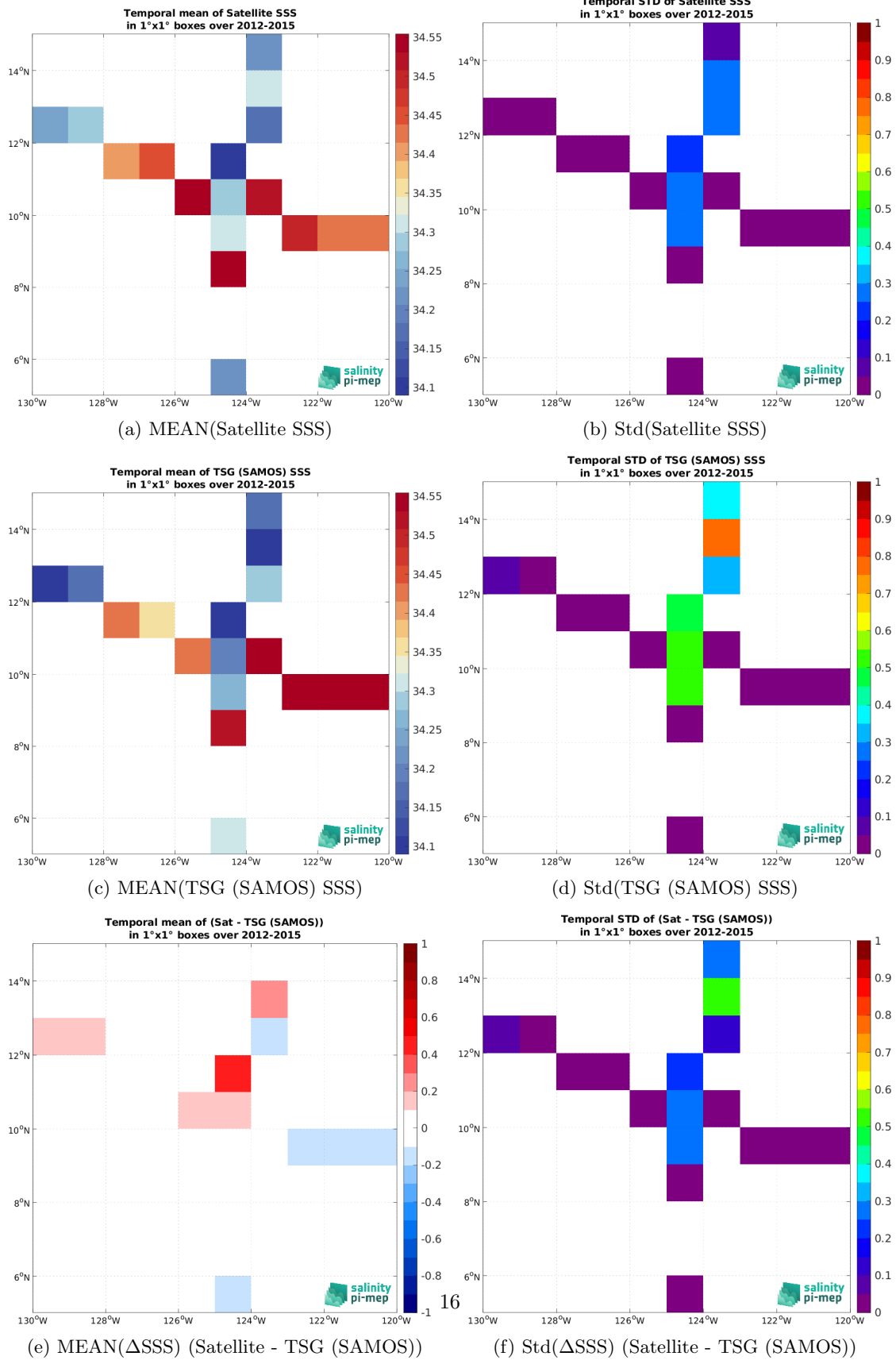
Figure 7: Temporal mean (left) and Std (right) of SSS from Aquarius SSS L3 OR v5 - Monthly (NASA-GSFC) (top), TSG (SAMOS) (middle), and of \Delta SSS (Satellite - TSG (SAMOS)). Only match-up pairs are used to generate these maps.
