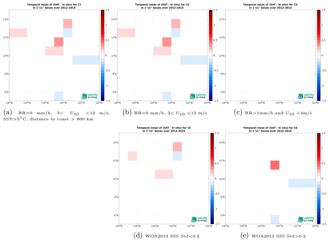
Figure 14: Temporal mean gridded over spatial boxes of size 1^\circ \times 1^\circ of \Delta\text{SSS} (Aquarius SSS L3 OR v5 - Monthly (NASA-GSFC) - TSG (SAMOS)) for 5 different subdatasets corresponding to:RR=0 mm/h, 3 < U_{10} < 12 m/s, SST>5°C, distance to coast > 800 km (a), RR=0 mm/h, 3 < U_{10} < 12 m/s (b), RR>1mm/h and U_{10} < 4 m/s (c), WOA2013 SSS Std<0.2 (d), WOA2013 SSS Std>0.2 (e).
