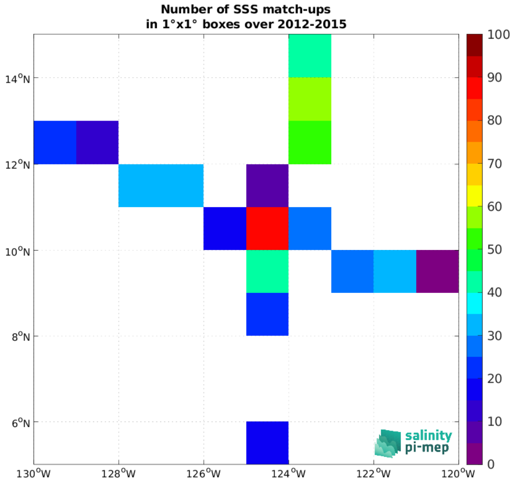
Figure 5: Number of SSS match-ups between TSG (SAMOS) SSS and the Aquarius SSS L3 OR v5 - Monthly (NASA-GSFC) SSS product for the SPURS 2 Pi-MEP region over 1^\circ \times 1^\circ boxes and for the full satellite product period.
