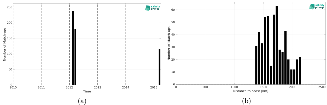
Figure 2: Number of match-ups between TSG (SAMOS) and Aquarius SSS L3 OR v5 - Monthly (NASA-GSFC) SSS as a function of time (a) and as function of the distance to coast (b) over the SPURS 2 Pi-MEP region and for the full satellite product period.
