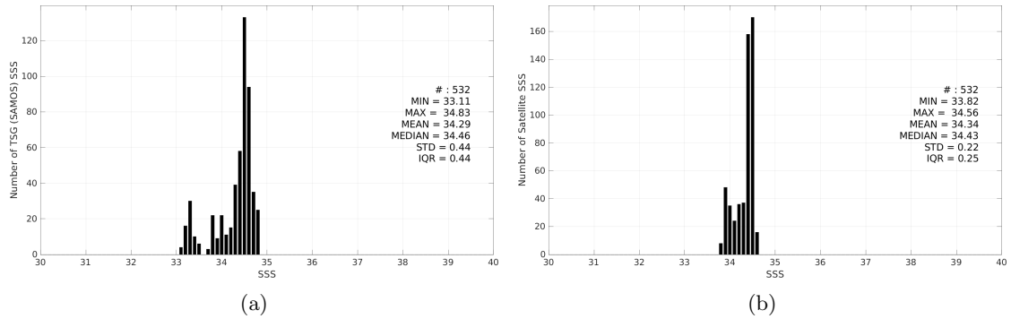
Figure 3: Histograms of SSS from TSG (SAMOS) (a) and Aquarius SSS L3 OR v5 - Monthly (NASA-GSFC) (b) considering all match-up pairs per bins of 0.1 over the SPURS 2 Pi-MEP region and for the full satellite product period.
