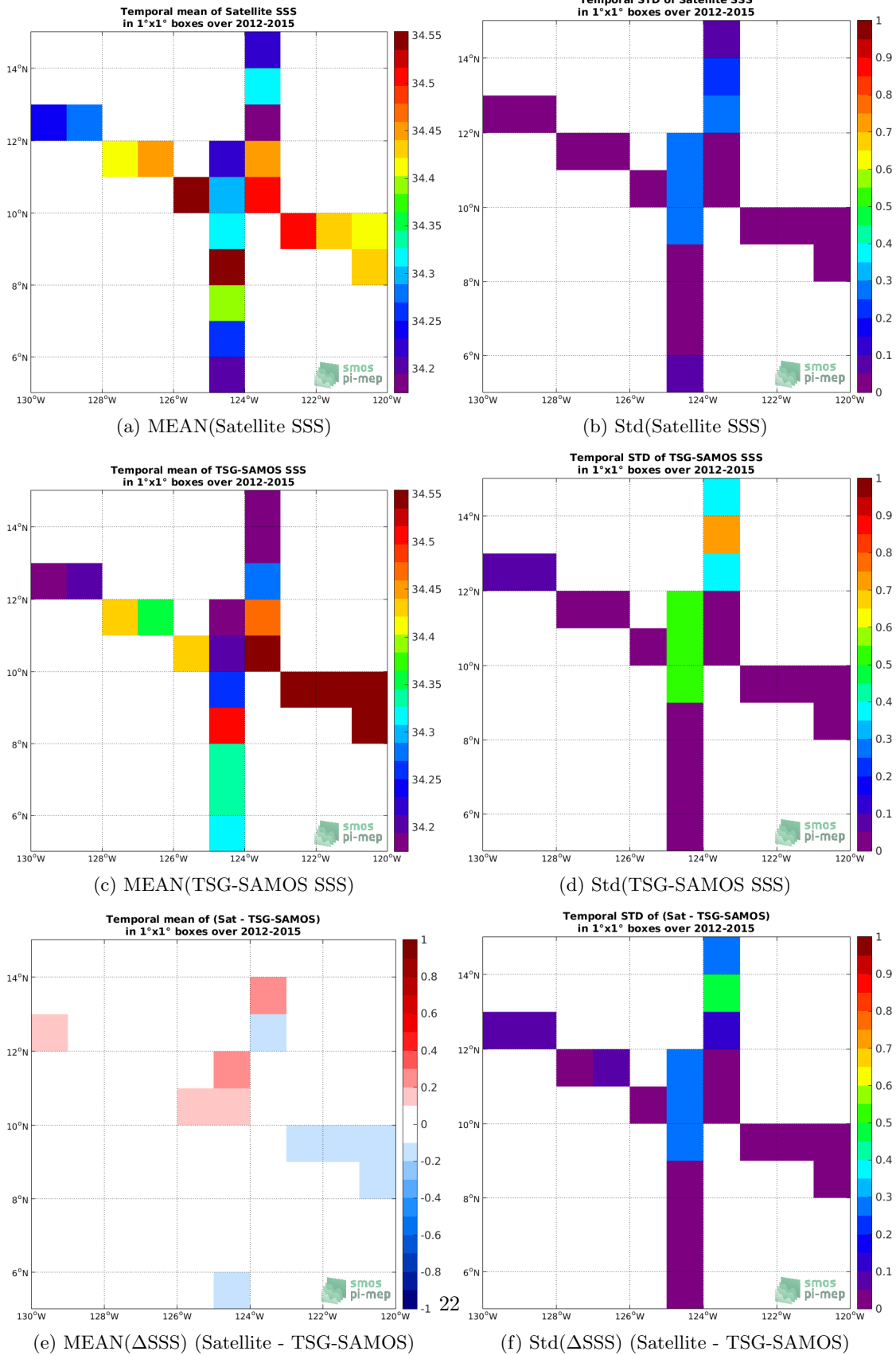
Figure 6: Temporal mean (left) and Std (right) of SSS from Aquarius-L3-OR-V5-MONTHLY-1DEG (top), TSG-SAMOS (middle), and of \Delta SSS (Satellite - TSG-SAMOS). Only match-up pairs are used to generate these maps.
