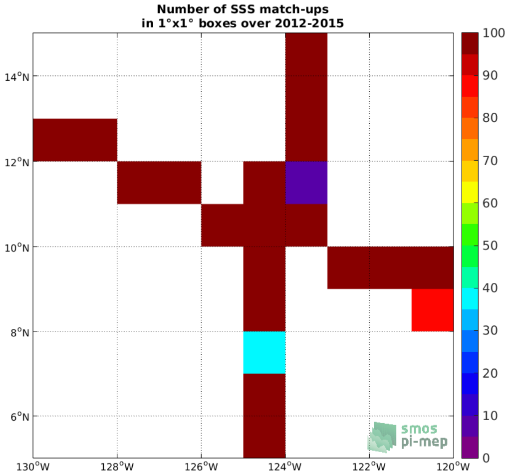
Figure 4: Number of SSS match-ups between TSG-SAMOS SSS and the Aquarius-L3-OR-V5-MONTHLY-1DEG SSS product for the SPURS 2 Pi-MEP region over 1°x1° boxes and for the full satellite product period.
