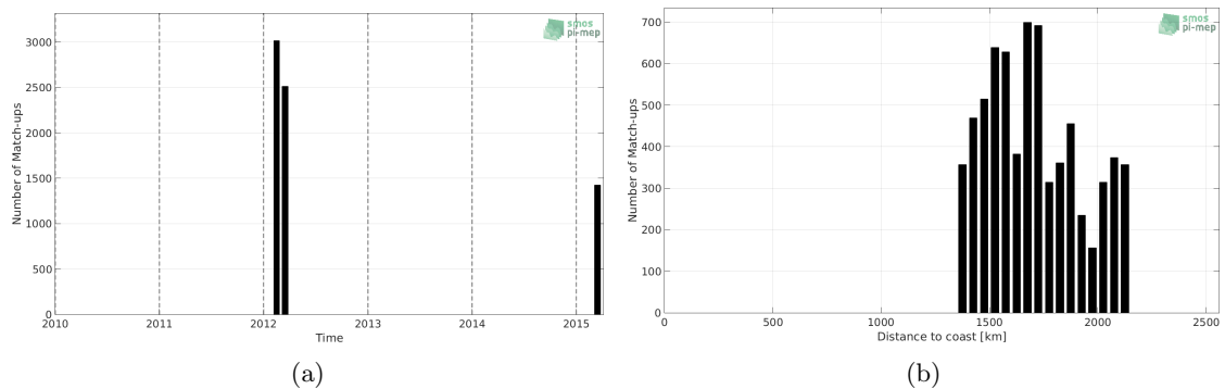
Figure 1: Number of match-ups between TSG-SAMOS and Aquarius-L3-OR-V5-MONTHLY-1DEG SSS as a function of time (a) and as function of the distance to coast (b) over the SPURS 2 Pi-MEP region and for the full satellite product period.
