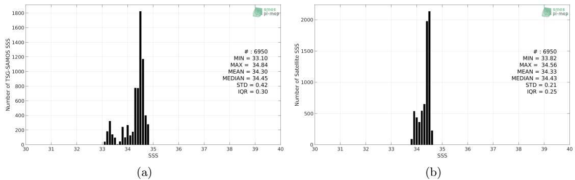
Figure 2: Histograms of SSS from TSG-SAMOS (a) and Aquarius-L3-OR-V5-MONTHLY-1DEG (b) considering all match-up pairs per bins of 0.1 over the SPURS 2 Pi-MEP region and for the full satellite product period.
