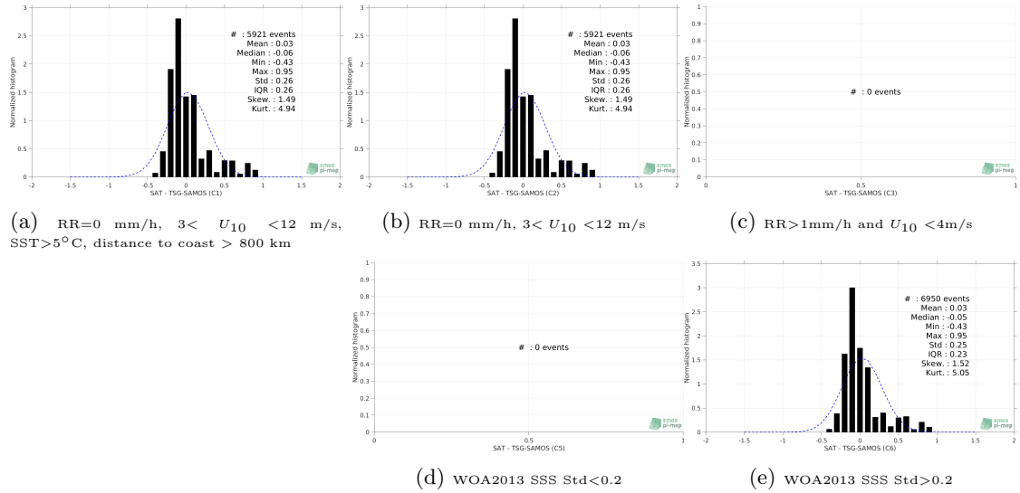
Figure 13: Normalized histogram of \Delta\text{SSS} (Aquarius-L3-OR-V5-MONTHLY-1DEG - TSG-SAMOS) for 5 different subdatasets corresponding to: RR=0 mm/h, 3 < U_{10} < 12 m/s, SST >5^{\circ}\text{C} , distance to coast > 800 km (a), RR=0 mm/h, 3 < U_{10} < 12 m/s (b), RR >1 mm/h and U_{10} < 4 m/s (c), WOA2013 SSS Std <0.2 (d), WOA2013 SSS Std >0.2 (e).
