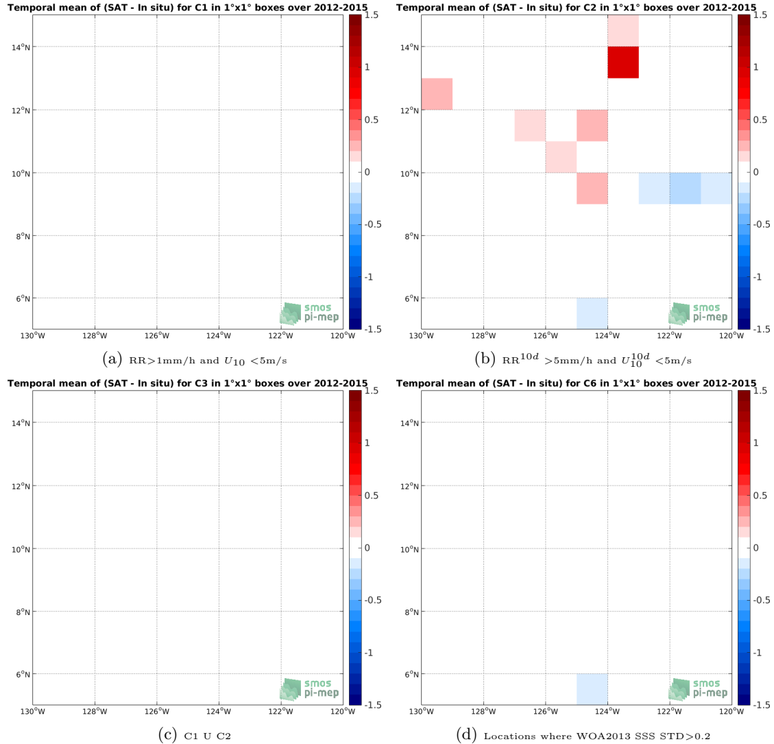
Figure 12: Temporal mean gridded over spatial boxes of size 1^\circ \times 1^\circ of \Delta SSS (Aquarius-L3-OR-V5-MONTHLY - TSG-SAMOS) for 4 different subdatasets corresponding to: RR > 1\text{mm/h} and U_{10} < 5\text{m/s} (a), RR^{10d} > 5\text{mm/h} and U_{10}^{10d} < 5\text{m/s} (b), C1 U C2 (c), Locations where WOA2013 SSS STD > 0.2 (d).
