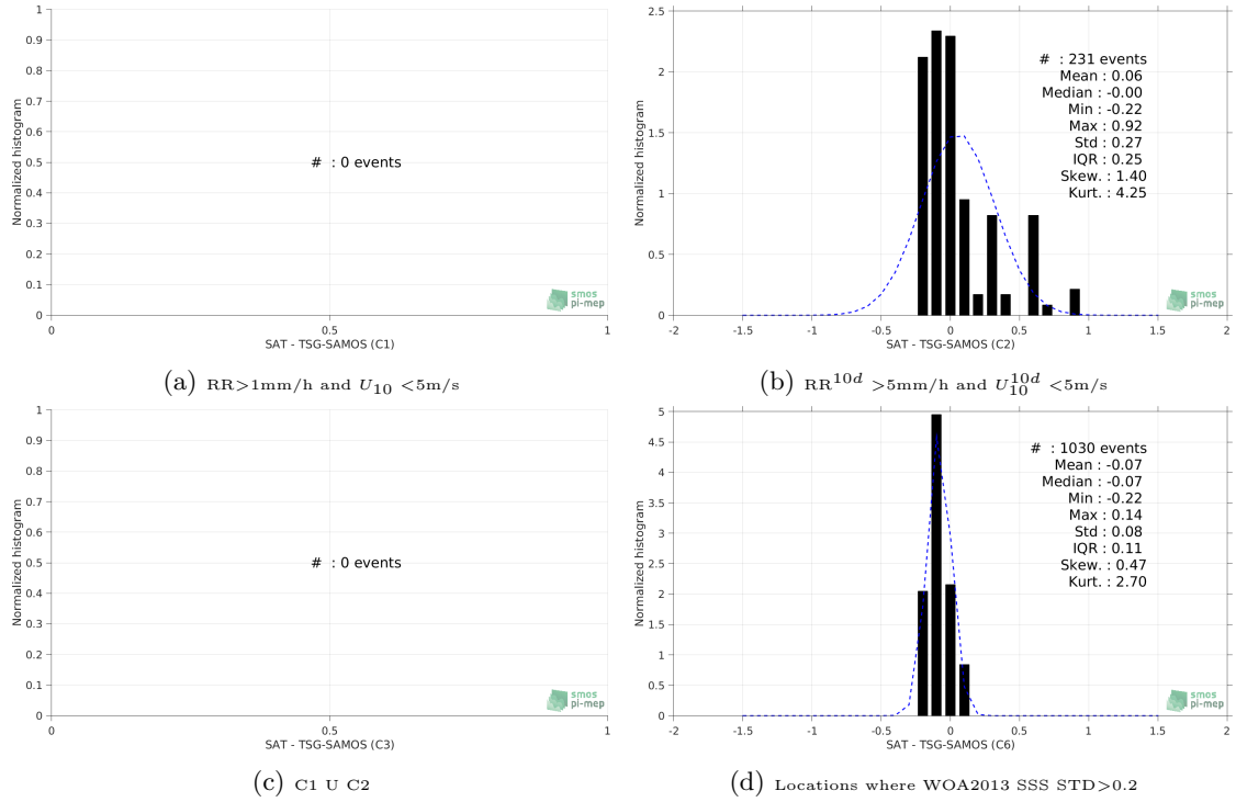
Figure 13: Normalized histogram of \Delta\text{SSS} (Aquarius-L3-OR-V5-MONTHLY - TSG-SAMOS) for 6 different subdatasets corresponding to: RR > 1\text{mm/h} and U_{10} < 5\text{m/s} (a), RR^{10d} > 5\text{mm/h} and U_{10}^{10d} < 5\text{m/s} (b), C1 \cup C2 (c), Locations where WOA2013 SSS STD > 0.2 (d).
