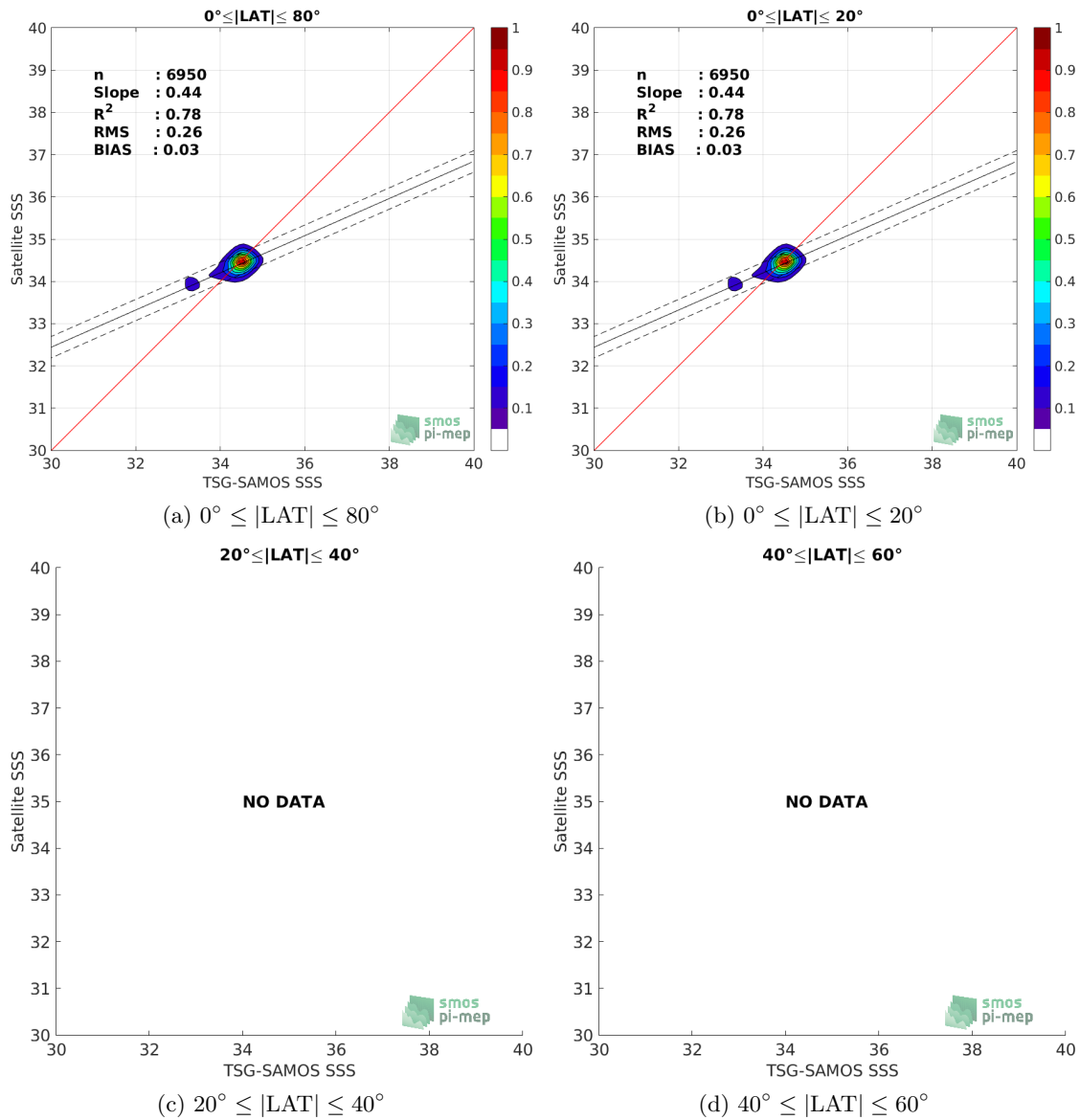
Figure 9: Contour maps of the concentration of Aquarius-L3-OR-V5-MONTHLY SSS (y-axis) versus TSG-SAMOS SSS (x-axis) at match-up pairs for different latitude bands. For each plot, the red line shows x=y . The black thin and dashed lines indicate a linear fit through the data cloud and the \pm 95\% confidence levels, respectively. The number match-up pairs n , the slope and R^2 coefficient of the linear fit, the root mean square (RMS) and the mean bias between satellite and in situ data are indicated for each latitude band in each plots.
