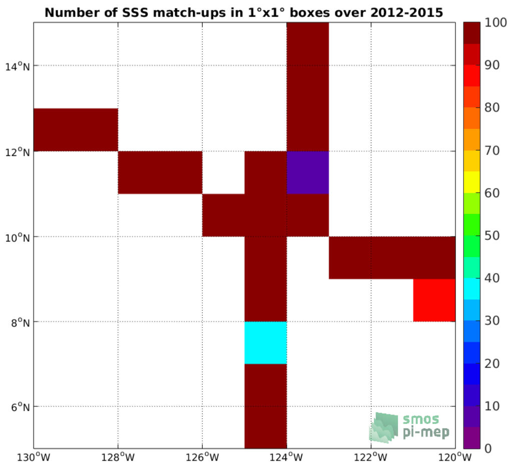
Figure 4: Number of SSS match-ups between TSG-SAMOS SSS and the Aquarius-L3-OR-V5-MONTHLY SSS product for the SPURS 2 Pi-MEP region over 1°x1° boxes and for the full satellite product period.
