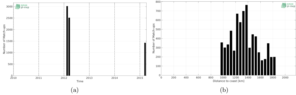
Figure 1: Number of match-ups between TSG-SAMOS and Aquarius-L3-OR-V5-MONTHLY SSS as a function of time (a) and as function of the distance to coast (b) over the SPURS 2 Pi-MEP region and for the full satellite product period.
