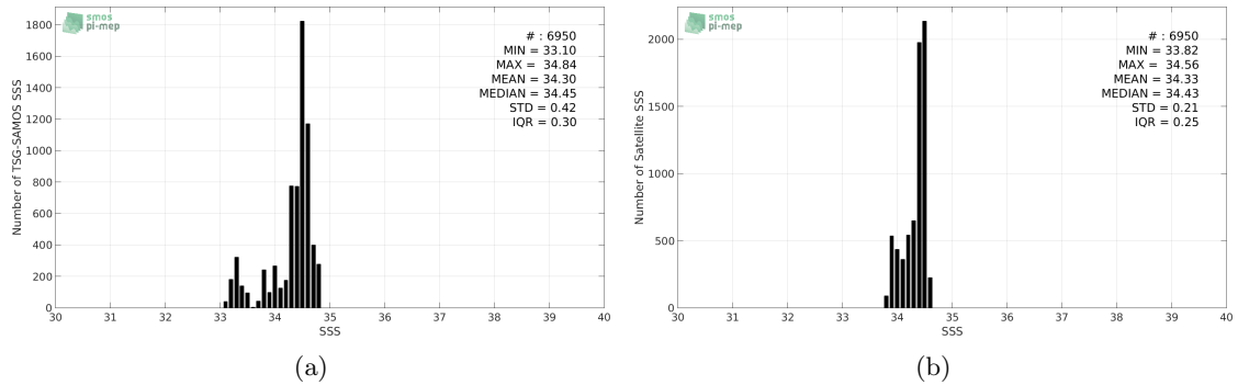
Figure 2: Histograms of SSS from TSG-SAMOS (a) and Aquarius-L3-OR-V5-MONTHLY (b) considering all match-up pairs per bins of 0.1 over the SPURS 2 Pi-MEP region and for the full satellite product period.
