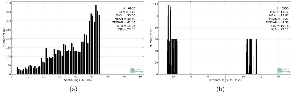
Figure 5: Histograms of the spatial (a) and temporal (b) lags between the time of the TSG-SAMOS measurements and the date of the corresponding Aquarius-L3-OR-V5-MONTHLY SSS product.
