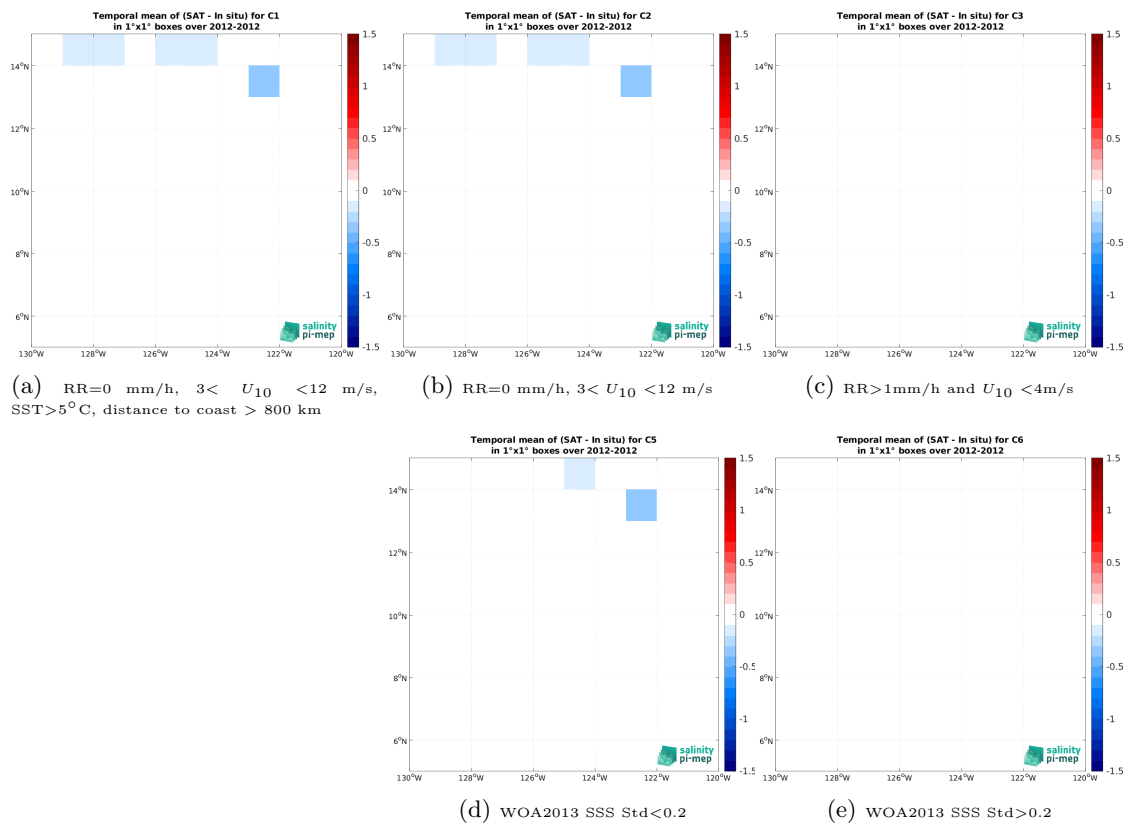
Figure 14: Temporal mean gridded over spatial boxes of size 1^\circ \times 1^\circ of \Delta\text{SSS} (Aquarius SSS L3 OR v5 - Monthly (NASA-GSFC) - TSG (GOSUD-Research-vessel)) for 5 different subdatasets corresponding to: RR=0 mm/h, 3 < U_{10} < 12 m/s, SST > 5°C, distance to coast > 800 km (a), RR=0 mm/h, 3 < U_{10} < 12 m/s (b), RR > 1mm/h and U_{10} < 4 m/s (c), WOA2013 SSS Std < 0.2 (d), WOA2013 SSS Std > 0.2 (e).
