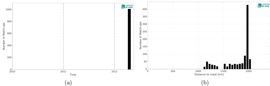
Figure 2: Number of match-ups between TSG (GOSUD-Research-vessel) and Aquarius SSS L3 OR v5 - Monthly (NASA-GSFC) SSS as a function of time (a) and as function of the distance to coast (b) over the SPURS 2 Pi-MEP region and for the full satellite product period.
