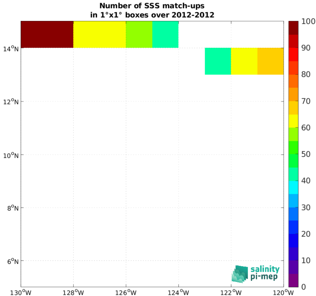
Figure 5: Number of SSS match-ups between TSG (GOSUD-Research-vessel) SSS and the Aquarius SSS L3 OR v5 - Monthly (NASA-GSFC) SSS product for the SPURS 2 Pi-MEP region over 1^\circ \times 1^\circ boxes and for the full satellite product period.
