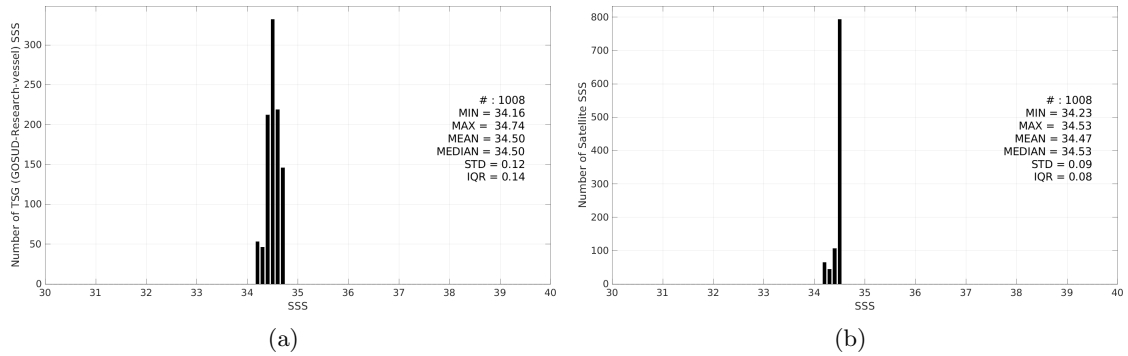
Figure 3: Histograms of SSS from TSG (GOSUD-Research-vessel) (a) and Aquarius SSS L3 OR v5 - Monthly (NASA-GSFC) (b) considering all match-up pairs per bins of 0.1 over the SPURS 2 Pi-MEP region and for the full satellite product period.
