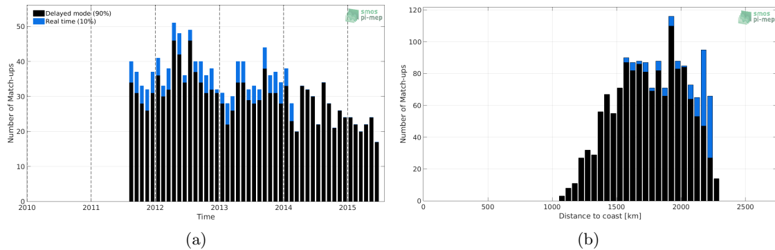
Figure 1: Number of match-ups between Argo and Aquarius-L3-OR-V5-MONTHLY-1DEG SSS as a function of time (a) and as function of the distance to coast (b) over the SPURS 2 Pi-MEP region and for the full satellite product period.
