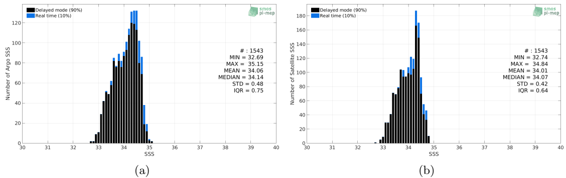
Figure 2: Histograms of SSS from Argo (a) and Aquarius-L3-OR-V5-MONTHLY-1DEG (b) considering all match-up pairs per bins of 0.1 over the SPURS 2 Pi-MEP region and for the full satellite product period.
