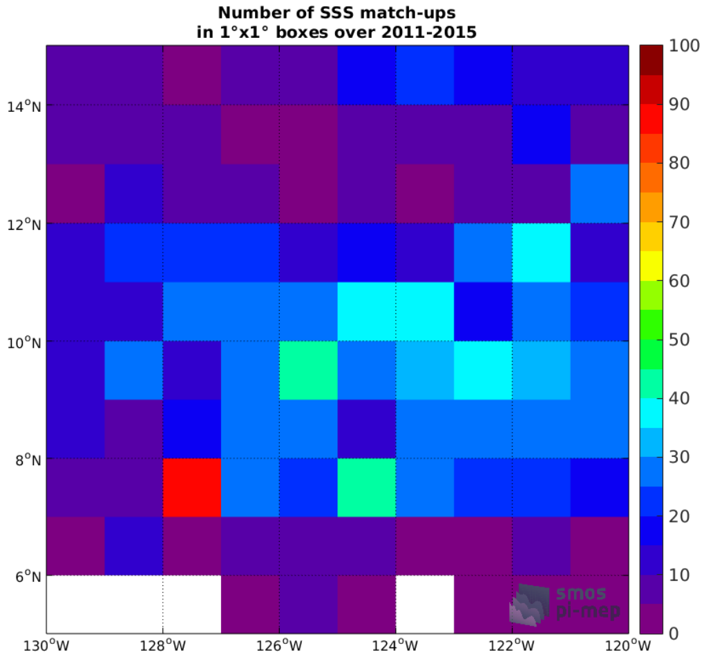
Figure 4: Number of SSS match-ups between Argo SSS and the Aquarius-L3-OR-V5-MONTHLY-1DEG SSS product for the SPURS 2 Pi-MEP region over 1°x1° boxes and for the full satellite product period.
