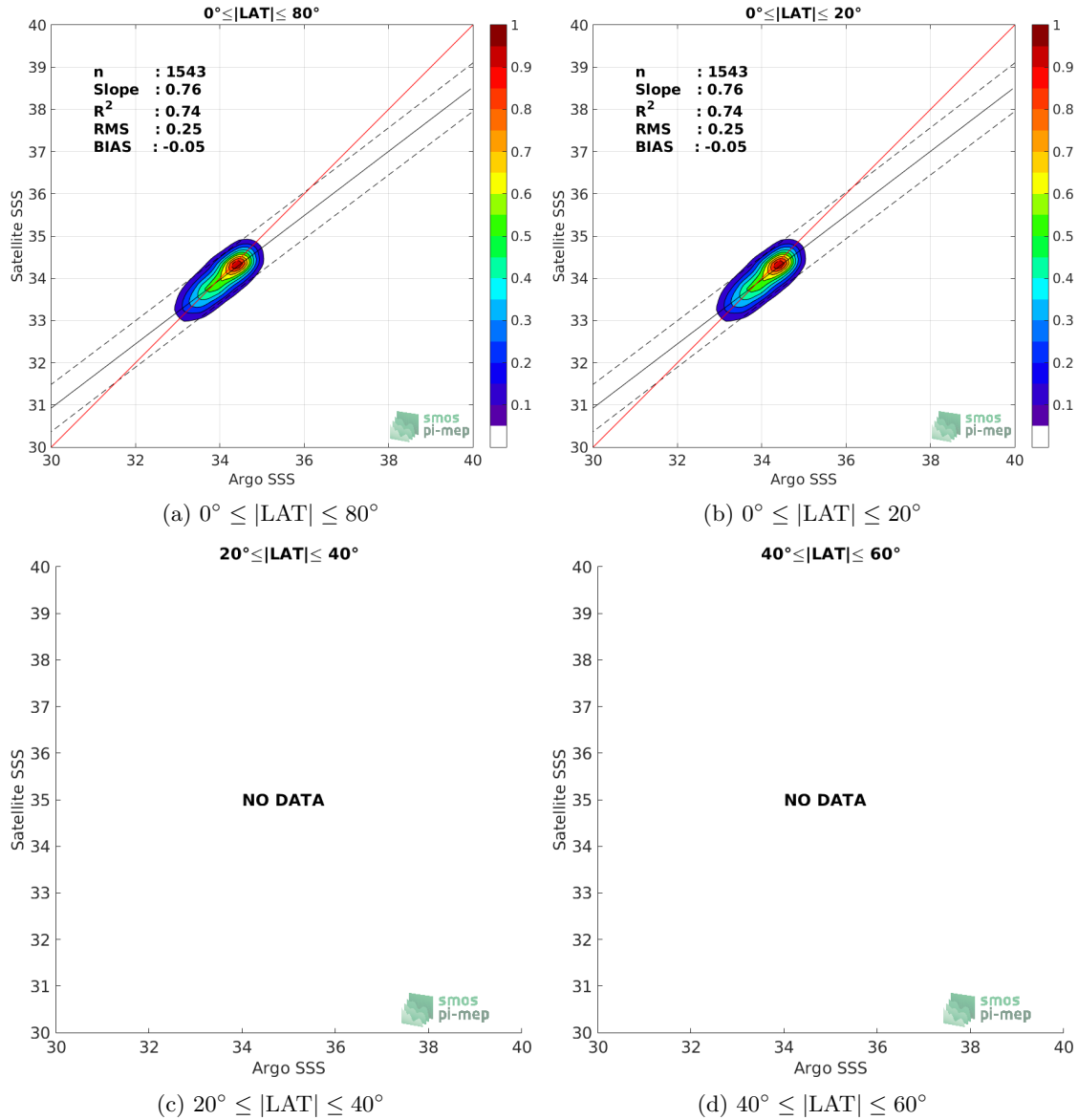
Figure 9: Contour maps of the concentration of Aquarius-L3-OR-V5-MONTHLY SSS (y-axis) versus Argo SSS (x-axis) at match-up pairs for different latitude bands. For each plot, the red line shows x=y . The black thin and dashed lines indicate a linear fit through the data cloud and the \pm 95\% confidence levels, respectively. The number match-up pairs n , the slope and R^2 coefficient of the linear fit, the root mean square (RMS) and the mean bias between satellite and in situ data are indicated for each latitude band in each plots.
