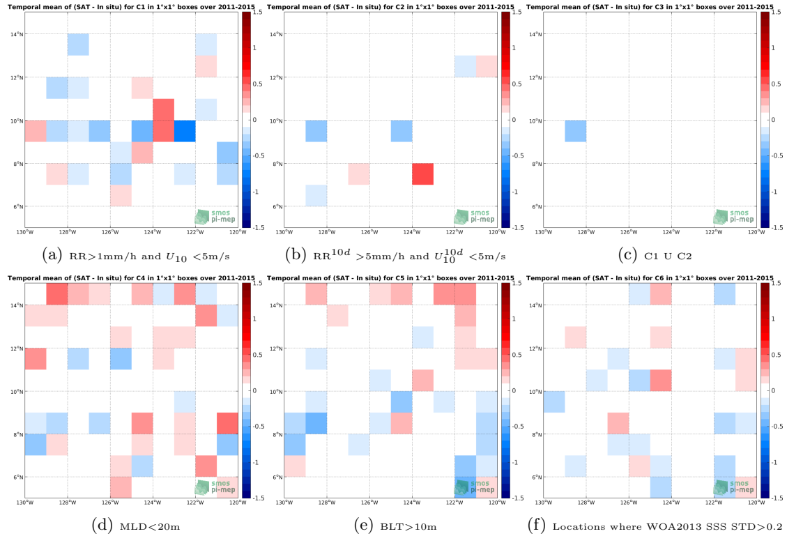
Figure 12: Temporal mean gridded over spatial boxes of size 1^\circ \times 1^\circ of \Delta\text{SSS} (Aquarius-L3-OR-V5-MONTHLY - Argo) for 6 different subdatasets corresponding to: \text{RR} > 1\text{mm/h} and U_{10} < 5\text{m/s} (a), \text{RR}^{10d} > 5\text{mm/h} and U_{10}^{10d} < 5\text{m/s} (b), C1 U C2 (c), \text{MLD} < 20\text{m} (d), \text{BLT} > 10\text{m} (e), Locations where WOA2013 SSS STD > 0.2 (f).
