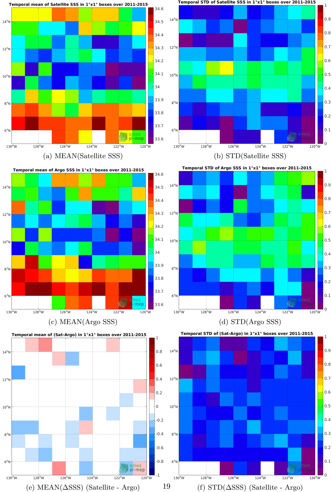
Figure 6: Temporal mean (left) and STD (right) of SSS from Aquarius-L3-OR-V5-MONTHLY (top), Argo (middle), and of \Delta SSS (Satellite - Argo). Only match-up pairs are used to generate these maps.
