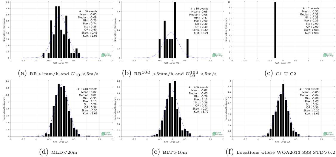
Figure 13: Normalized histogram of \Delta SSS (Aquarius-L3-OR-V5-MONTHLY - Argo) for 6 different subdatasets corresponding to: RR > 1\text{mm/h} and U_{10} < 5\text{m/s} (a), RR^{10d} > 5\text{mm/h} and U_{10}^{10d} < 5\text{m/s} (b), C1 \cup C2 (c), MLD < 20\text{m} (d), BLT > 10\text{m} (e), Locations where WOA2013 SSS STD > 0.2 (f).
