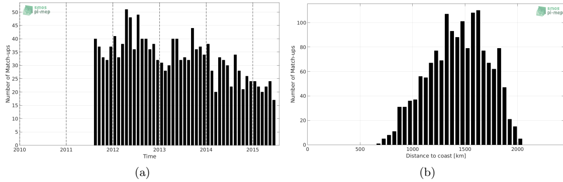
Figure 1: Number of match-ups between Argo and Aquarius-L3-OR-V5-MONTHLY SSS as a function of time (a) and as function of the distance to coast (b) over the SPURS 2 Pi-MEP region and for the full satellite product period.
