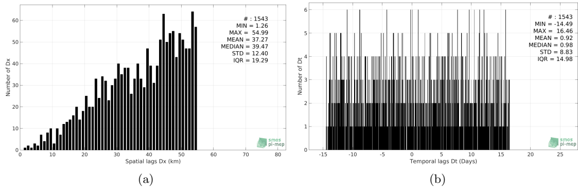
Figure 5: Histograms of the spatial (a) and temporal (b) lags between the time of the Argo measurements and the date of the corresponding Aquarius-L3-OR-V5-MONTHLY SSS product.
