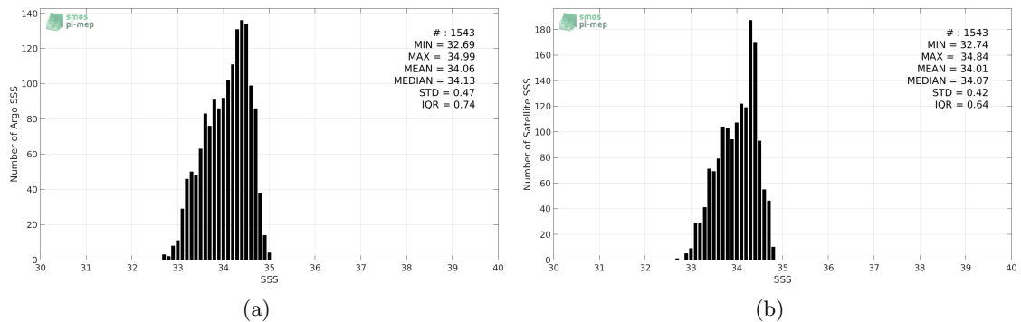
Figure 2: Histograms of SSS from Argo (a) and Aquarius-L3-OR-V5-MONTHLY (b) considering all match-up pairs per bins of 0.1 over the SPURS 2 Pi-MEP region and for the full satellite product period.
