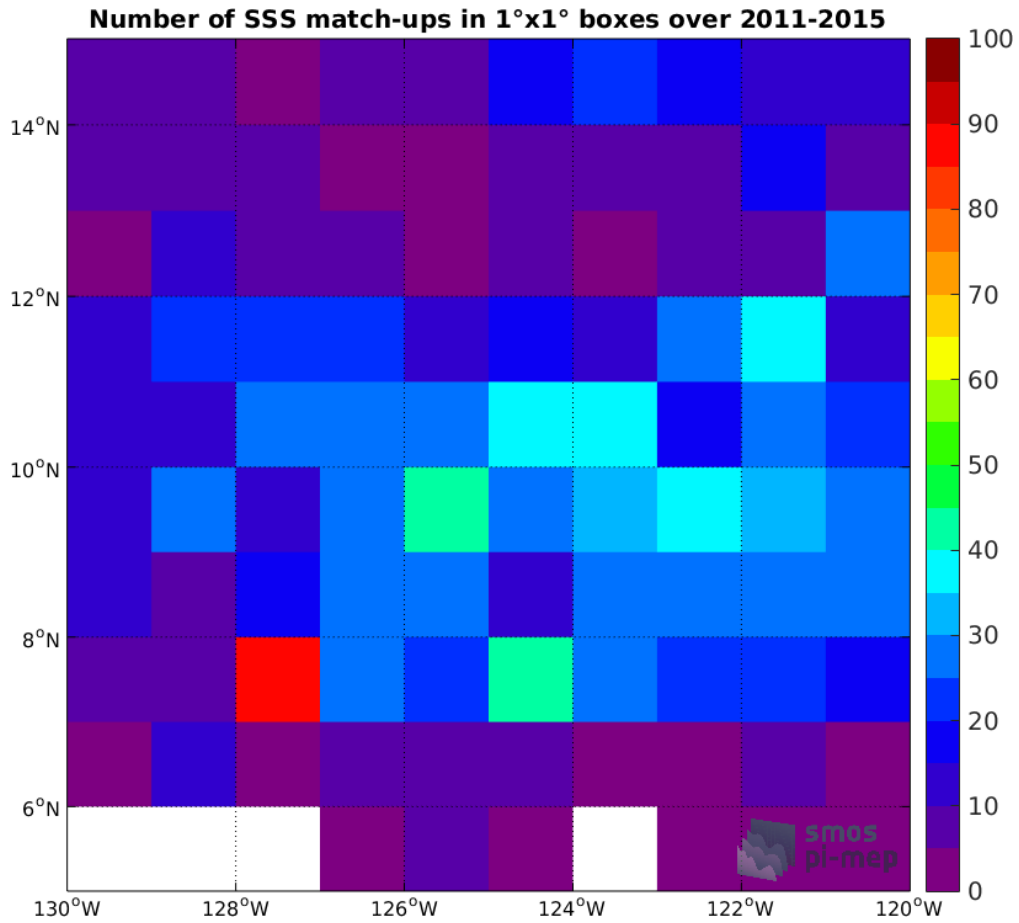
Figure 4: Number of SSS match-ups between Argo SSS and the Aquarius-L3-OR-V5-MONTHLY SSS product for the SPURS 2 Pi-MEP region over 1°x1° boxes and for the full satellite product period.
