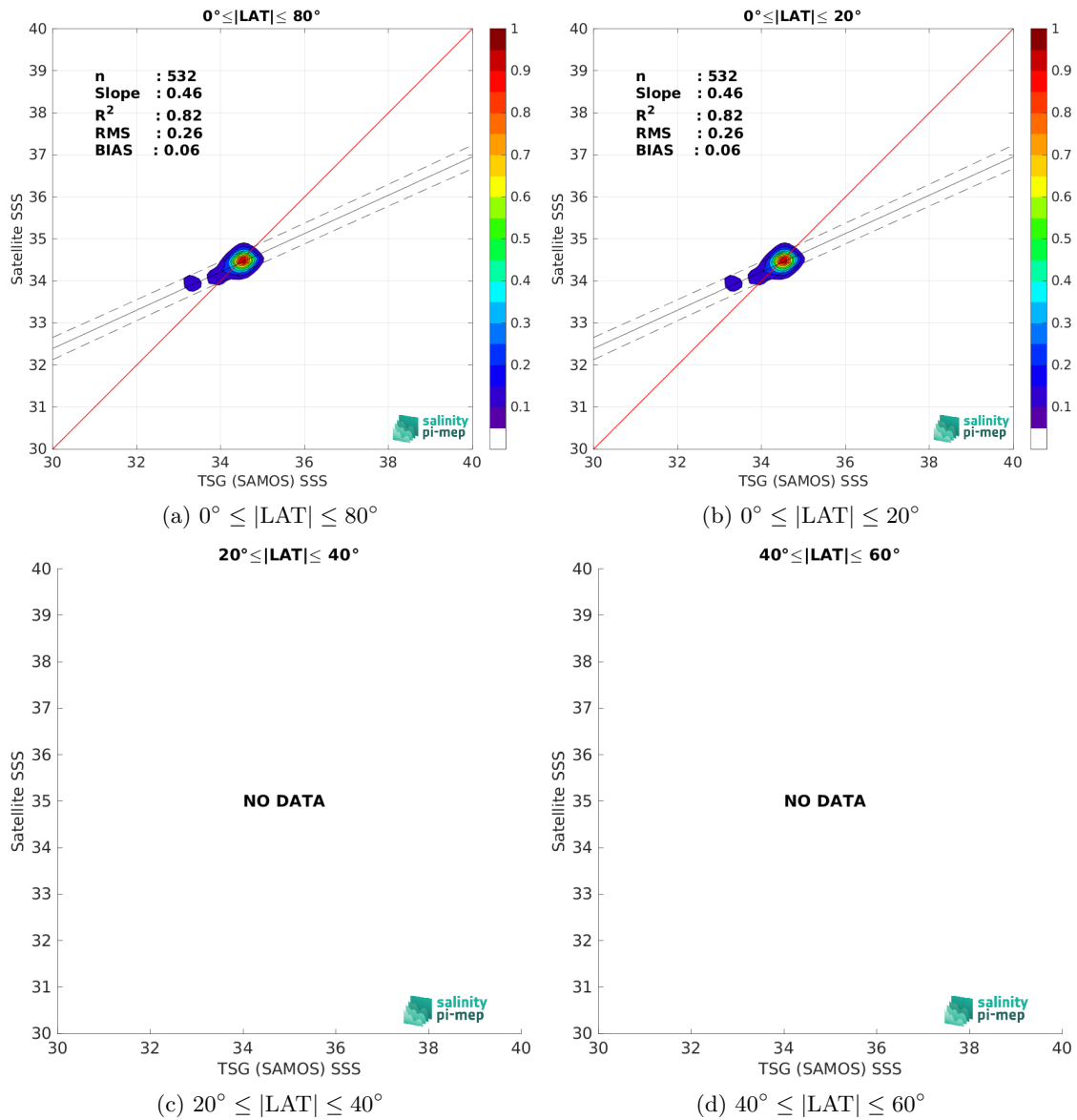
Figure 10: Contour maps of the concentration of Aquarius SSS L3 OR v5 - Monthly - Rain mask (NASA-GSFC) SSS (y-axis) versus TSG (SAMOS) SSS (x-axis) at match-up pairs for different latitude bands. For each plot, the red line shows x=y . The black thin and dashed lines indicate a linear fit through the data cloud and the \pm 95\% confidence levels, respectively. The number match-up pairs n , the slope and R^2 coefficient of the linear fit, the root mean square (RMS) and the mean bias between satellite and in situ data are indicated for each latitude band in each plots.
