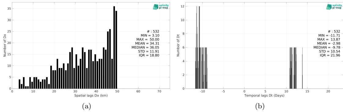
Figure 6: Histograms of the spatial (a) and temporal (b) lags between the location/time of the TSG (SAMOS) measurement and the date of the corresponding Aquarius SSS L3 OR v5 - Monthly - Rain mask (NASA-GSFC) SSS pixel.
