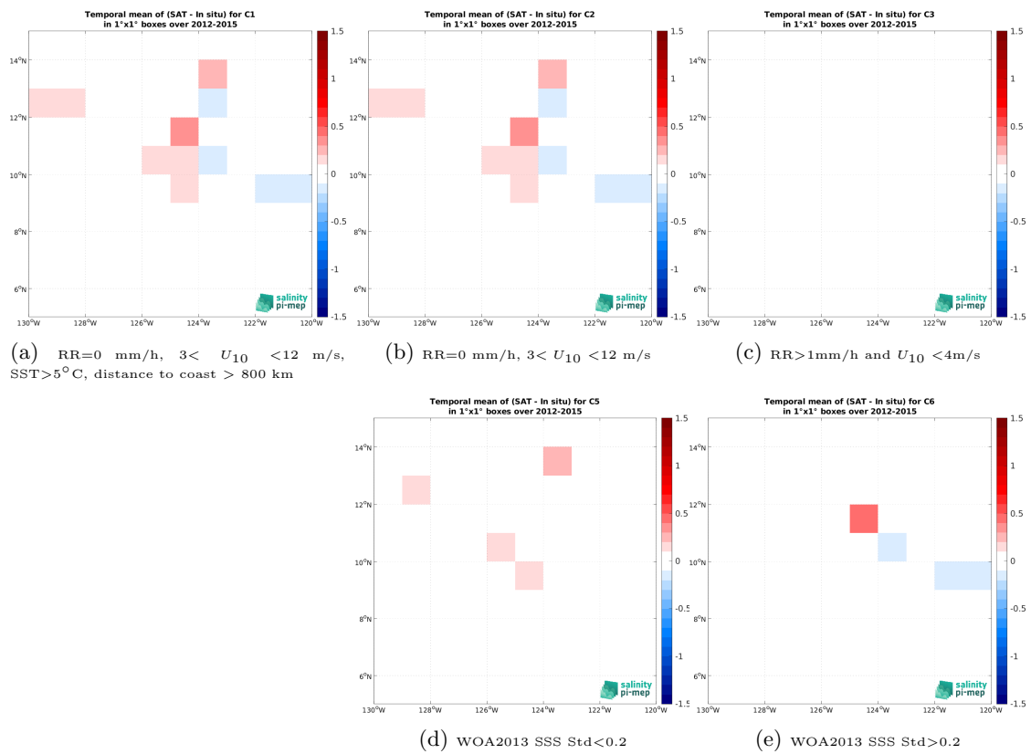
Figure 14: Temporal mean gridded over spatial boxes of size 1^\circ \times 1^\circ of \Delta SSS (Aquarius SSS L3 OR v5 - Monthly - Rain mask (NASA-GSFC) - TSG (SAMOS)) for 5 different subdatasets corresponding to: RR=0 mm/h, 3 < U_{10} < 12 m/s, SST > 5°C, distance to coast > 800 km (a), RR=0 mm/h, 3 < U_{10} < 12 m/s (b), RR > 1mm/h and U_{10} < 4 m/s (c), WOA2013 SSS Std < 0.2 (d), WOA2013 SSS Std > 0.2 (e).
