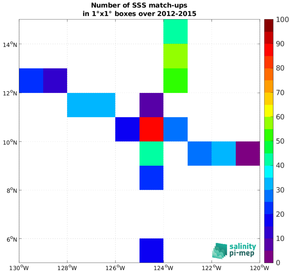
Figure 5: Number of SSS match-ups between TSG (SAMOS) SSS and the Aquarius SSS L3 OR v5 - Monthly - Rain mask (NASA-GSFC) SSS product for the SPURS 2 Pi-MEP region over 1^\circ \times 1^\circ boxes and for the full satellite product period.
