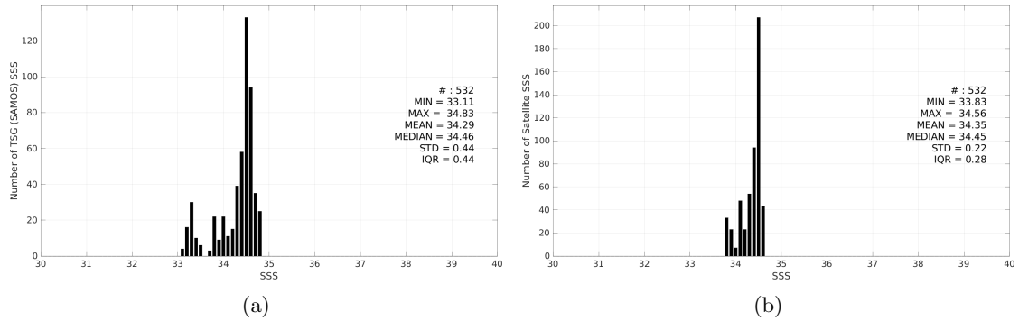
Figure 3: Histograms of SSS from TSG (SAMOS) (a) and Aquarius SSS L3 OR v5 - Monthly - Rain mask (NASA-GSFC) (b) considering all match-up pairs per bins of 0.1 over the SPURS 2 Pi-MEP region and for the full satellite product period.
