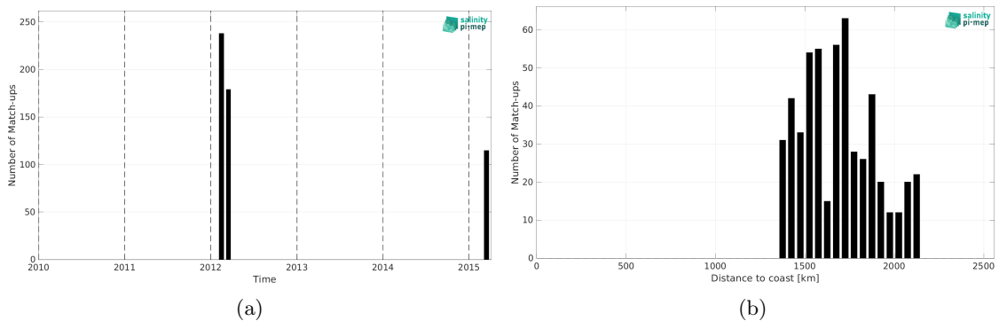
Figure 2: Number of match-ups between TSG (SAMOS) and Aquarius SSS L3 OR v5 - Monthly - Rain mask (NASA-GSFC) SSS as a function of time (a) and as function of the distance to coast (b) over the SPURS 2 Pi-MEP region and for the full satellite product period.
