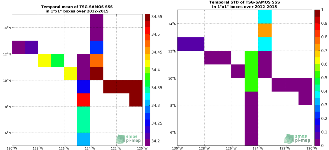
(c) MEAN(TSG-SAMOS SSS)
