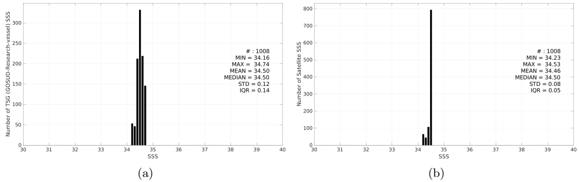
Figure 3: Histograms of SSS from TSG (GOSUD-Research-vessel) (a) and Aquarius SSS L3 OR v5 - Monthly - Rain mask (NASA-GSFC) (b) considering all match-up pairs per bins of 0.1 over the SPURS 2 Pi-MEP region and for the full satellite product period.
