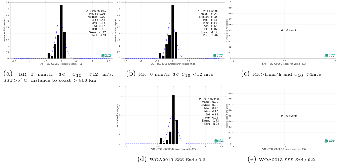
Figure 15: Normalized histogram of \Delta\text{SSS} (Aquarius SSS L3 OR v5 - Monthly - Rain mask (NASA-GSFC) - TSG (GOSUD-Research-vessel)) for 5 different subdatasets corresponding to: RR=0 mm/h, 3 < U_{10} < 12 m/s, SST > 5^\circ\text{C} , distance to coast > 800 km (a), RR=0 mm/h, 3 < U_{10} < 12 m/s (b), RR > 1\text{mm/h} and U_{10} < 4\text{m/s} (c), WOA2013 SSS Std < 0.2 (d), WOA2013 SSS Std > 0.2 (e).
