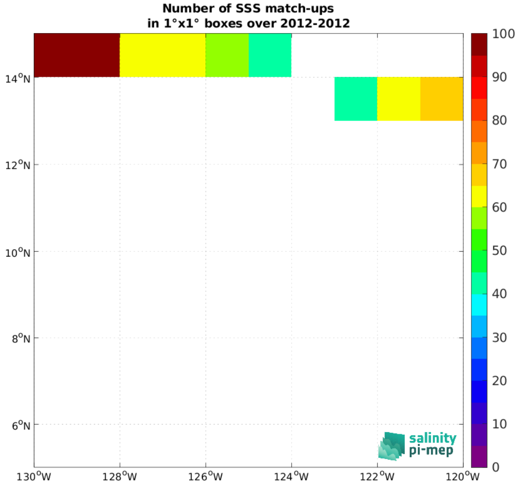
Figure 5: Number of SSS match-ups between TSG (GOSUD-Research-vessel) SSS and the Aquarius SSS L3 OR v5 - Monthly - Rain mask (NASA-GSFC) SSS product for the SPURS 2 Pi-MEP region over 1^\circ \times 1^\circ boxes and for the full satellite product period.
