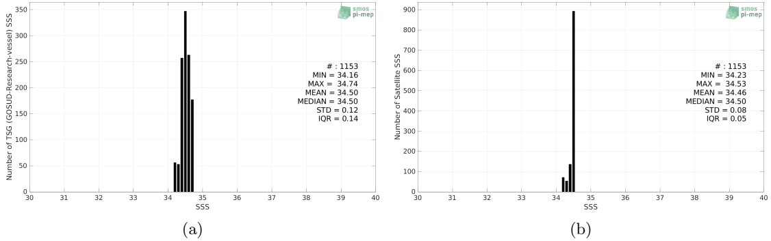
Figure 2: Histograms of SSS from TSG (GOSUD-Research-vessel) (a) and Aquarius SSS L3 OR v5 - Monthly - Rain mask (NASA-GSFC) (b) considering all match-up pairs per bins of 0.1 over the SPURS 2 Pi-MEP region and for the full satellite product period.
