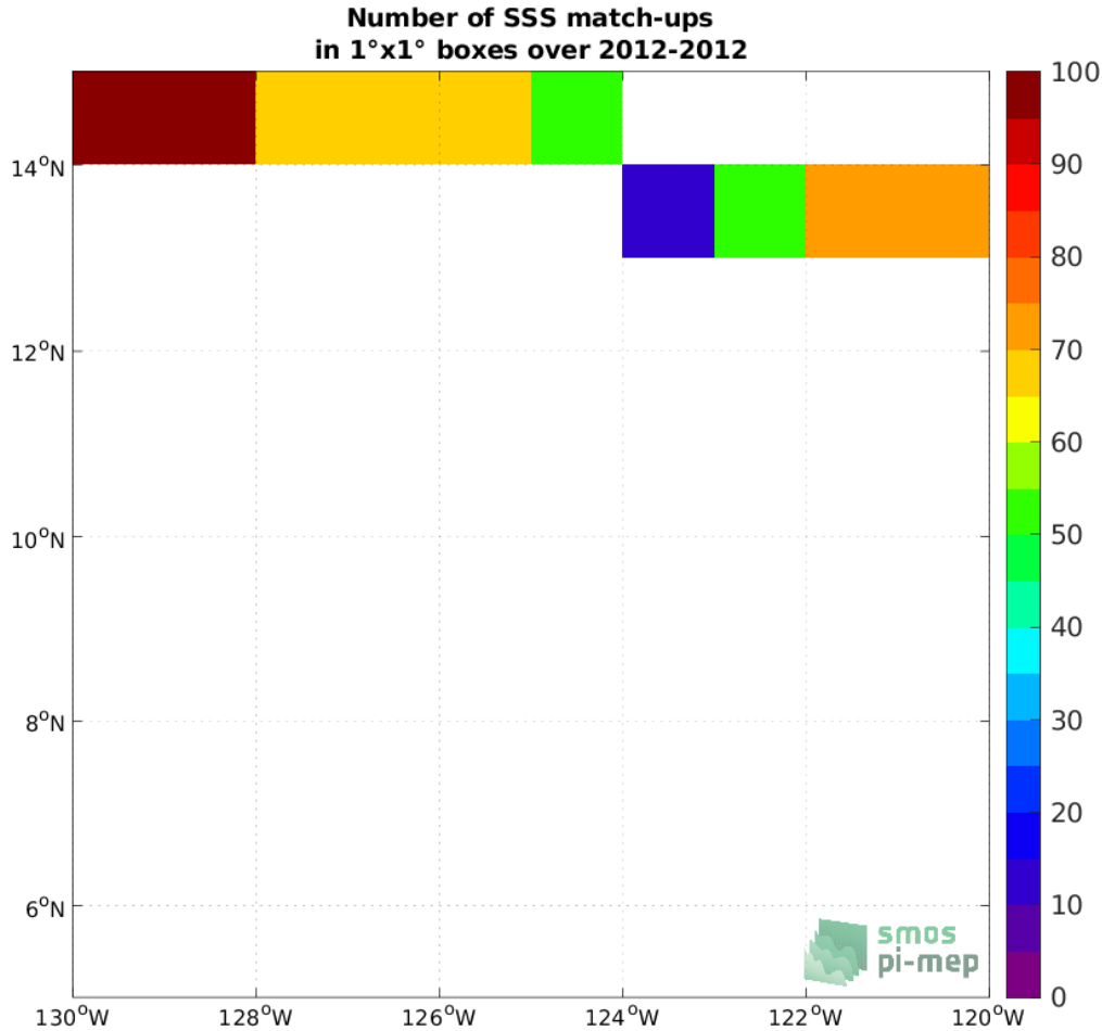
Figure 4: Number of SSS match-ups between TSG (GOSUD-Research-vessel) SSS and the Aquarius SSS L3 OR v5 - Monthly - Rain mask (NASA-GSFC) SSS product for the SPURS 2 Pi-MEP region over 1^\circ \times 1^\circ boxes and for the full satellite product period.
