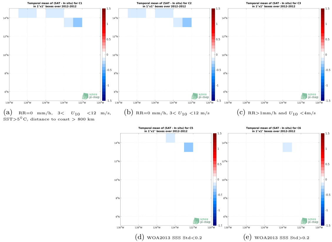
Figure 12: Temporal mean gridded over spatial boxes of size 1^\circ \times 1^\circ of \Delta\text{SSS} (Aquarius SSS L3 OR v5 - Monthly - Rain mask (NASA-GSFC) - TSG (GOSUD-Research-vessel)) for 5 different subdatasets corresponding to: RR=0 mm/h, 3 < U_{10} < 12 m/s, SST > 5^\circ\text{C} , distance to coast > 800 km (a), RR=0 mm/h, 3 < U_{10} < 12 m/s (b), RR > 1\text{mm/h} and U_{10} < 4\text{m/s} (c), WOA2013 SSS Std < 0.2 (d), WOA2013 SSS Std > 0.2 (e).
