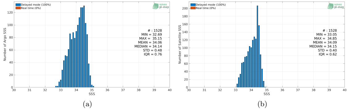
Figure 2: Histograms of SSS from Argo (a) and Aquarius SSS L3 OR v5 - Monthly - Rain mask (NASA-GSFC) (b) considering all match-up pairs per bins of 0.1 over the SPURS 2 Pi-MEP region and for the full satellite product period.
