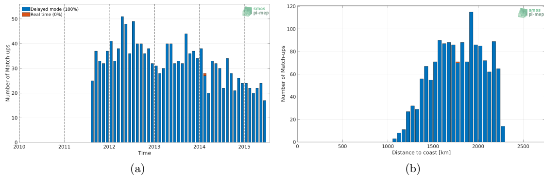
Figure 1: Number of match-ups between Argo and Aquarius SSS L3 OR v5 - Monthly - Rain mask (NASA-GSFC) SSS as a function of time (a) and as function of the distance to coast (b) over the SPURS 2 Pi-MEP region and for the full satellite product period.
