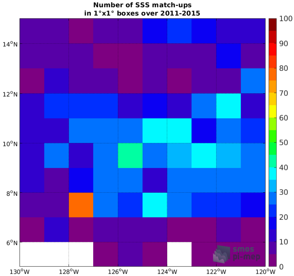
Figure 4: Number of SSS match-ups between Argo SSS and the Aquarius SSS L3 OR v5 - Monthly - Rain mask (NASA-GSFC) SSS product for the SPURS 2 Pi-MEP region over 1°x1° boxes and for the full satellite product period.
