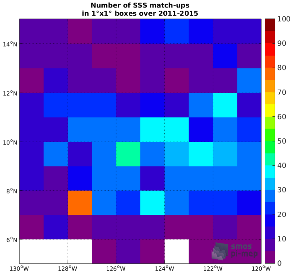
Figure 4: Number of SSS match-ups between Argo SSS and the Aquarius-L3-OR-V5-MONTHLY-RAIN-MASK-1DEG SSS product for the SPURS 2 Pi-MEP region over 1°x1° boxes and for the full satellite product period.
