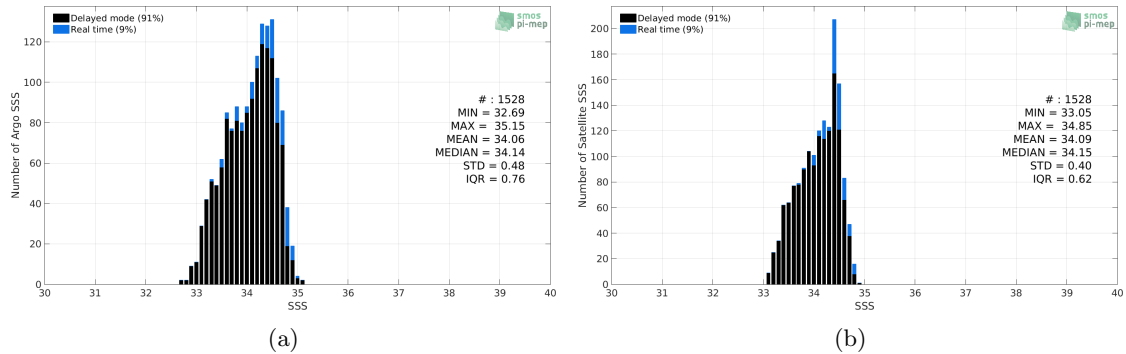
Figure 2: Histograms of SSS from Argo (a) and Aquarius-L3-OR-V5-MONTHLY-RAIN-MASK-1DEG (b) considering all match-up pairs per bins of 0.1 over the SPURS 2 Pi-MEP region and for the full satellite product period.
