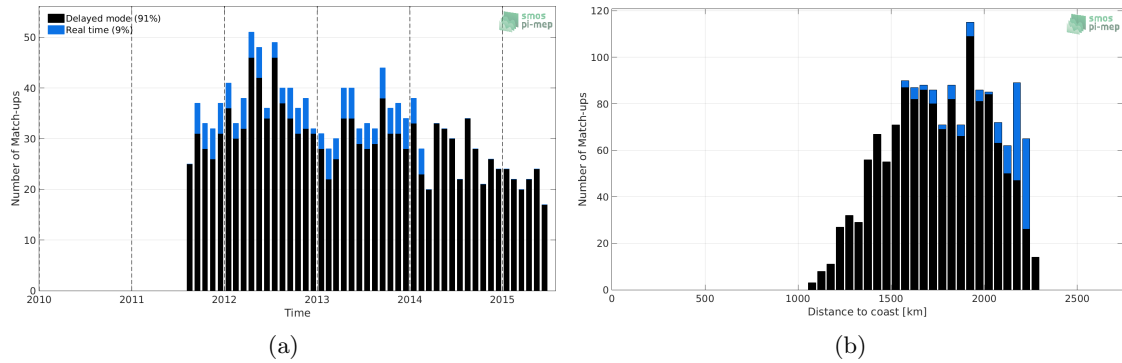
Figure 1: Number of match-ups between Argo and Aquarius-L3-OR-V5-MONTHLY-RAIN-MASK-1DEG SSS as a function of time (a) and as function of the distance to coast (b) over the SPURS 2 Pi-MEP region and for the full satellite product period.
