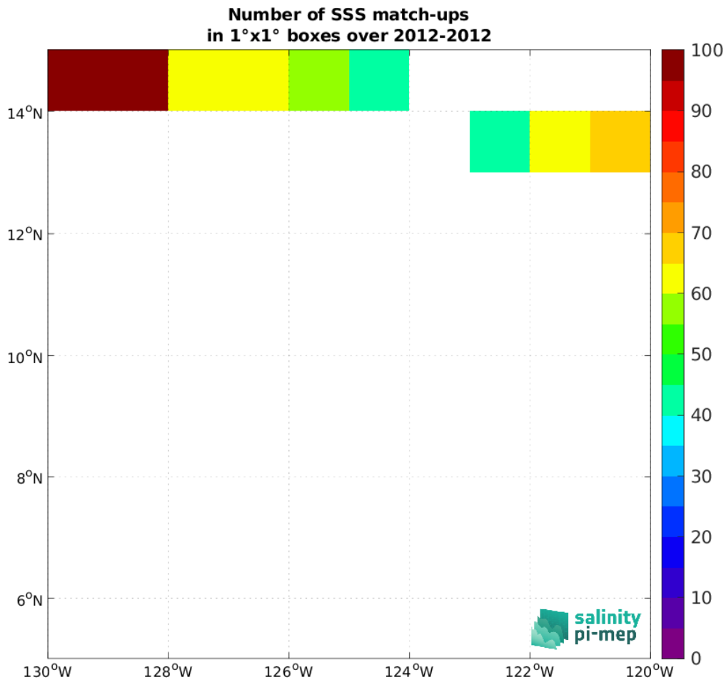
Figure 5: Number of SSS match-ups between TSG (GOSUD-Research-vessel) SSS and the Aquarius SSS L3 CAP v5 - 7-Day running (JPL) SSS product for the SPURS 2 Pi-MEP region over 1°x1° boxes and for the full satellite product period.
