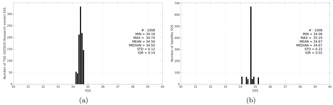
Figure 3: Histograms of SSS from TSG (GOSUD-Research-vessel) (a) and Aquarius SSS L3 CAP v5 - 7-Day running (JPL) (b) considering all match-up pairs per bins of 0.1 over the SPURS 2 Pi-MEP region and for the full satellite product period.
