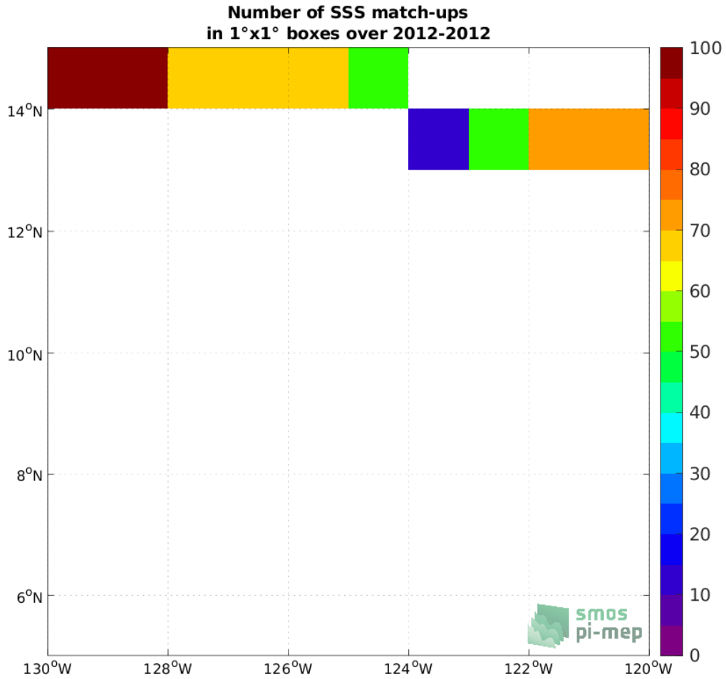
Figure 4: Number of SSS match-ups between TSG (GOSUD-Research-vessel) SSS and the Aquarius SSS L3 CAP v5 - 7-Day running (JPL) SSS product for the SPURS 2 Pi-MEP region over 1^\circ \times 1^\circ boxes and for the full satellite product period.
