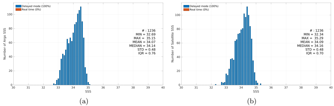
Figure 3: Histograms of SSS from Argo (a) and Aquarius SSS L3 CAP v5 - 7-Day running (JPL) (b) considering all match-up pairs per bins of 0.1 over the SPURS 2 Pi-MEP region and for the full satellite product period.
