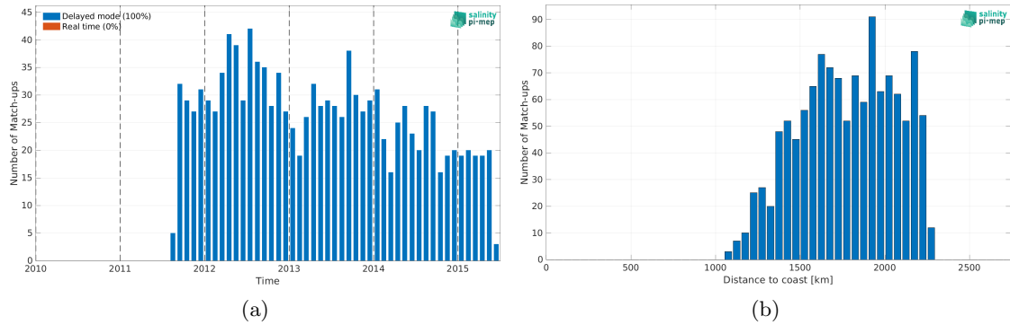
Figure 2: Number of match-ups between Argo and Aquarius SSS L3 CAP v5 - 7-Day running (JPL) SSS as a function of time (a) and as function of the distance to coast (b) over the SPURS 2 Pi-MEP region and for the full satellite product period.
