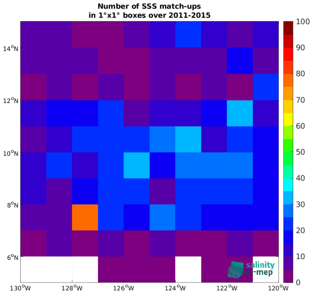
Figure 5: Number of SSS match-ups between Argo SSS and the Aquarius SSS L3 CAP v5 - 7-Day running (JPL) SSS product for the SPURS 2 Pi-MEP region over 1°x1° boxes and for the full satellite product period.
