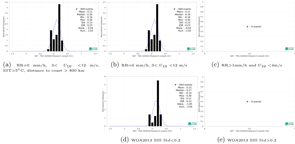
Figure 15: Normalized histogram of \Delta\text{SSS} (Aquarius SSS L3 CAP v5 - Monthly (JPL) - TSG (GOSUD-Research-vessel)) for 5 different subdatasets corresponding to: RR=0 mm/h, 3 < U_{10} < 12 m/s, SST > 5^\circ\text{C} , distance to coast > 800 km (a), RR=0 mm/h, 3 < U_{10} < 12 m/s (b), RR > 1\text{mm/h} and U_{10} < 4\text{m/s} (c), WOA2013 SSS Std < 0.2 (d), WOA2013 SSS Std > 0.2 (e).
