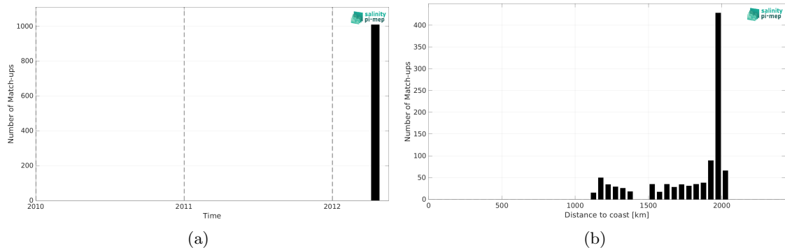
Figure 2: Number of match-ups between TSG (GOSUD-Research-vessel) and Aquarius SSS L3 CAP v5 - Monthly (JPL) SSS as a function of time (a) and as function of the distance to coast (b) over the SPURS 2 Pi-MEP region and for the full satellite product period.
