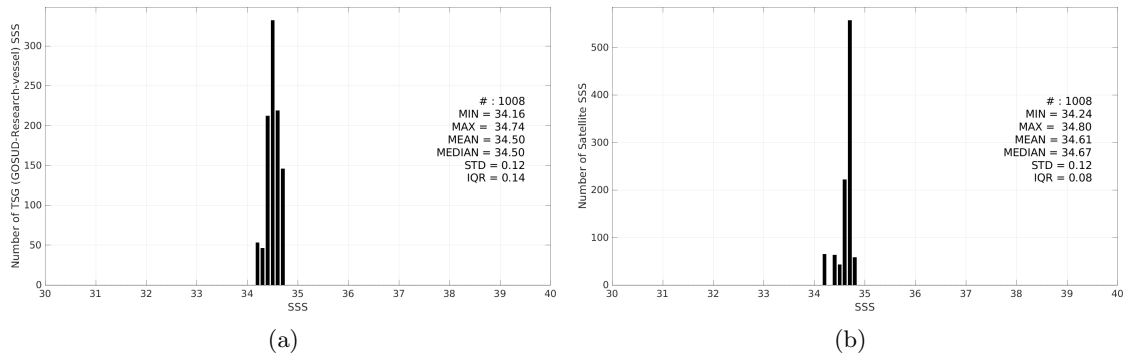
Figure 3: Histograms of SSS from TSG (GOSUD-Research-vessel) (a) and Aquarius SSS L3 CAP v5 - Monthly (JPL) (b) considering all match-up pairs per bins of 0.1 over the SPURS 2 Pi-MEP region and for the full satellite product period.
