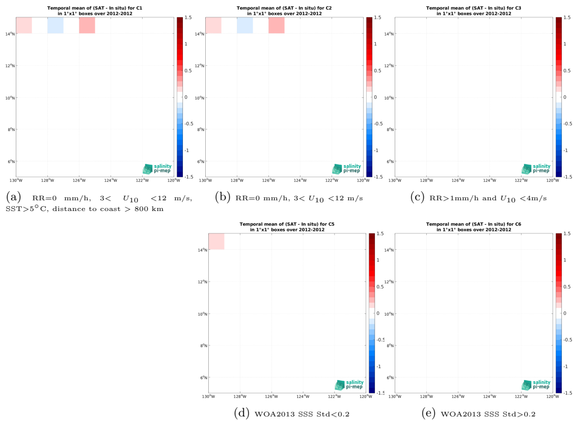
Figure 14: Temporal mean gridded over spatial boxes of size 1^\circ \times 1^\circ of \Delta\text{SSS} (Aquarius SSS L3 CAP v5 - Monthly (JPL) - TSG (GOSUD-Research-vessel)) for 5 different subdatasets corresponding to:RR=0 mm/h, 3 < U_{10} < 12 m/s, SST >5^\circ\text{C} , distance to coast > 800 km (a), RR=0 mm/h, 3 < U_{10} < 12 m/s (b), RR >1 mm/h and U_{10} < 4 m/s (c), WOA2013 SSS Std <0.2 (d), WOA2013 SSS Std >0.2 (e).
