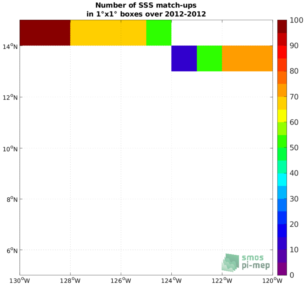
Figure 4: Number of SSS match-ups between TSG (GOSUD-Research-vessel) SSS and the Aquarius SSS L3 CAP v5 - Monthly (JPL) SSS product for the SPURS 2 Pi-MEP region over 1^\circ \times 1^\circ boxes and for the full satellite product period.
