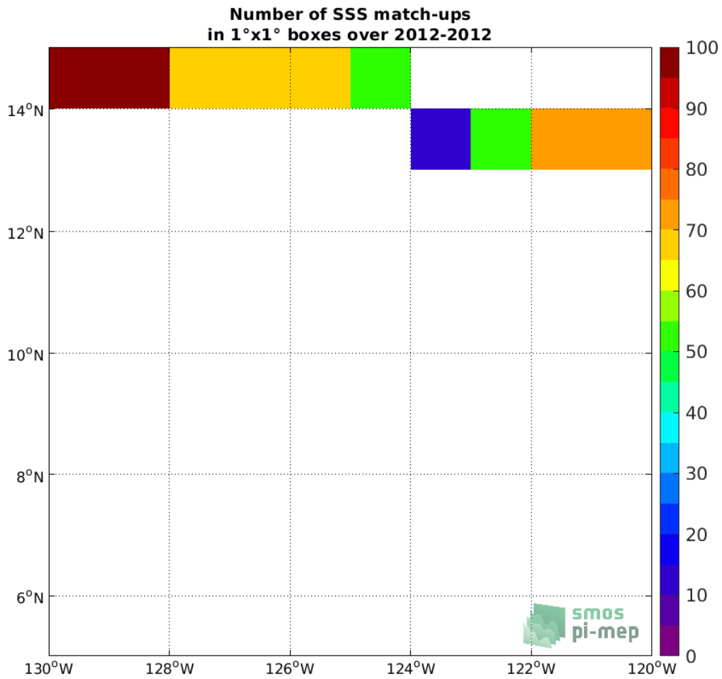
Figure 4: Number of SSS match-ups between TSG (GOSUD-Research-vessel) SSS and the Aquarius SSS L3 CAP v5 - Monthly (JPL) SSS product for the SPURS 2 Pi-MEP region over 1°x1° boxes and for the full satellite product period.
