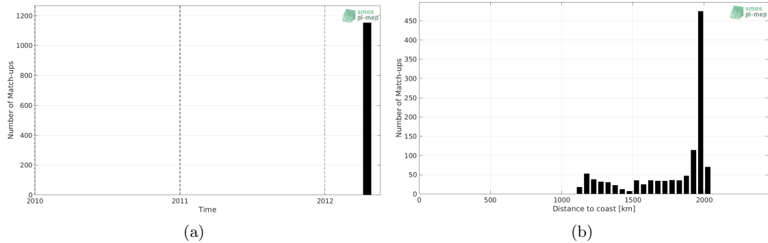
Figure 1: Number of match-ups between TSG (GOSUD-Research-vessel) and Aquarius SSS L3 CAP v5 - Monthly (JPL) SSS as a function of time (a) and as function of the distance to coast (b) over the SPURS 2 Pi-MEP region and for the full satellite product period.
