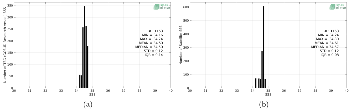
Figure 2: Histograms of SSS from TSG (GOSUD-Research-vessel) (a) and Aquarius SSS L3 CAP v5 - Monthly (JPL) (b) considering all match-up pairs per bins of 0.1 over the SPURS 2 Pi-MEP region and for the full satellite product period.
