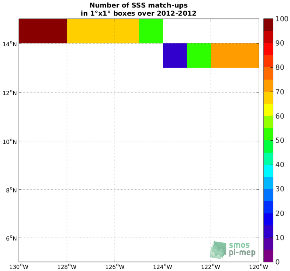
Figure 4: Number of SSS match-ups between TSG-GOSUD-Research-vessel SSS and the Aquarius-L3-JPL-V5-MONTHLY SSS product for the SPURS 2 Pi-MEP region over 1°x1° boxes and for the full satellite product period.
