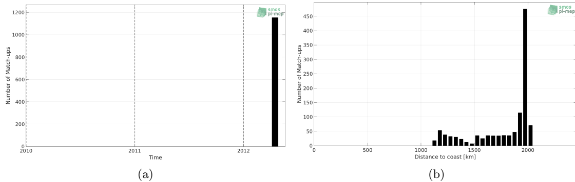
Figure 1: Number of match-ups between TSG-GOSUD-Research-vessel and Aquarius-L3-JPL-V5-MONTHLY SSS as a function of time (a) and as function of the distance to coast (b) over the SPURS 2 Pi-MEP region and for the full satellite product period.
