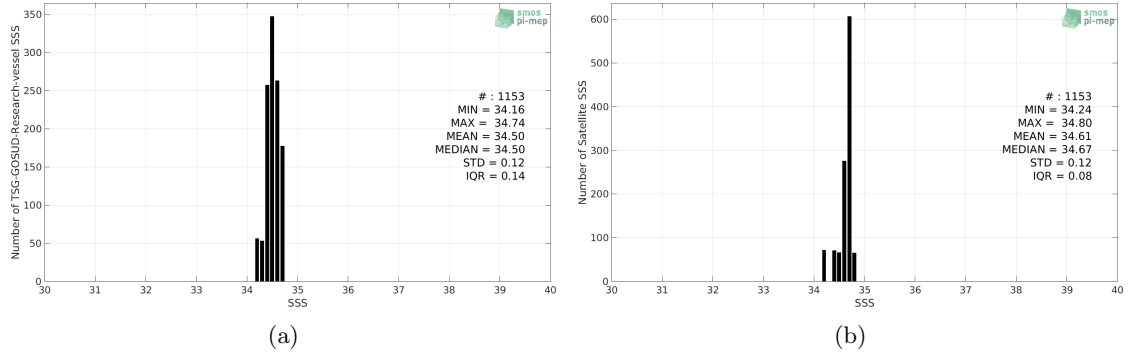
Figure 2: Histograms of SSS from TSG-GOSUD-Research-vessel (a) and Aquarius-L3-JPL-V5-MONTHLY (b) considering all match-up pairs per bins of 0.1 over the SPURS 2 Pi-MEP region and for the full satellite product period.
