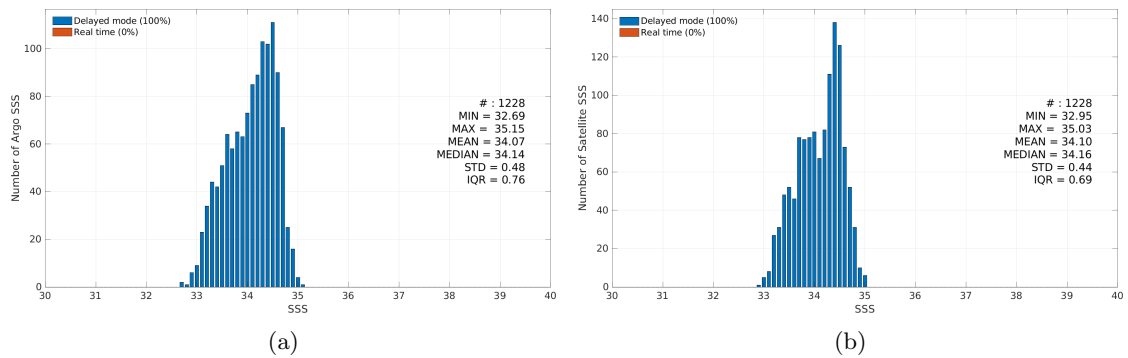
Figure 3: Histograms of SSS from Argo (a) and Aquarius SSS L3 CAP v5 - Monthly (JPL) (b) considering all match-up pairs per bins of 0.1 over the SPURS 2 Pi-MEP region and for the full satellite product period.
