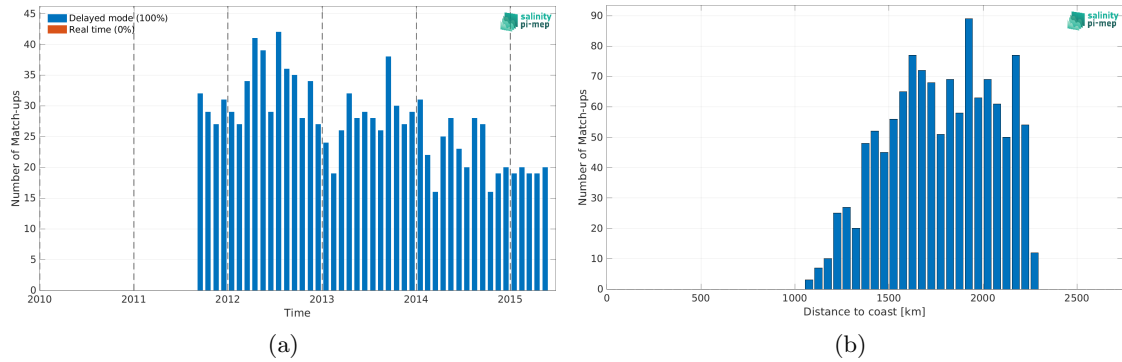
Figure 2: Number of match-ups between Argo and Aquarius SSS L3 CAP v5 - Monthly (JPL) SSS as a function of time (a) and as function of the distance to coast (b) over the SPURS 2 Pi-MEP region and for the full satellite product period.
