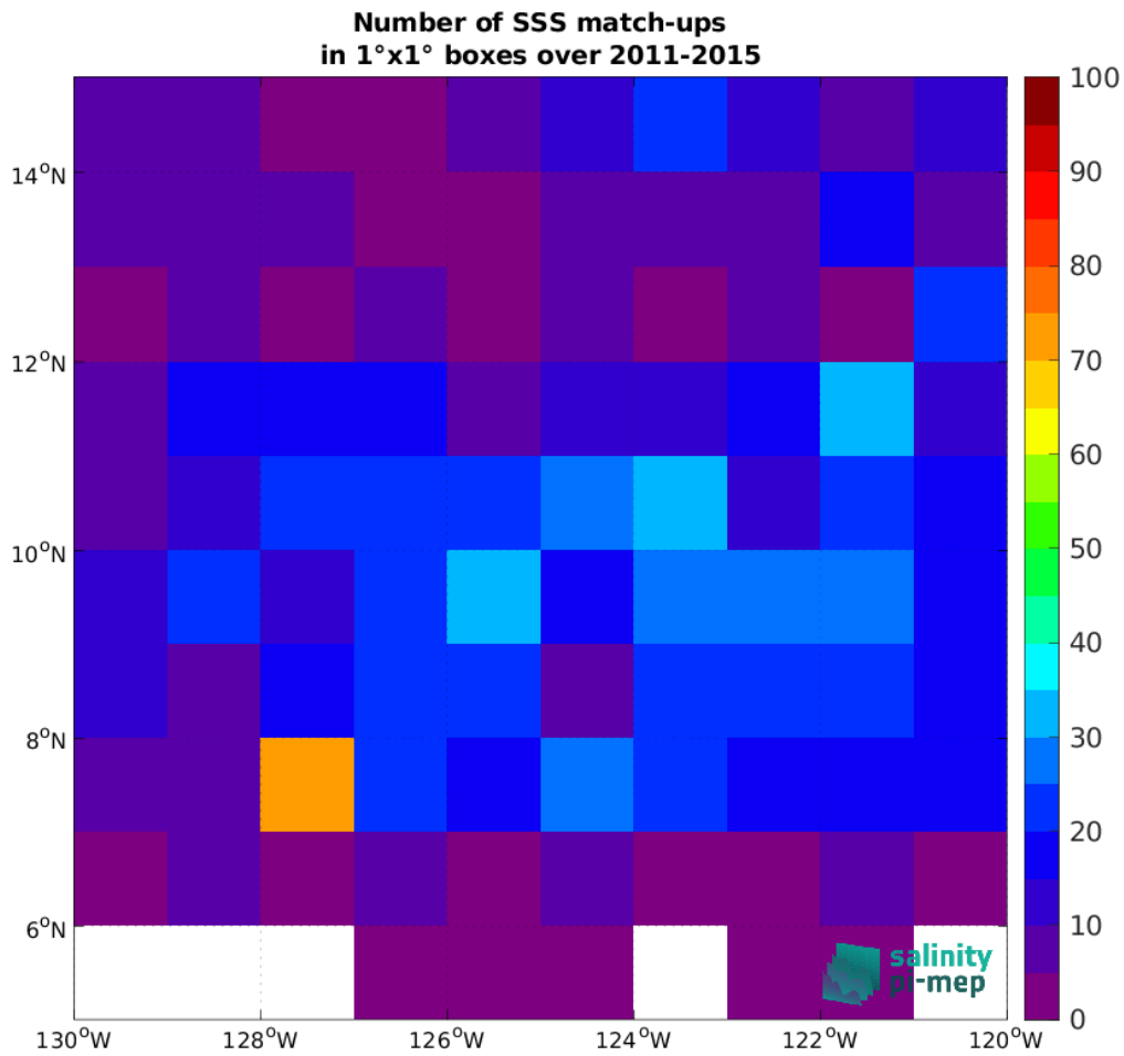
Figure 5: Number of SSS match-ups between Argo SSS and the Aquarius SSS L3 CAP v5 - Monthly (JPL) SSS product for the SPURS 2 Pi-MEP region over 1°x1° boxes and for the full satellite product period.
