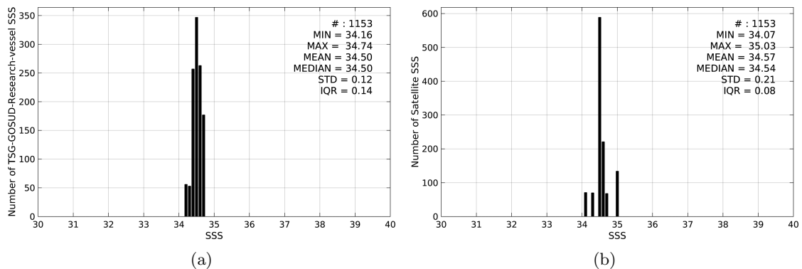
Figure 2: Histograms of SSS from TSG-GOSUD-Research-vessel (a) and Aquarius-L3-JPL-V4-7DAY-RUNNING (b) considering all match-up pairs per bins of 0.1 over the SPURS 2 Pi-MEP region and for the full satellite product period.
