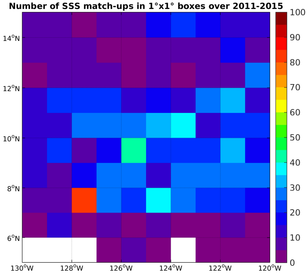
Figure 4: Number of SSS match-ups between Argo SSS and the Aquarius-L3-JPL-V4-7DAY-RUNNING SSS product for the SPURS 2 Pi-MEP region over 1°x1° boxes and for the full satellite product period.
