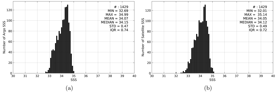
Figure 2: Histograms of SSS from Argo (a) and Aquarius-L3-JPL-V4-7DAY-RUNNING (b) considering all match-up pairs per bins of 0.1 over the SPURS 2 Pi-MEP region and for the full satellite product period.
