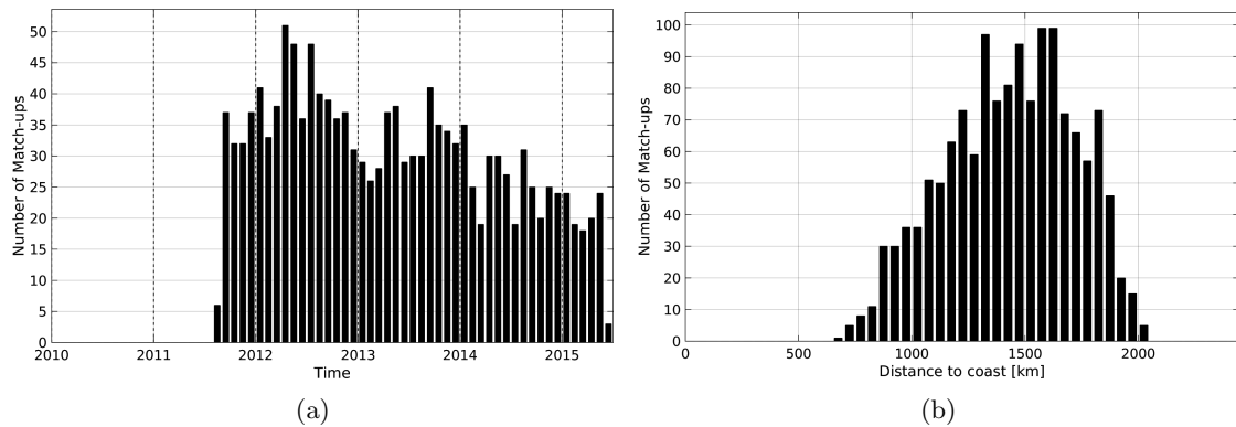
Figure 1: Number of match-ups between Argo and Aquarius-L3-JPL-V4-7DAY-RUNNING SSS as a function of time (a) and as function of the distance to coast (b) over the SPURS 2 Pi-MEP region and for the full satellite product period.
