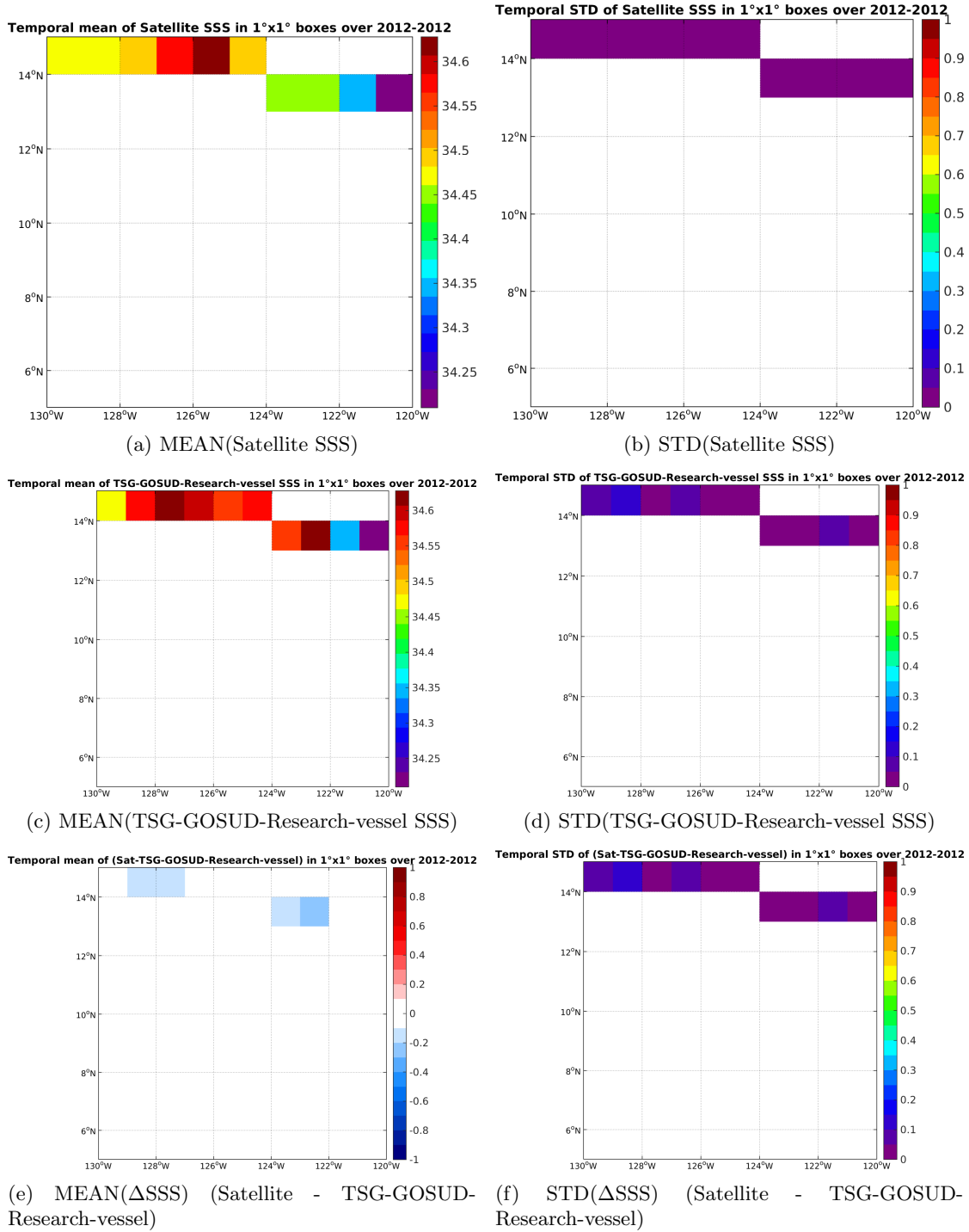
Figure 6: Temporal mean (left) and STD (right) of SSS from Aquarius-L3-JPL-V4-MONTHLY (top), TSG-GOSUD-Research-vessel (middle), and of \Delta SSS (Satellite - TSG-GOSUD-Research-vessel). Only match-up pairs are used to generate these maps.
