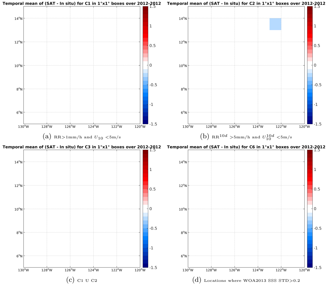
Figure 12: Temporal mean gridded over spatial boxes of size 1°x1° of \Delta SSS (Aquarius-L3-JPL-V4-MONTHLY - TSG-GOSUD-Research-vessel) for 4 different subdatasets corresponding to: RR > 1mm/h and U_{10} < 5m/s (a), RR^{10d} > 5mm/h and U_{10}^{10d} < 5m/s (b), C1 U C2 (c), Locations where WOA2013 SSS STD > 0.2 (d).
