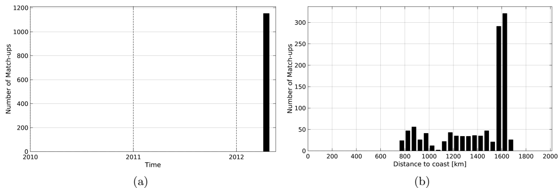
Figure 1: Number of match-ups between TSG-GOSUD-Research-vessel and Aquarius-L3-JPL-V4-MONTHLY SSS as a function of time (a) and as function of the distance to coast (b) over the SPURS 2 Pi-MEP region and for the full satellite product period.
