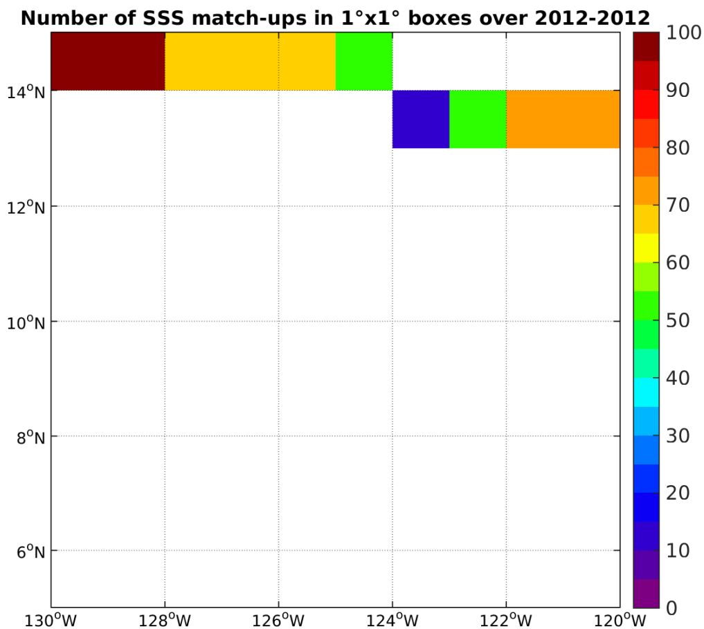
Figure 4: Number of SSS match-ups between TSG-GOSUD-Research-vessel SSS and the Aquarius-L3-JPL-V4-MONTHLY SSS product for the SPURS 2 Pi-MEP region over 1°x1° boxes and for the full satellite product period.
