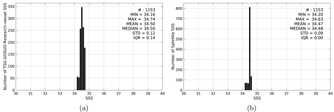
Figure 2: Histograms of SSS from TSG-GOSUD-Research-vessel (a) and Aquarius-L3-JPL-V4-MONTHLY (b) considering all match-up pairs per bins of 0.1 over the SPURS 2 Pi-MEP region and for the full satellite product period.
