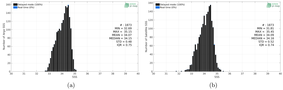
Figure 2: Histograms of SSS from Argo (a) and Aquarius SSS L2-AVERAGED CAP v5 (JPL) (b) considering all match-up pairs per bins of 0.1 over the SPURS 2 Pi-MEP region and for the full satellite product period.
