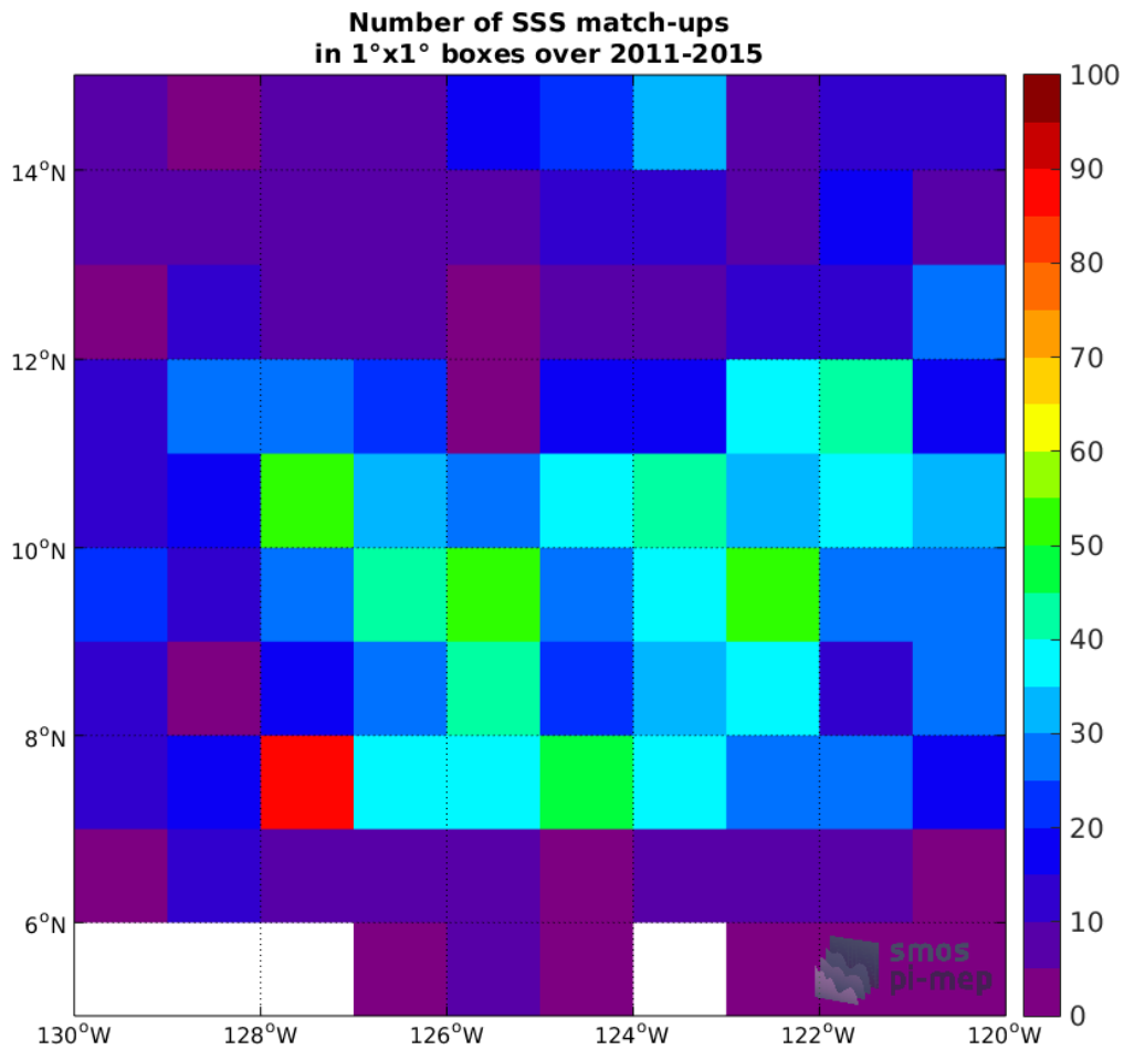
Figure 4: Number of SSS match-ups between Argo SSS and the Aquarius SSS L2-AVERAGED CAP v5 (JPL) SSS product for the SPURS 2 Pi-MEP region over 1°x1° boxes and for the full satellite product period.
