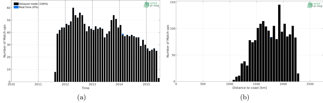
Figure 1: Number of match-ups between Argo and Aquarius SSS L2-AVERAGED CAP v5 (JPL) SSS as a function of time (a) and as function of the distance to coast (b) over the SPURS 2 Pi-MEP region and for the full satellite product period.
