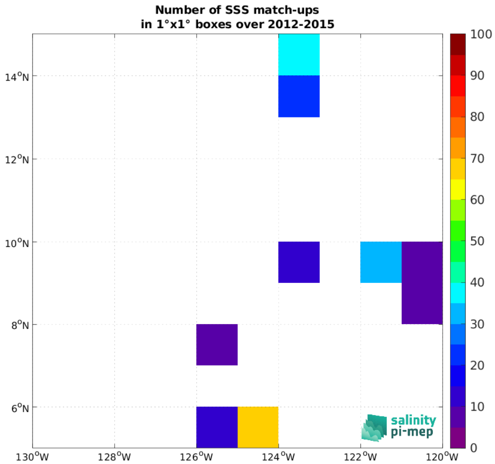
Figure 5: Number of SSS match-ups between TSG (SAMOS) SSS and the Aquarius SSS L2 OR v5 (NASA-GSFC) SSS product for the SPURS 2 Pi-MEP region over 1°x1° boxes and for the full satellite product period.
