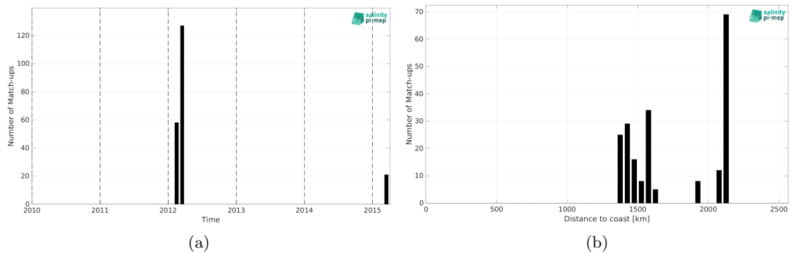
Figure 2: Number of match-ups between TSG (SAMOS) and Aquarius SSS L2 OR v5 (NASA-GSFC) SSS as a function of time (a) and as function of the distance to coast (b) over the SPURS 2 Pi-MEP region and for the full satellite product period.
