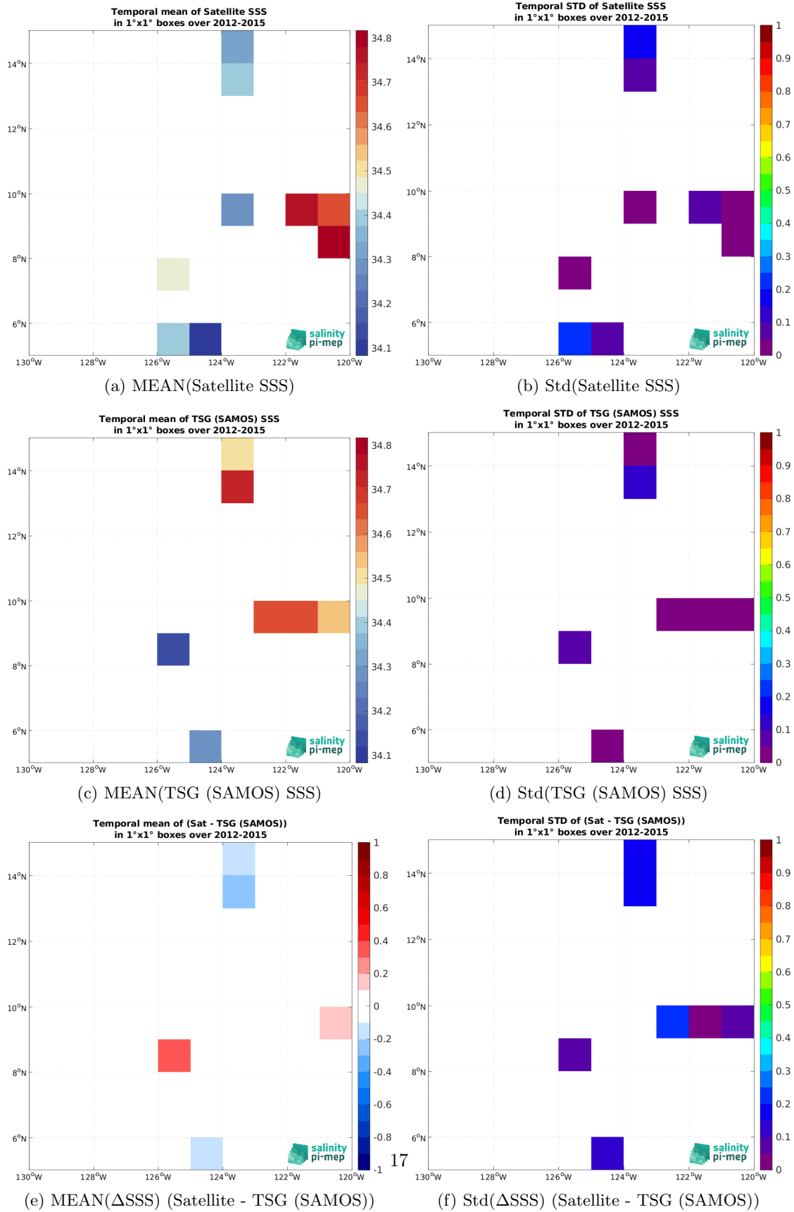
Figure 7: Temporal mean (left) and Std (right) of SSS from Aquarius SSS L2 OR v5 (NASA-GSFC) (top), TSG (SAMOS) (middle), and of \Delta SSS (Satellite - TSG (SAMOS)). Only match-up pairs are used to generate these maps.
