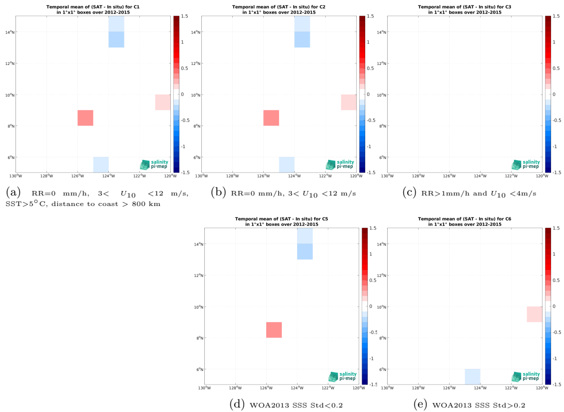
Figure 14: Temporal mean gridded over spatial boxes of size 1^\circ \times 1^\circ of \Delta SSS (Aquarius SSS L2 OR v5 (NASA-GSFC) - TSG (SAMOS)) for 5 different subdatasets corresponding to:RR=0 mm/h, 3 < U_{10} < 12 m/s, SST>5°C, distance to coast > 800 km (a), RR=0 mm/h, 3 < U_{10} < 12 m/s (b), RR>1mm/h and U_{10} < 4 m/s (c), WOA2013 SSS Std<0.2 (d), WOA2013 SSS Std>0.2 (e).
