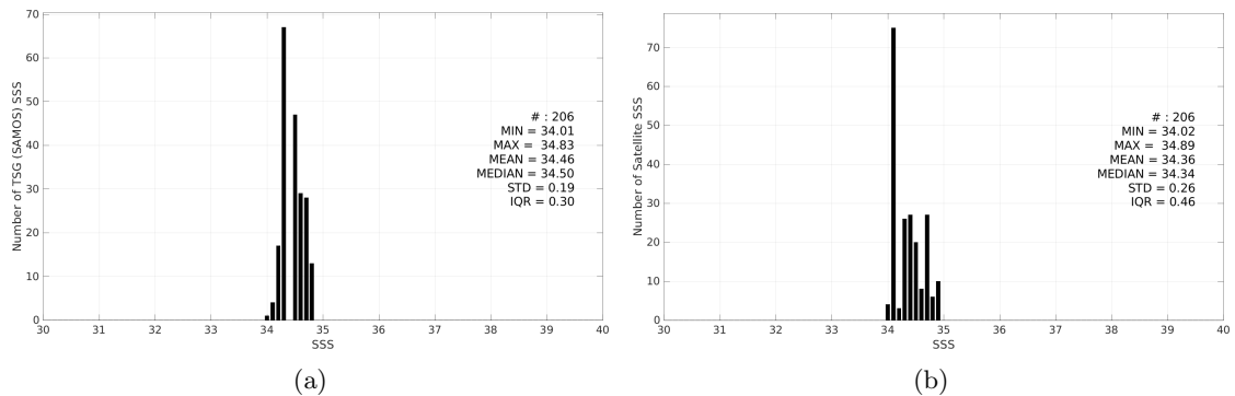
Figure 3: Histograms of SSS from TSG (SAMOS) (a) and Aquarius SSS L2 OR v5 (NASA-GSFC) (b) considering all match-up pairs per bins of 0.1 over the SPURS 2 Pi-MEP region and for the full satellite product period.
