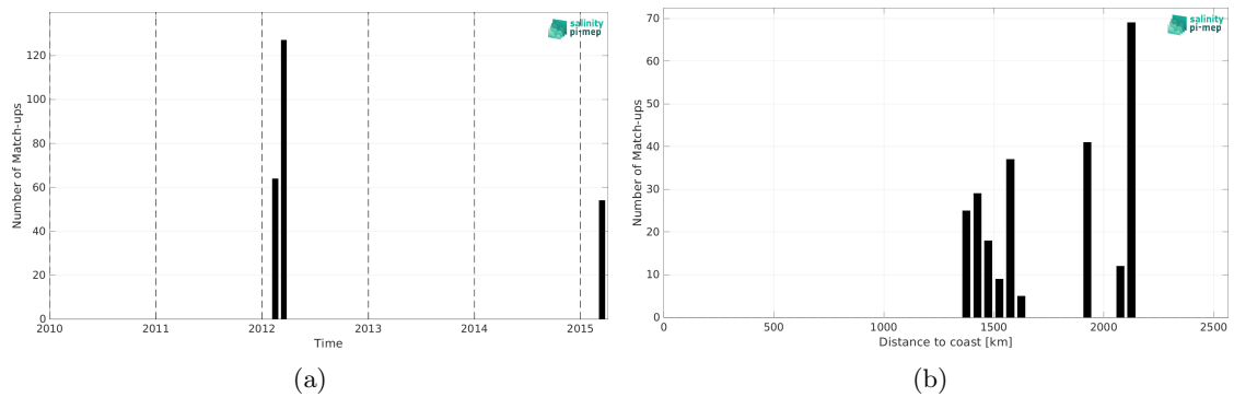
Figure 1: Number of match-ups between TSG (SAMOS) and Aquarius SSS L2 OR v5 (NASA-GSFC) SSS as a function of time (a) and as function of the distance to coast (b) over the SPURS 2 Pi-MEP region and for the full satellite product period.
