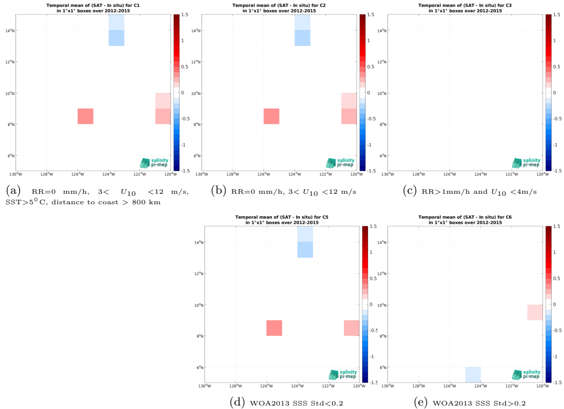
Figure 12: Temporal mean gridded over spatial boxes of size 1^\circ \times 1^\circ of \Delta SSS (Aquarius SSS L2 OR v5 (NASA-GSFC) - TSG (SAMOS)) for 5 different subdatasets corresponding to:RR=0 mm/h, 3 < U_{10} < 12 m/s, SST >5^\circ\text{C} , distance to coast > 800 km (a), RR=0 mm/h, 3 < U_{10} < 12 m/s (b), RR >1 mm/h and U_{10} < 4 m/s (c), WOA2013 SSS Std <0.2 (d), WOA2013 SSS Std >0.2 (e).
