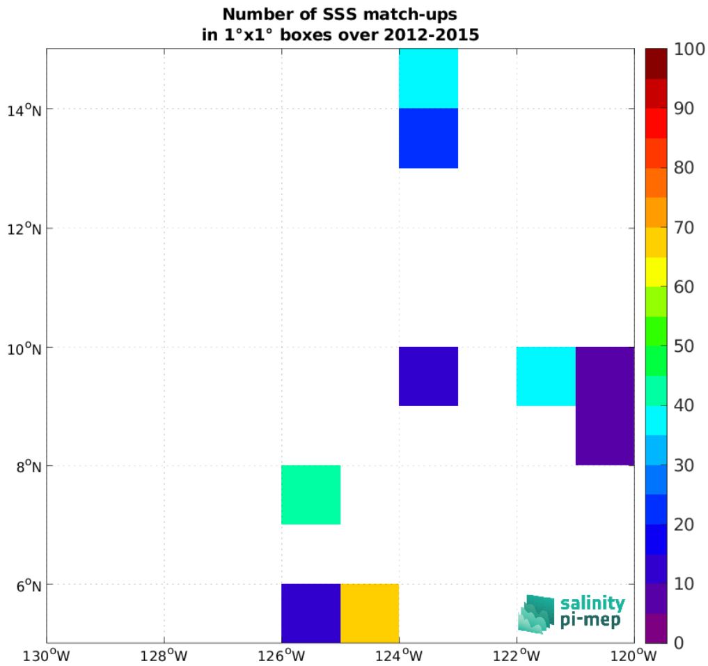
Figure 4: Number of SSS match-ups between TSG (SAMOS) SSS and the Aquarius SSS L2 OR v5 (NASA-GSFC) SSS product for the SPURS 2 Pi-MEP region over 1°x1° boxes and for the full satellite product period.
