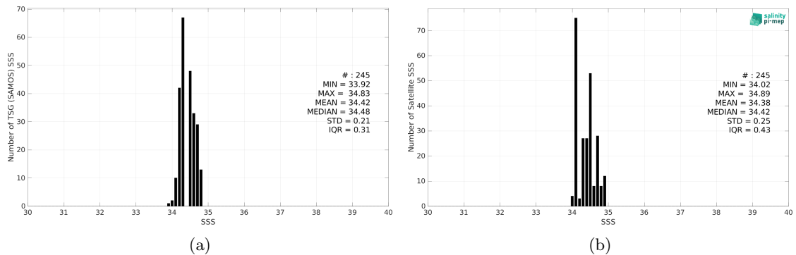
Figure 2: Histograms of SSS from TSG (SAMOS) (a) and Aquarius SSS L2 OR v5 (NASA-GSFC) (b) considering all match-up pairs per bins of 0.1 over the SPURS 2 Pi-MEP region and for the full satellite product period.
