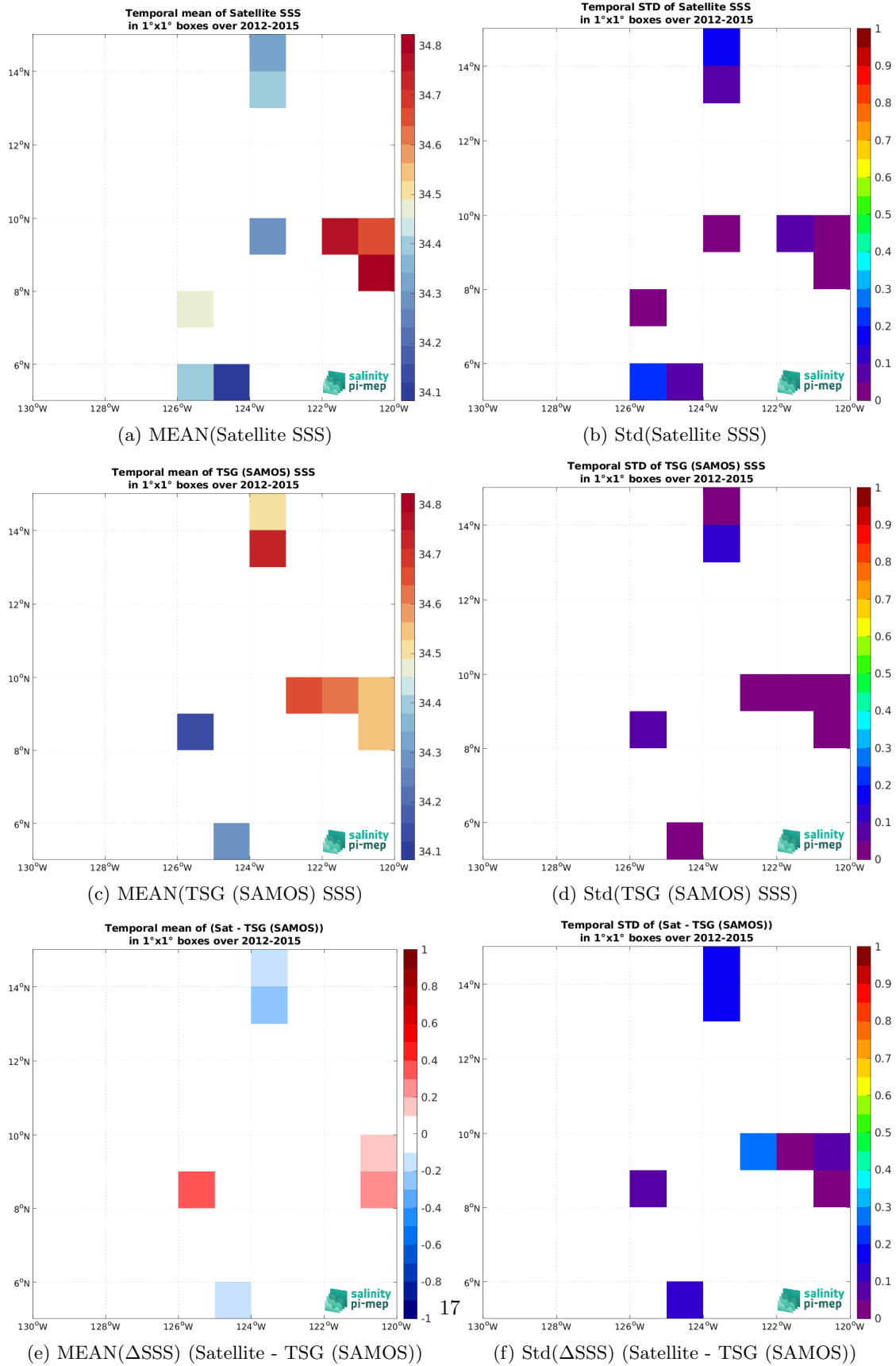
Figure 6: Temporal mean (left) and Std (right) of SSS from Aquarius SSS L2 OR v5 (NASA-GSFC) (top), TSG (SAMOS) (middle), and of \Delta SSS (Satellite - TSG (SAMOS)). Only match-up pairs are used to generate these maps.
