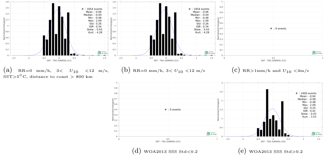
Figure 13: Normalized histogram of \Delta\text{SSS} (Aquarius SSS L2 OR v5 (NASA-GSFC) - TSG (SAMOS)) for 5 different subdatasets corresponding to: RR=0 mm/h, 3 < U_{10} < 12 m/s, SST > 5^\circ\text{C} , distance to coast > 800 km (a), RR=0 mm/h, 3 < U_{10} < 12 m/s (b), RR > 1\text{mm/h} and U_{10} < 4\text{m/s} (c), WOA2013 SSS Std < 0.2 (d), WOA2013 SSS Std > 0.2 (e).
