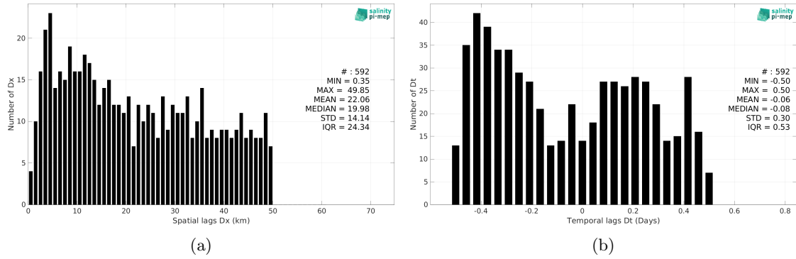
Figure 6: Histograms of the spatial (a) and temporal (b) lags between the location/time of the TSG (GOSUD-Research-vessel) measurement and the date of the corresponding Aquarius SSS L2 OR v5 (NASA-GSFC) SSS pixel.
