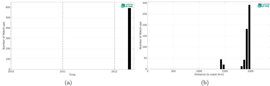
Figure 2: Number of match-ups between TSG (GOSUD-Research-vessel) and Aquarius SSS L2 OR v5 (NASA-GSFC) SSS as a function of time (a) and as function of the distance to coast (b) over the SPURS 2 Pi-MEP region and for the full satellite product period.
