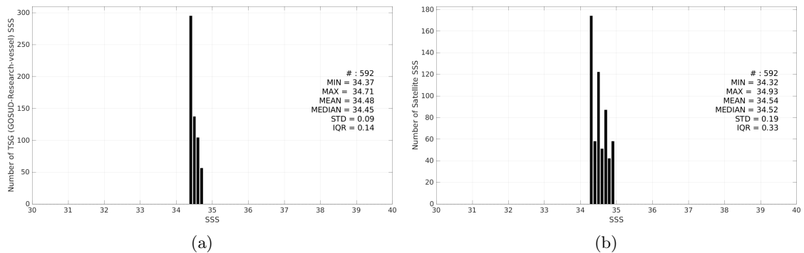
Figure 3: Histograms of SSS from TSG (GOSUD-Research-vessel) (a) and Aquarius SSS L2 OR v5 (NASA-GSFC) (b) considering all match-up pairs per bins of 0.1 over the SPURS 2 Pi-MEP region and for the full satellite product period.
