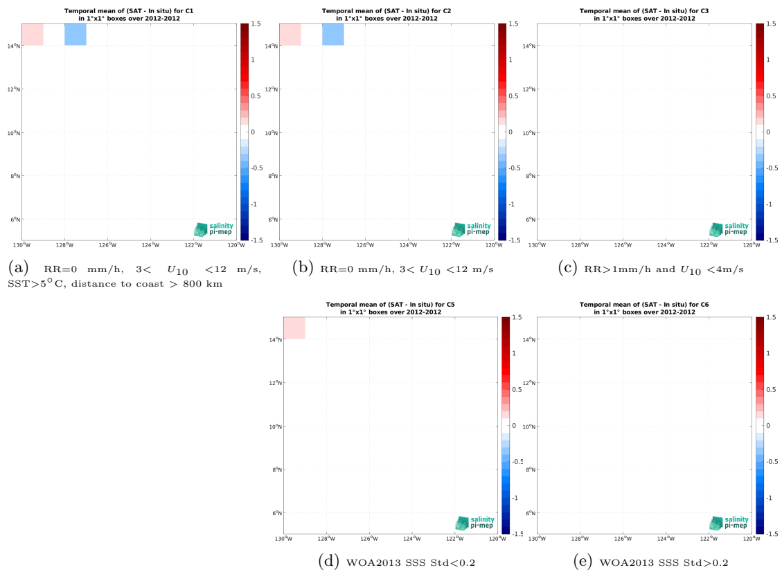
Figure 14: Temporal mean gridded over spatial boxes of size 1^\circ \times 1^\circ of \Delta\text{SSS} (Aquarius SSS L2 OR v5 (NASA-GSFC) - TSG (GOSUD-Research-vessel)) for 5 different subdatasets corresponding to:RR=0 mm/h, 3 < U_{10} < 12 m/s, SST>5°C, distance to coast > 800 km (a), RR=0 mm/h, 3 < U_{10} < 12 m/s (b), RR>1mm/h and U_{10} < 4 m/s (c), WOA2013 SSS Std<0.2 (d), WOA2013 SSS Std>0.2 (e).
