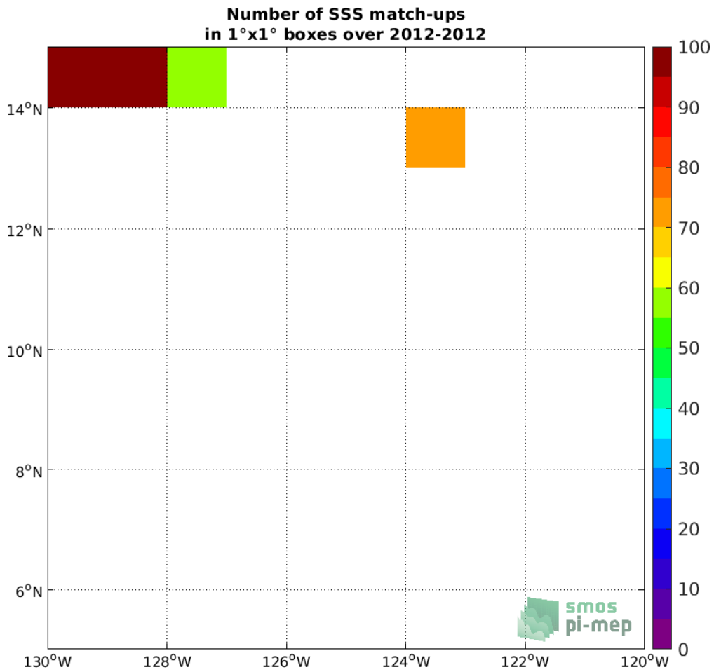
Figure 4: Number of SSS match-ups between TSG (GOSUD-Research-vessel) SSS and the Aquarius SSS L2 OR v5 (NASA-GSFC) SSS product for the SPURS 2 Pi-MEP region over 1°x1° boxes and for the full satellite product period.
