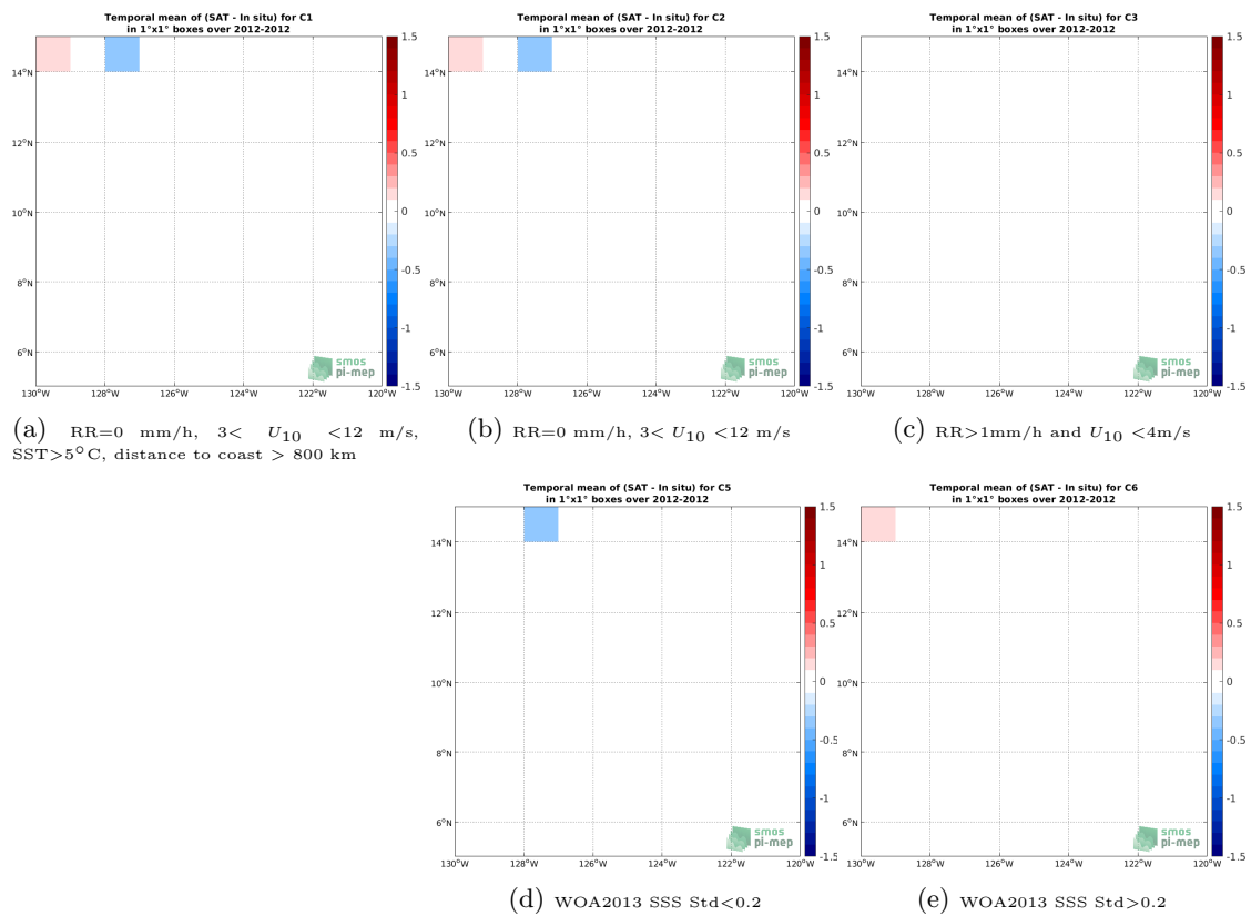
Figure 12: Temporal mean gridded over spatial boxes of size 1^\circ \times 1^\circ of \Delta\text{SSS} (Aquarius SSS L2 OR v5 (NASA-GSFC) - TSG (GOSUD-Research-vessel)) for 5 different subdatasets corresponding to:RR=0 mm/h, 3 < U_{10} < 12 m/s, SST>5°C, distance to coast > 800 km (a), RR=0 mm/h, 3 < U_{10} < 12 m/s (b), RR>1mm/h and U_{10} < 4 m/s (c), WOA2013 SSS Std<0.2 (d), WOA2013 SSS Std>0.2 (e).
