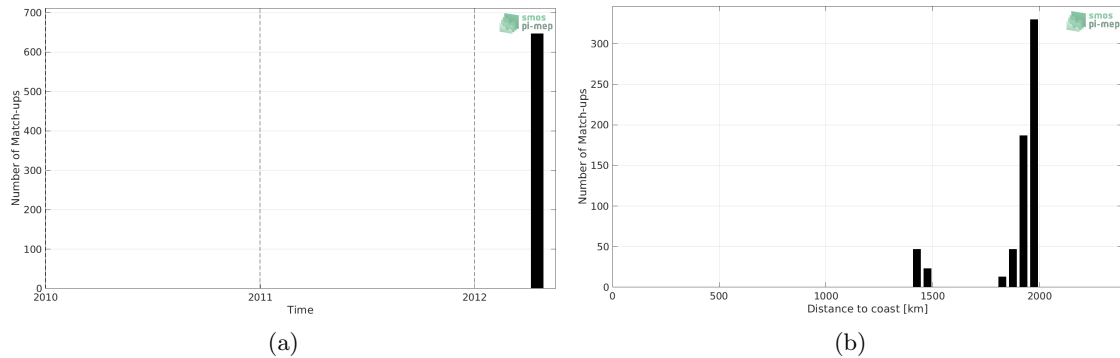
Figure 1: Number of match-ups between TSG (GOSUD-Research-vessel) and Aquarius SSS L2 OR v5 (NASA-GSFC) SSS as a function of time (a) and as function of the distance to coast (b) over the SPURS 2 Pi-MEP region and for the full satellite product period.
