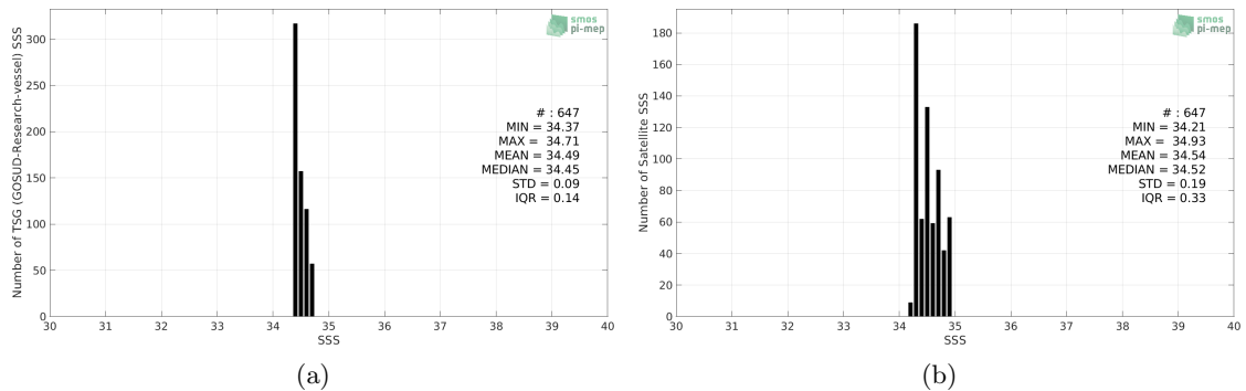
Figure 2: Histograms of SSS from TSG (GOSUD-Research-vessel) (a) and Aquarius SSS L2 OR v5 (NASA-GSFC) (b) considering all match-up pairs per bins of 0.1 over the SPURS 2 Pi-MEP region and for the full satellite product period.
