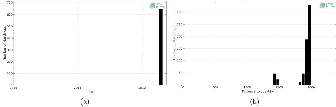
Figure 1: Number of match-ups between TSG-GOSUD-Research-vessel and Aquarius-L2-OR-V5 SSS as a function of time (a) and as function of the distance to coast (b) over the SPURS 2 Pi-MEP region and for the full satellite product period.
