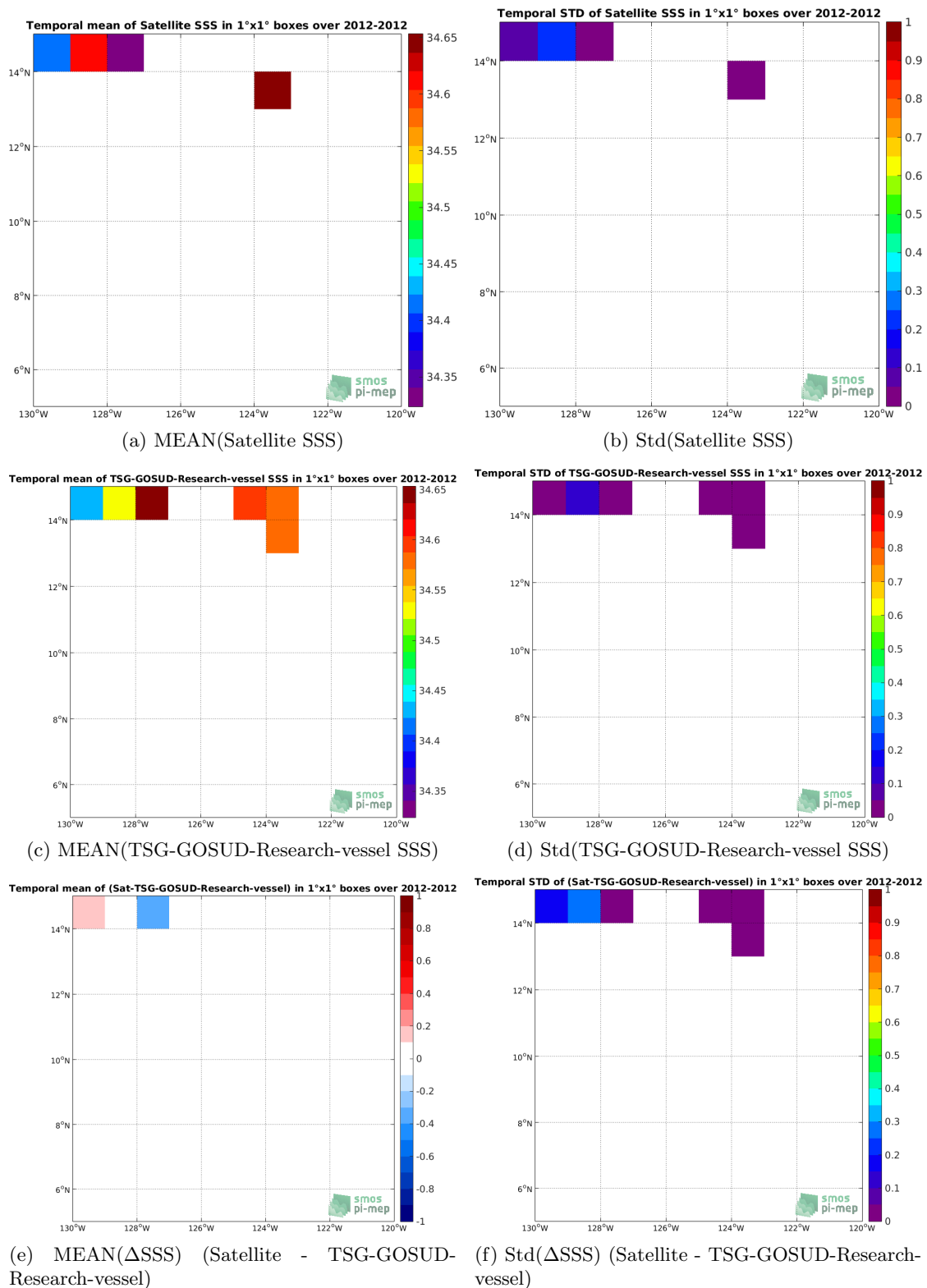
Figure 6: Temporal mean (left) and Std (right) of SSS from Aquarius-L2-OR-V5 (top), TSG-GOSUD-Research-vessel (middle), and of \Delta SSS (Satellite - TSG-GOSUD-Research-vessel). Only match-up pairs are used to generate these maps 22
