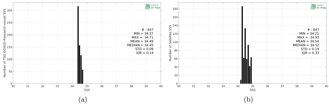
Figure 2: Histograms of SSS from TSG-GOSUD-Research-vessel (a) and Aquarius-L2-OR-V5 (b) considering all match-up pairs per bins of 0.1 over the SPURS 2 Pi-MEP region and for the full satellite product period.
