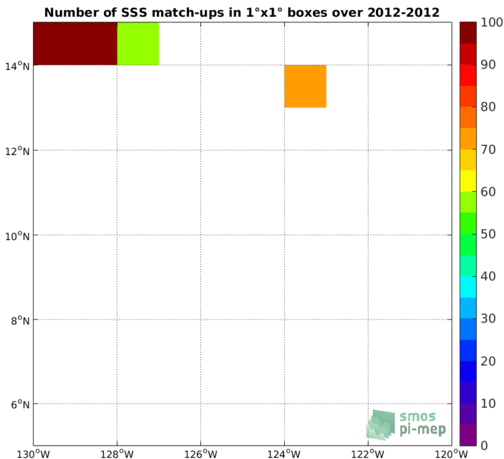
Figure 4: Number of SSS match-ups between TSG-GOSUD-Research-vessel SSS and the Aquarius-L2-OR-V5 SSS product for the SPURS 2 Pi-MEP region over 1°x1° boxes and for the full satellite product period.
