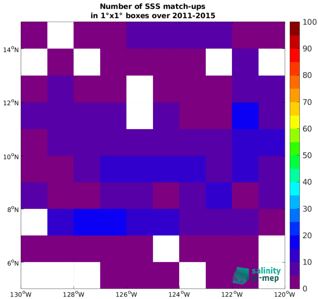
Figure 4: Number of SSS match-ups between Argo SSS and the Aquarius SSS L2 OR v5 (NASA-GSFC) SSS product for the SPURS 2 Pi-MEP region over 1°x1° boxes and for the full satellite product period.
