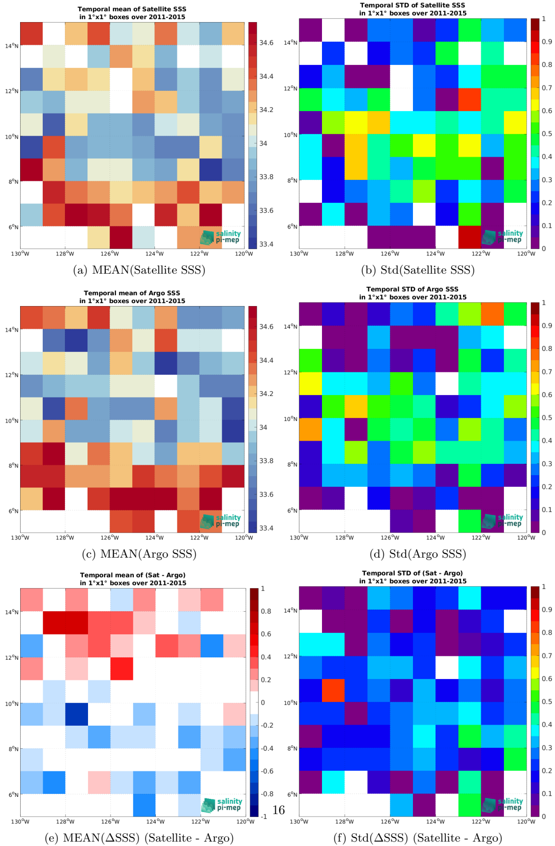
Figure 6: Temporal mean (left) and Std (right) of SSS from Aquarius SSS L2 OR v5 (NASA-GSFC) (top), Argo (middle), and of \Delta SSS (Satellite - Argo). Only match-up pairs are used to generate these maps.
