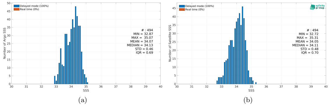
Figure 2: Histograms of SSS from Argo (a) and Aquarius SSS L2 OR v5 (NASA-GSFC) (b) considering all match-up pairs per bins of 0.1 over the SPURS 2 Pi-MEP region and for the full satellite product period.
