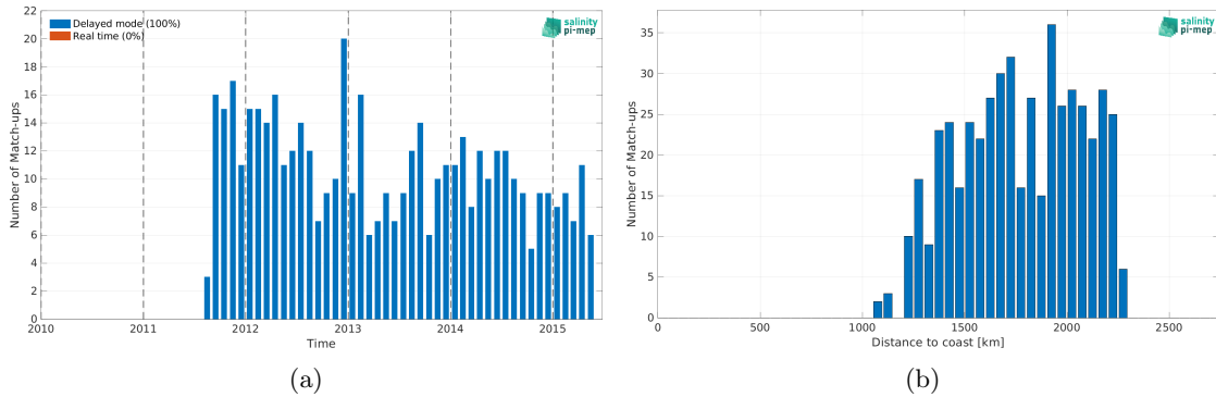
Figure 1: Number of match-ups between Argo and Aquarius SSS L2 OR v5 (NASA-GSFC) SSS as a function of time (a) and as function of the distance to coast (b) over the SPURS 2 Pi-MEP region and for the full satellite product period.
