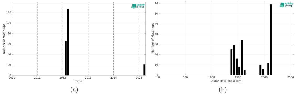
Figure 2: Number of match-ups between TSG (SAMOS) and Aquarius SSS L2 CAP v5 (JPL) SSS as a function of time (a) and as function of the distance to coast (b) over the SPURS 2 Pi-MEP region and for the full satellite product period.
