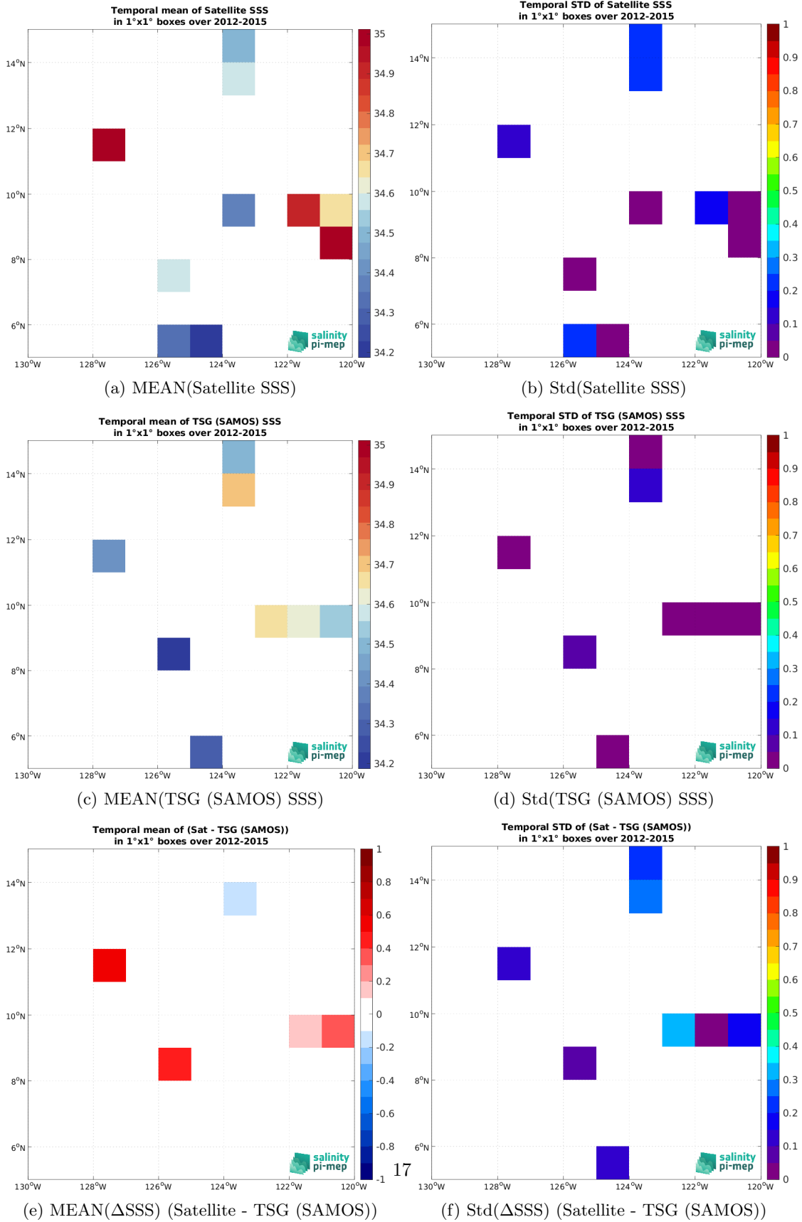
Figure 7: Temporal mean (left) and Std (right) of SSS from Aquarius SSS L2 CAP v5 (JPL) (top), TSG (SAMOS) (middle), and of \Delta SSS (Satellite - TSG (SAMOS)). Only match-up pairs are used to generate these maps.
