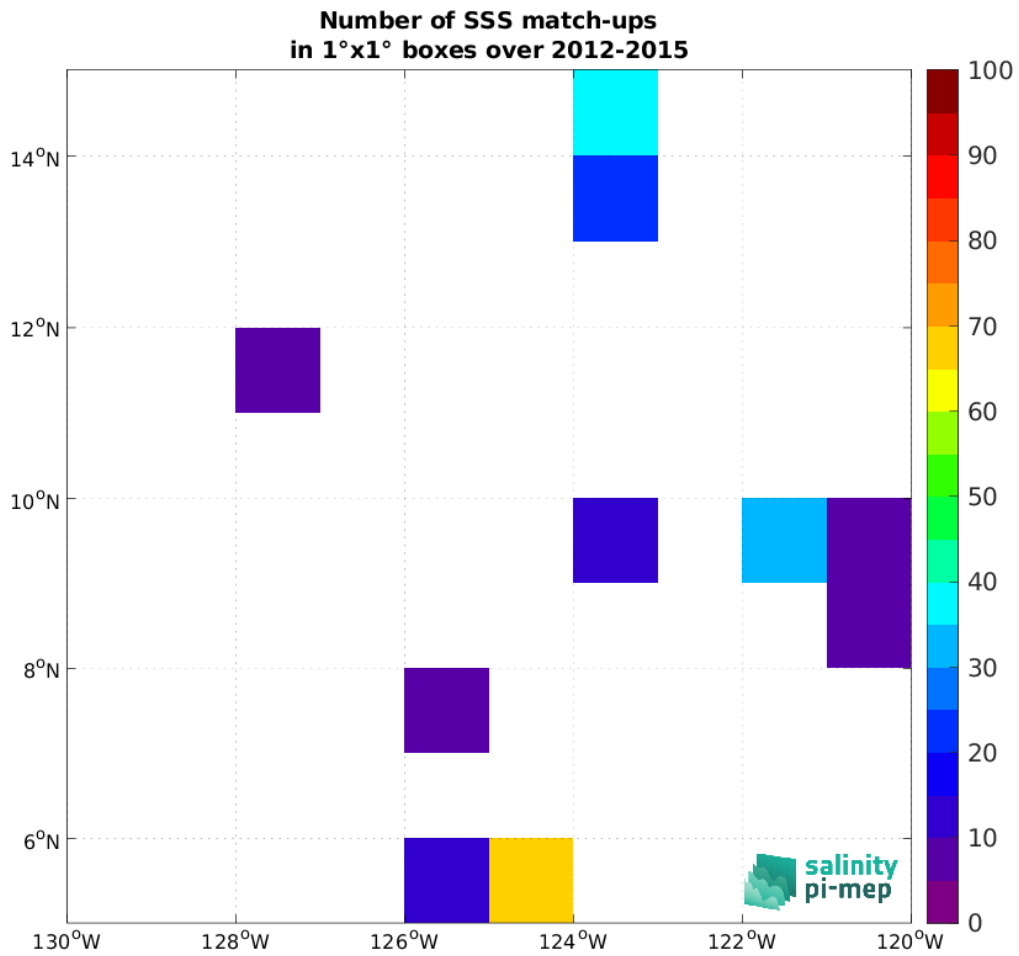
Figure 5: Number of SSS match-ups between TSG (SAMOS) SSS and the Aquarius SSS L2 CAP v5 (JPL) SSS product for the SPURS 2 Pi-MEP region over 1°x1° boxes and for the full satellite product period.
