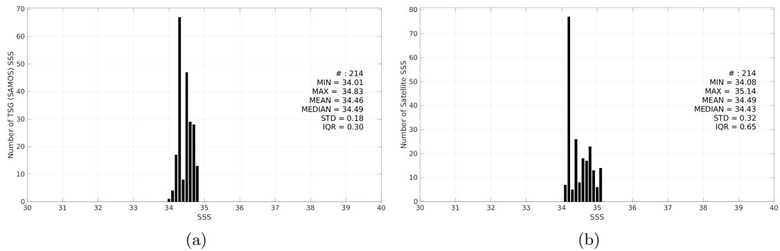
Figure 3: Histograms of SSS from TSG (SAMOS) (a) and Aquarius SSS L2 CAP v5 (JPL) (b) considering all match-up pairs per bins of 0.1 over the SPURS 2 Pi-MEP region and for the full satellite product period.
