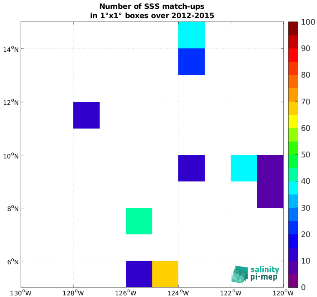
Figure 4: Number of SSS match-ups between TSG (SAMOS) SSS and the Aquarius SSS L2 CAP v5 (JPL) SSS product for the SPURS 2 Pi-MEP region over 1°x1° boxes and for the full satellite product period.
