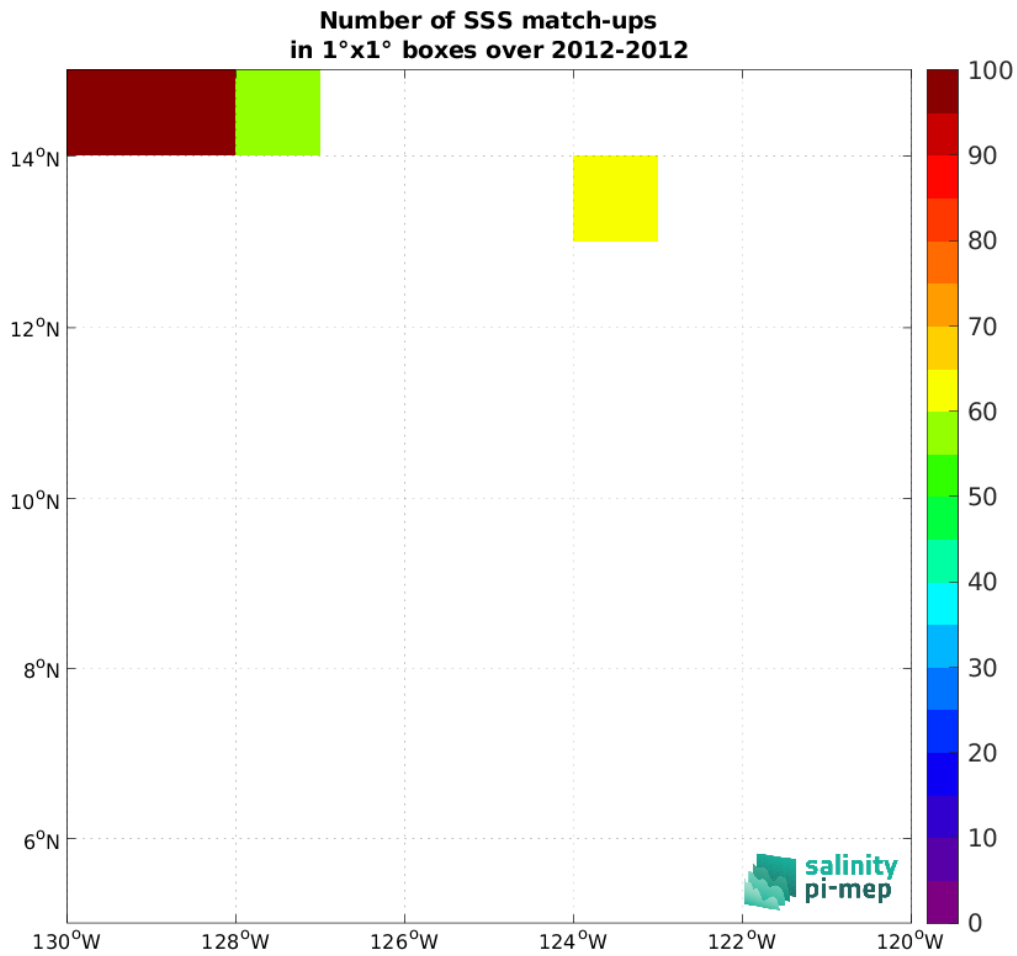
Figure 5: Number of SSS match-ups between TSG (GOSUD-Research-vessel) SSS and the Aquarius SSS L2 CAP v5 (JPL) SSS product for the SPURS 2 Pi-MEP region over 1°x1° boxes and for the full satellite product period.
