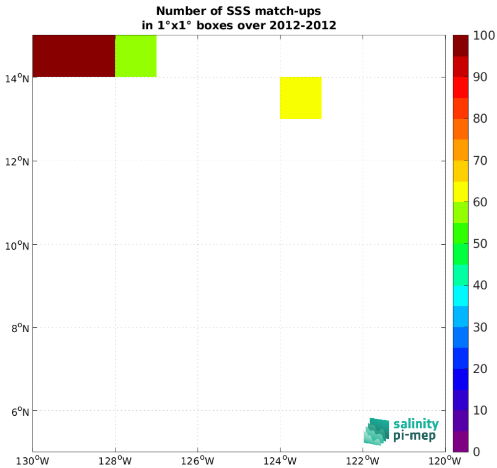
Figure 5: Number of SSS match-ups between TSG (GOSUD-Research-vessel) SSS and the Aquarius SSS L2 CAP v5 (JPL) SSS product for the SPURS 2 Pi-MEP region over 1°×1° boxes and for the full satellite product period.
