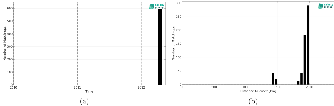
Figure 2: Number of match-ups between TSG (GOSUD-Research-vessel) and Aquarius SSS L2 CAP v5 (JPL) SSS as a function of time (a) and as function of the distance to coast (b) over the SPURS 2 Pi-MEP region and for the full satellite product period.
