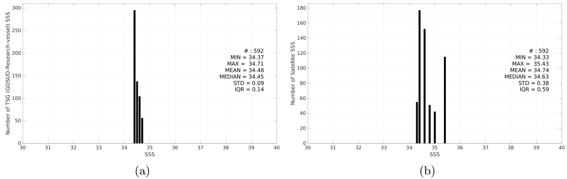
Figure 3: Histograms of SSS from TSG (GOSUD-Research-vessel) (a) and Aquarius SSS L2 CAP v5 (JPL) (b) considering all match-up pairs per bins of 0.1 over the SPURS 2 Pi-MEP region and for the full satellite product period.
