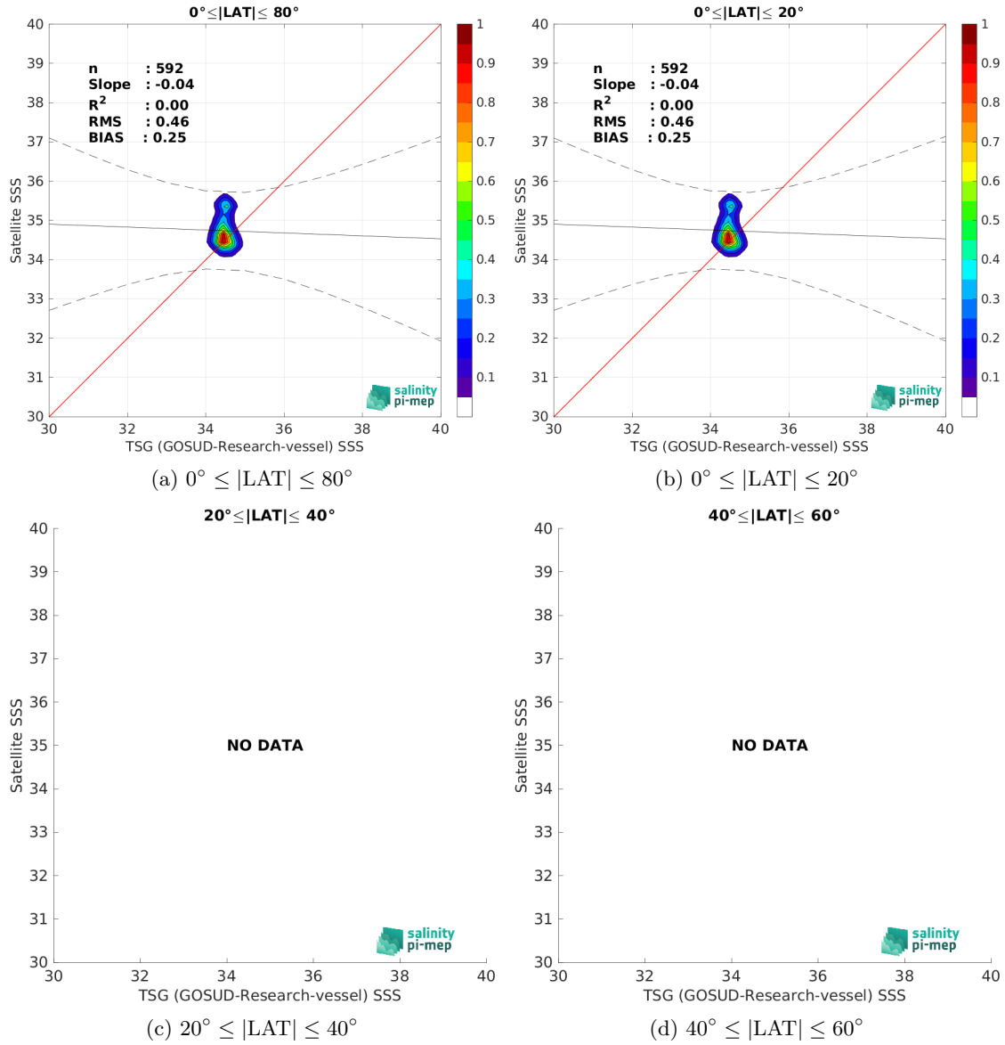
Figure 10: Contour maps of the concentration of Aquarius SSS L2 CAP v5 (JPL) SSS (y-axis) versus TSG (GOSUD-Research-vessel) SSS (x-axis) at match-up pairs for different latitude bands. For each plot, the red line shows x=y . The black thin and dashed lines indicate a linear fit through the data cloud and the \pm 95\% confidence levels, respectively. The number match-up pairs n , the slope and R^2 coefficient of the linear fit, the root mean square (RMS) and the mean bias between satellite and in situ data are indicated for each latitude band in each plots.
