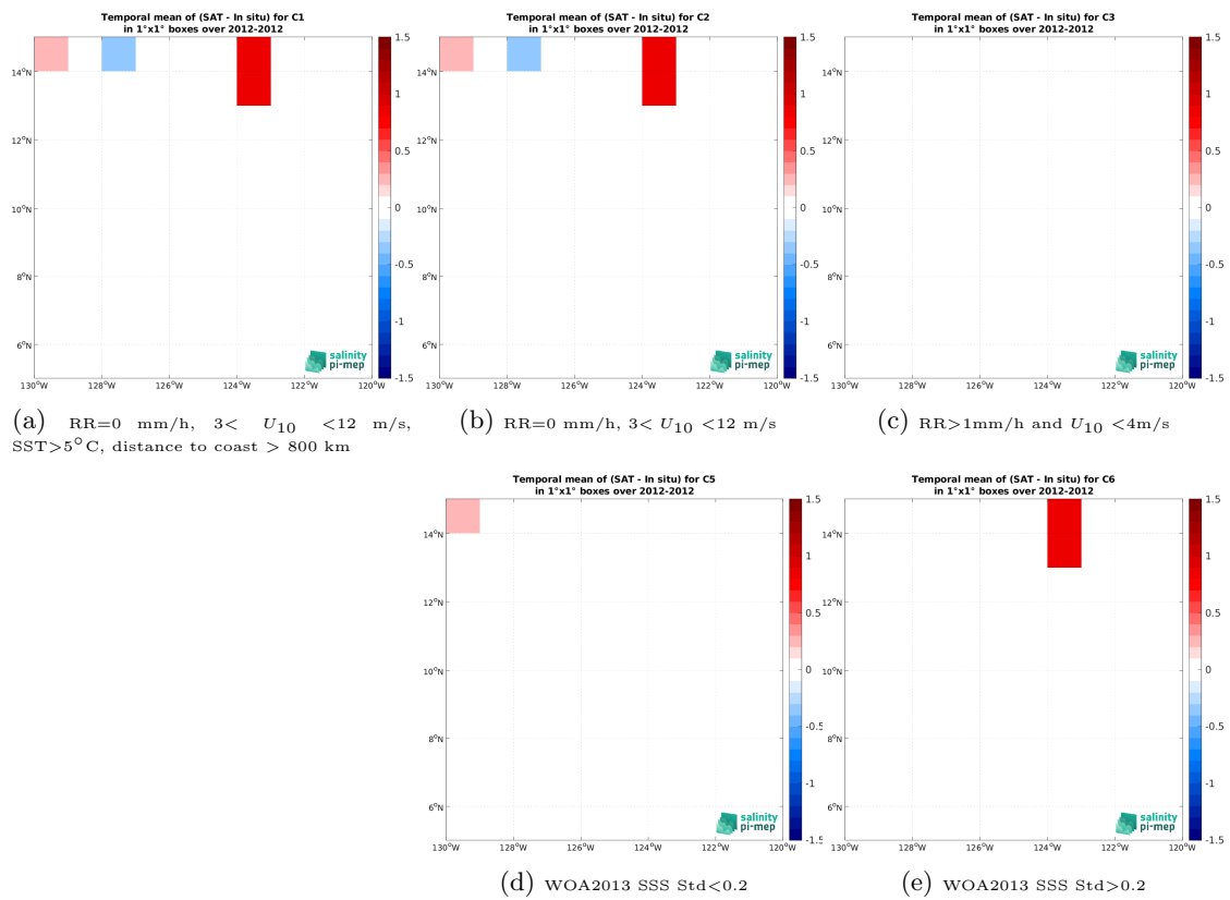
Figure 14: Temporal mean gridded over spatial boxes of size 1^\circ \times 1^\circ of \Delta SSS (Aquarius SSS L2 CAP v5 (JPL) - TSG (GOSUD-Research-vessel)) for 5 different subdatasets corresponding to:RR=0 mm/h, 3 < U_{10} < 12 m/s, SST>5°C, distance to coast > 800 km (a), RR=0 mm/h, 3 < U_{10} < 12 m/s (b), RR>1mm/h and U_{10} < 4 m/s (c), WOA2013 SSS Std<0.2 (d), WOA2013 SSS Std>0.2 (e).
