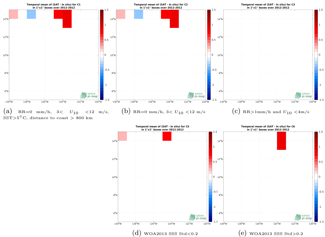
Figure 12: Temporal mean gridded over spatial boxes of size 1^\circ \times 1^\circ of \Delta\text{SSS} (Aquarius SSS L2 CAP v5 (JPL) - TSG (GOSUD-Research-vessel)) for 5 different subdatasets corresponding to:RR=0 mm/h, 3 < U_{10} < 12 m/s, SST >5^\circ\text{C} , distance to coast > 800 km (a), RR=0 mm/h, 3 < U_{10} < 12 m/s (b), RR >1 mm/h and U_{10} < 4 m/s (c), WOA2013 SSS Std <0.2 (d), WOA2013 SSS Std >0.2 (e).
