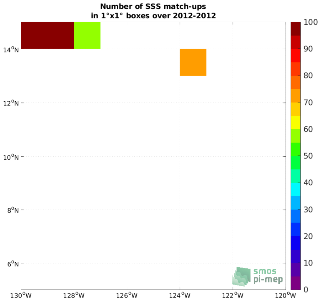
Figure 4: Number of SSS match-ups between TSG (GOSUD-Research-vessel) SSS and the Aquarius SSS L2 CAP v5 (JPL) SSS product for the SPURS 2 Pi-MEP region over 1°x1° boxes and for the full satellite product period.
