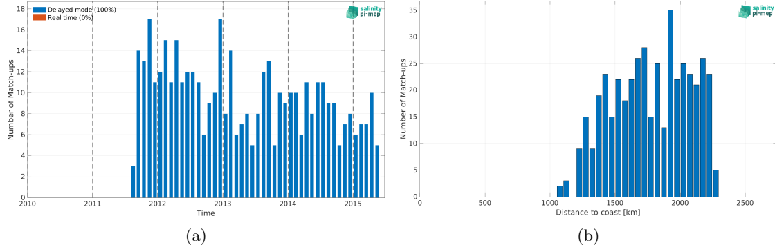
Figure 2: Number of match-ups between Argo and Aquarius SSS L2 CAP v5 (JPL) SSS as a function of time (a) and as function of the distance to coast (b) over the SPURS 2 Pi-MEP region and for the full satellite product period.
