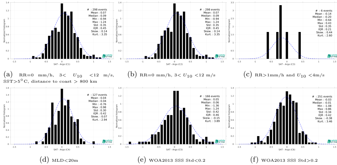
Figure 15: Normalized histogram of \Delta\text{SSS} (Aquarius SSS L2 CAP v5 (JPL) - Argo) for 6 different subdatasets corresponding to: RR=0 mm/h, 3 < U_{10} < 12 m/s, SST>5°C, distance to coast > 800 km (a), RR=0 mm/h, 3 < U_{10} < 12 m/s (b), RR>1mm/h and U_{10} < 4 m/s (c), MLD<20m (d), WOA2013 SSS Std<0.2 (e), WOA2013 SSS Std>0.2 (f).
