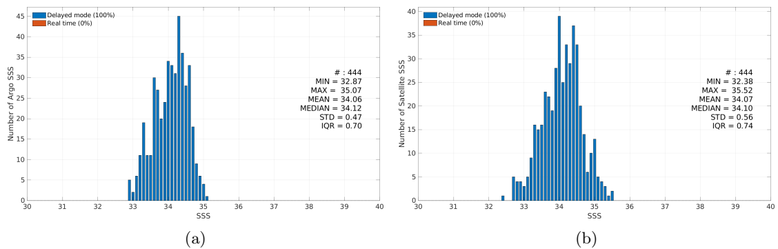
Figure 3: Histograms of SSS from Argo (a) and Aquarius SSS L2 CAP v5 (JPL) (b) considering all match-up pairs per bins of 0.1 over the SPURS 2 Pi-MEP region and for the full satellite product period.
