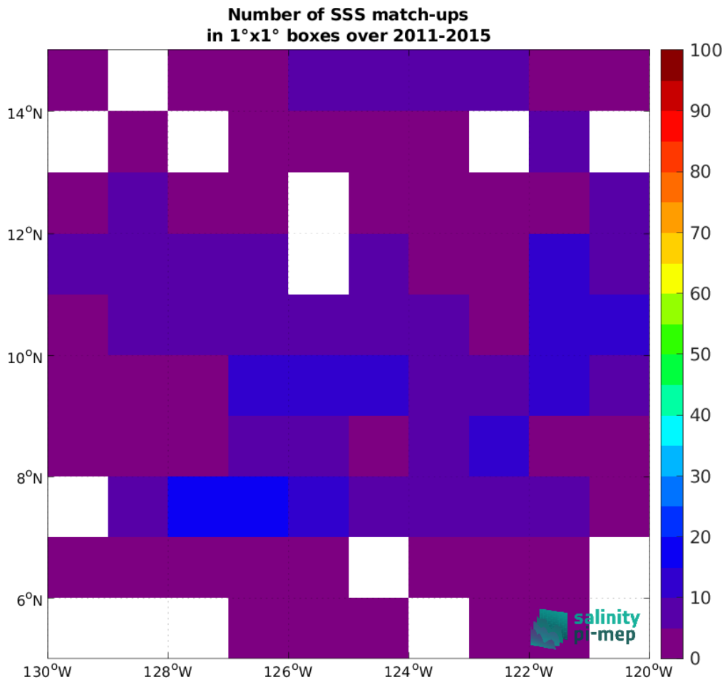
Figure 5: Number of SSS match-ups between Argo SSS and the Aquarius SSS L2 CAP v5 (JPL) SSS product for the SPURS 2 Pi-MEP region over 1°x1° boxes and for the full satellite product period.
