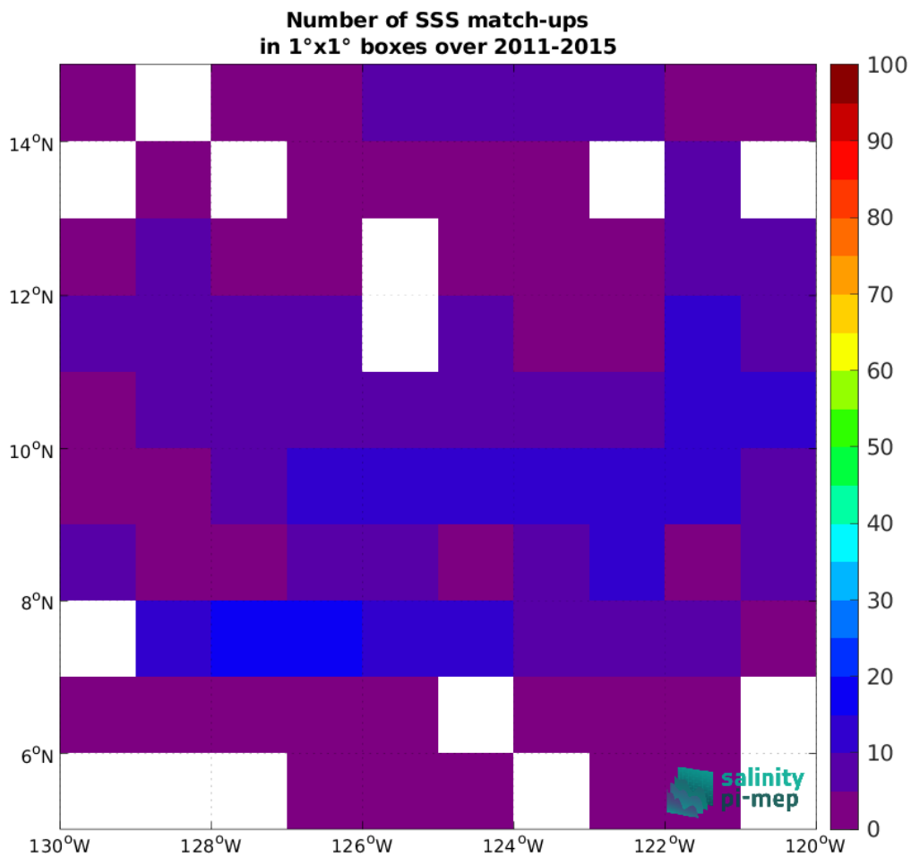
Figure 4: Number of SSS match-ups between Argo SSS and the Aquarius SSS L2 CAP v5 (JPL) SSS product for the SPURS 2 Pi-MEP region over 1°x1° boxes and for the full satellite product period.
