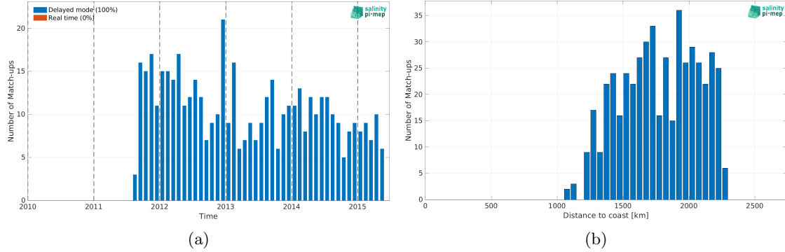
Figure 1: Number of match-ups between Argo and Aquarius SSS L2 CAP v5 (JPL) SSS as a function of time (a) and as function of the distance to coast (b) over the SPURS 2 Pi-MEP region and for the full satellite product period.
