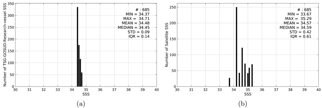
Figure 2: Histograms of SSS from TSG-GOSUD-Research-vessel (a) and AQUARIUS-L2-JPL-V4 (b) considering all match-up pairs per bins of 0.1 over the SPURS 2 Pi-MEP region and for the full satellite product period.
