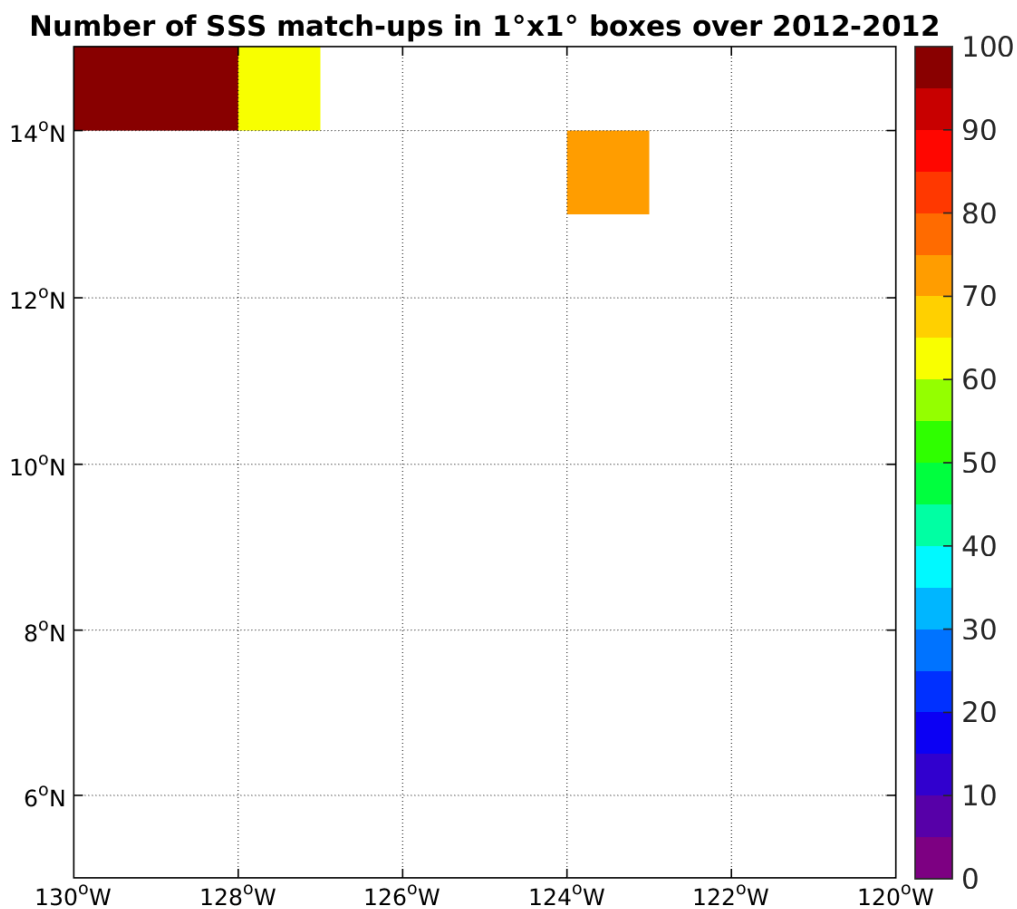
Figure 4: Number of SSS match-ups between TSG-GOSUD-Research-vessel SSS and the AQUARIUS-L2-JPL-V4 SSS product for the SPURS 2 Pi-MEP region over 1°x1° boxes and for the full satellite product period.
