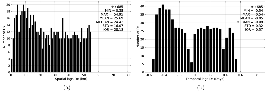
Figure 5: Histograms of the spatial (a) and temporal (b) lags between the time of the TSG-GOSUD-Research-vessel measurements and the date of the corresponding AQUARIUS-L2-JPL-V4 SSS product.
