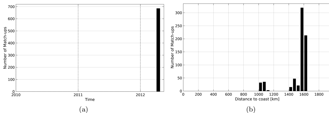
Figure 1: Number of match-ups between TSG-GOSUD-Research-vessel and AQUARIUS-L2-JPL-V4 SSS as a function of time (a) and as function of the distance to coast (b) over the SPURS 2 Pi-MEP region and for the full satellite product period.
