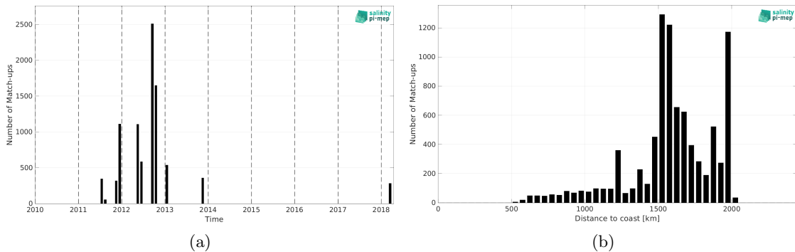
Figure 1: Number of match-ups between TSG (SAMOS) and SMOS and SMAP SSS L4 OI v1 - 7 Days (LOPS) SSS as a function of time (a) and as function of the distance to coast (b) over the SPURS 1 Pi-MEP region and for the full satellite product period.
