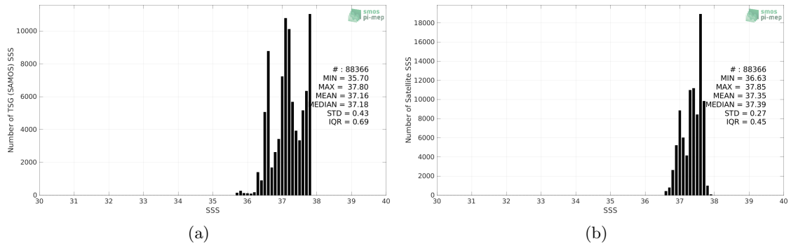
Figure 2: Histograms of SSS from TSG (SAMOS) (a) and SMOS and SMAP SSS L4 OI v1 - 7 Days (LOPS) (b) considering all match-up pairs per bins of 0.1 over the SPURS 1 Pi-MEP region and for the full satellite product period.
