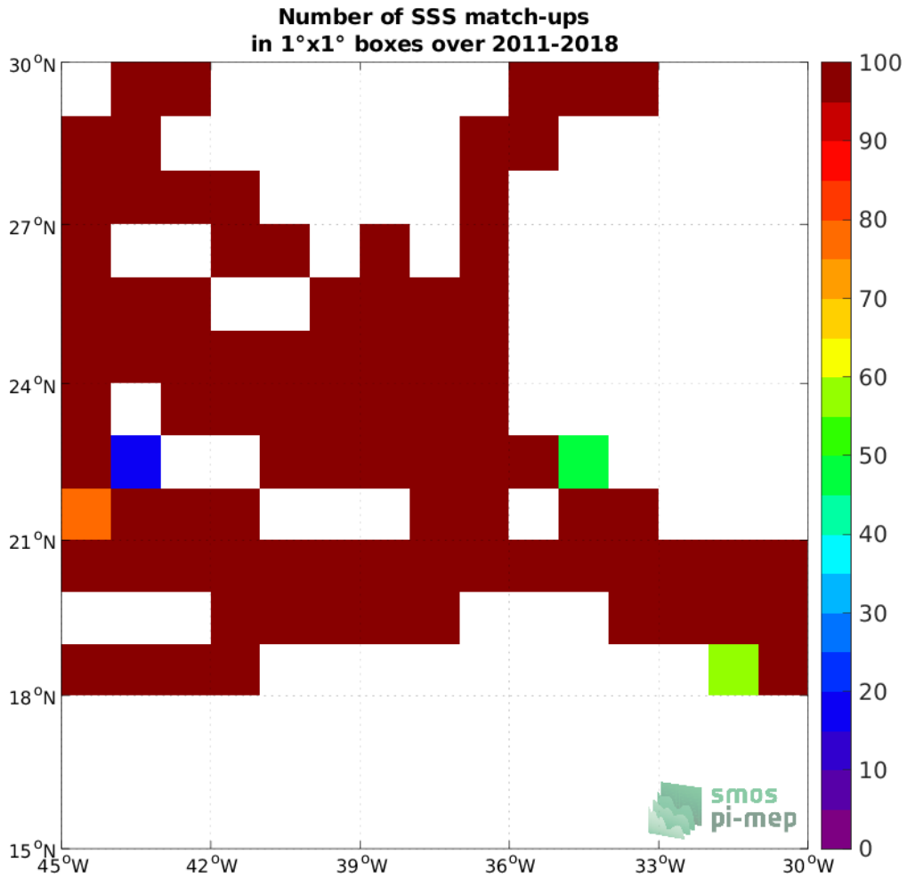
Figure 4: Number of SSS match-ups between TSG (SAMOS) SSS and the SMOS and SMAP SSS L4 OI v1 - 7 Days (LOPS) SSS product for the SPURS 1 Pi-MEP region over 1°x1° boxes and for the full satellite product period.
