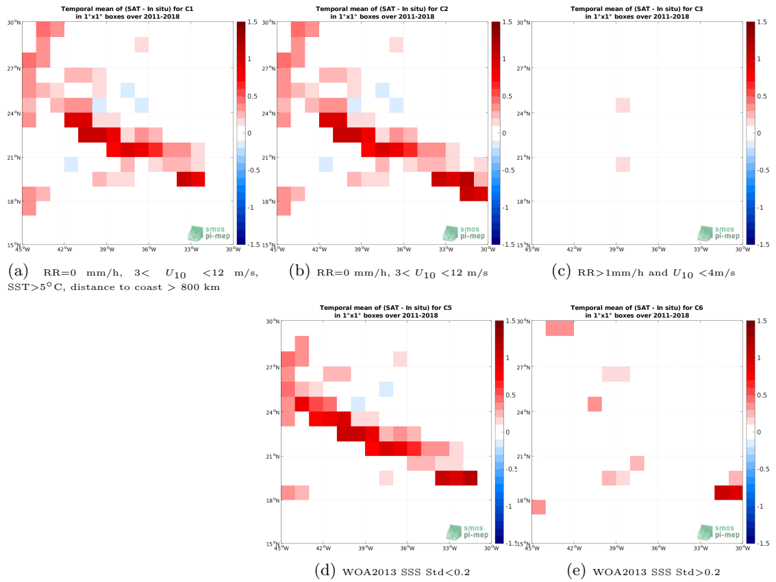
Figure 12: Temporal mean gridded over spatial boxes of size 1^\circ \times 1^\circ of \Delta SSS (SMOS and SMAP SSS L4 OI v1 - 7 Days (LOPS) - TSG (SAMOS)) for 5 different subdatasets corresponding to:RR=0 mm/h, 3 < U_{10} < 12 m/s, SST >5^\circ C, distance to coast > 800 km (a), RR=0 mm/h, 3 < U_{10} < 12 m/s (b), RR >1 mm/h and U_{10} < 4 m/s (c), WOA2013 SSS Std <0.2 (d), WOA2013 SSS Std >0.2 (e).
