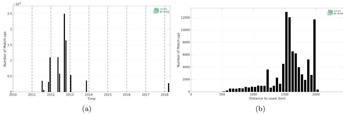
Figure 1: Number of match-ups between TSG (SAMOS) and SMOS and SMAP SSS L4 OI v1 - 7 Days (LOPS) SSS as a function of time (a) and as function of the distance to coast (b) over the SPURS 1 Pi-MEP region and for the full satellite product period.
