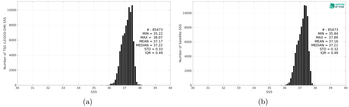
Figure 2: Histograms of SSS from TSG (LEGOS-DM) (a) and SMOS and SMAP SSS L4 OI v1 - 7 Days (LOPS) (b) considering all match-up pairs per bins of 0.1 over the SPURS 1 Pi-MEP region and for the full satellite product period.
