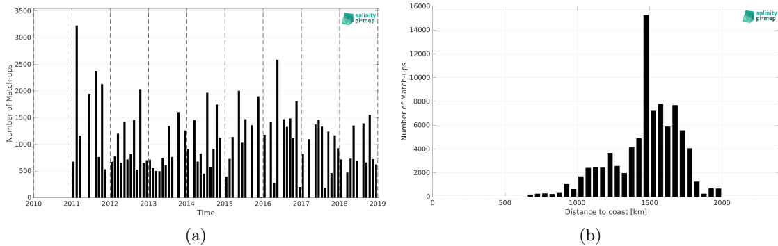
Figure 1: Number of match-ups between TSG (LEGOS-DM) and SMOS and SMAP SSS L4 OI v1 - 7 Days (LOPS) SSS as a function of time (a) and as function of the distance to coast (b) over the SPURS 1 Pi-MEP region and for the full satellite product period.
