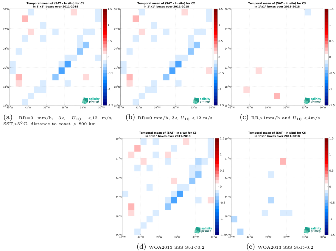
Figure 12: Temporal mean gridded over spatial boxes of size 1^{\circ}\times 1^{\circ} of \Delta\text{SSS} (SMOS and SMAP SSS L4 OI v1 - 7 Days (LOPS) - TSG (LEGOS-DM)) for 5 different subdatasets corresponding to:RR=0 mm/h, 3 < U_{10} < 12 m/s, SST >5^{\circ}\text{C} , distance to coast > 800 km (a), RR=0 mm/h, 3 < U_{10} < 12 m/s (b), RR >1 mm/h and U_{10} < 4 m/s (c), WOA2013 SSS Std <0.2 (d), WOA2013 SSS Std >0.2 (e).
